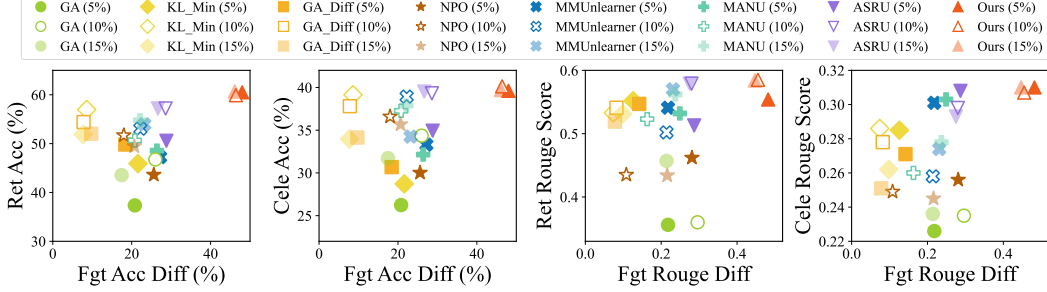
Figure 4: Forgetting-utility trade-off on MLLMU-Bench using LLaVA-1.5-7B under 5%, 10%, and 15% forgetting ratios. The two plots on the left present classification results, with the x -axis measuring the drop in forget-set accuracy (Fgt Acc Diff), whereas the two panels on the right present generation results, with the x -axis measuring the decrease in forget-set ROUGE score (Fgt Rouge Diff). The y -axis reports model utility on the retained (Ret) and celebrity (Cele) sets.
