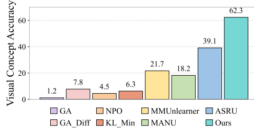
(b) Visual concept accuracy results.
