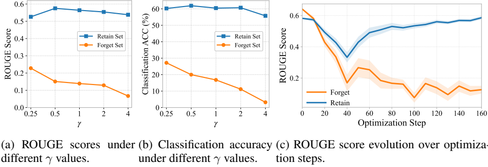
Figure 5: Parameter sensitivity and optimization dynamics on MLLMU-Bench with LLaVA-1.5-7B. (5a) and (5b) show the impact of \gamma on ROUGE score and classification accuracy, while (5c) presents ROUGE score evolution across optimization steps.
