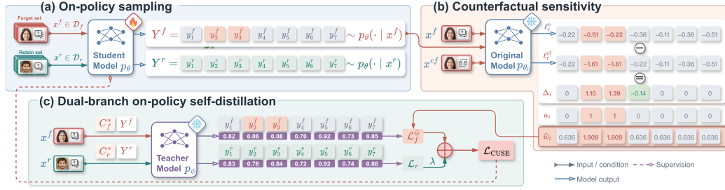
Figure 2: CUSE consists of (a) on-policy sampling, (b) counterfactual sensitivity estimation, and (c) dual-branch on-policy self-distillation with sensitivity-aware forgetting supervision.
