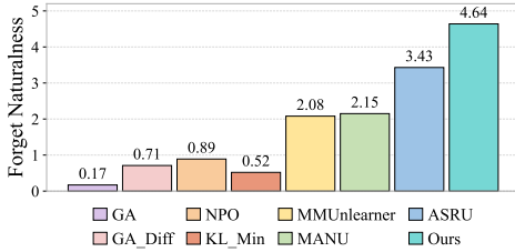
(a) Forget naturalness results.
