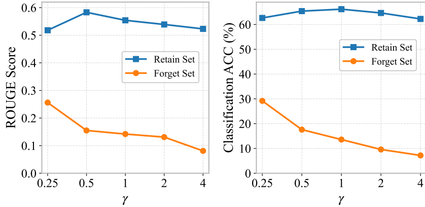
(a) ROUGE scores under different \gamma values. (b) Classification accuracy under different \gamma values.
