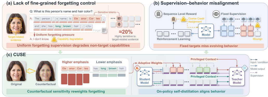
Figure 1: Motivation of CUSE and its key components for addressing fine-grained forgetting control and supervision-behavior misalignment in MLLM unlearning.
