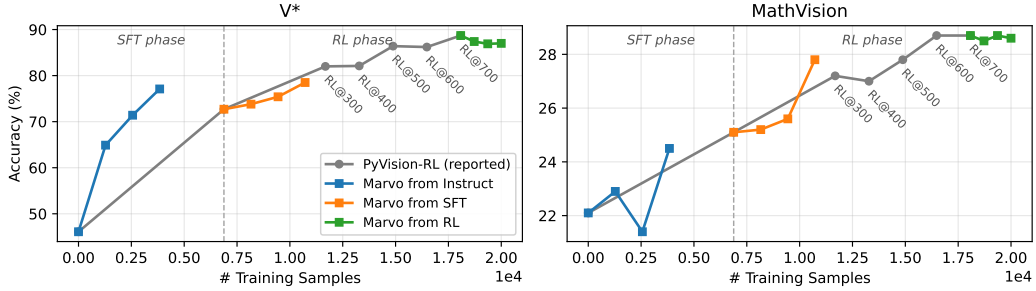
Figure 5: Marvo across post-training stages. The gray curve is the reported PyVision-RL training progress. Colored curves are Marvo experiments launched from different checkpoints.
