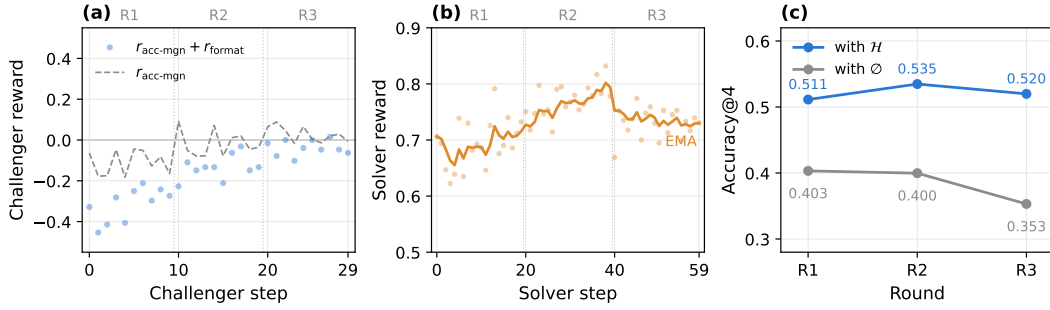
Figure 4: Training Dynamics. (a-b) Reward progress in challenger and solver training phase. (c) Per-round difficulty of challenger-generated datasets, as measured by model at each round.
