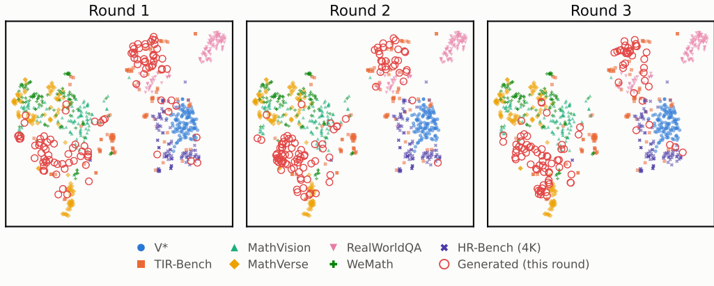
Figure 10: Image-embedding space of generated questions vs. evaluation benchmarks across training rounds. Each panel shows a shared 2D projection (PCA + t-SNE over Qwen3-VL-4B vision-tower embeddings) of 100 images sampled from each of seven evaluation benchmarks (colored points) and 100 images underlying the questions generated in the indicated training round (red rings).
