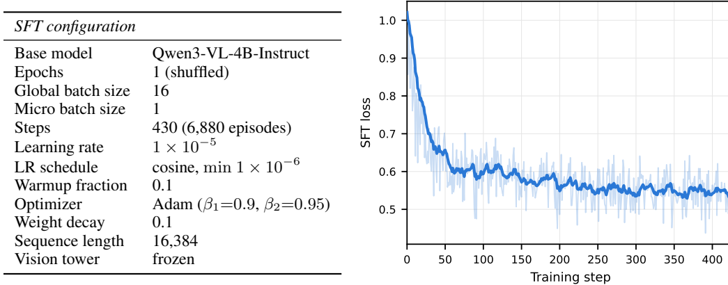
Figure 8: Left: SFT hyperparameters. Right: SFT training loss.
