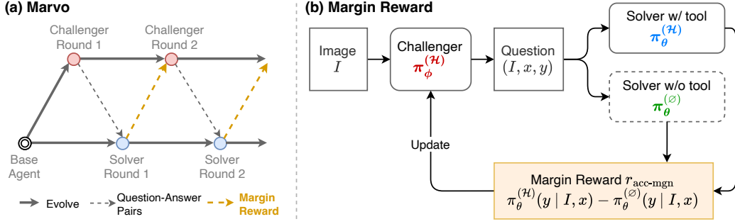
Figure 1: Flowchart of Marvo. (a) Marvo employs an evolution loop between a challenger and a solver, driven by the Margin Reward. (b) The Margin Reward quantifies the solver’s performance gap with and without tools, encouraging the challenger to propose questions that require tool use.
