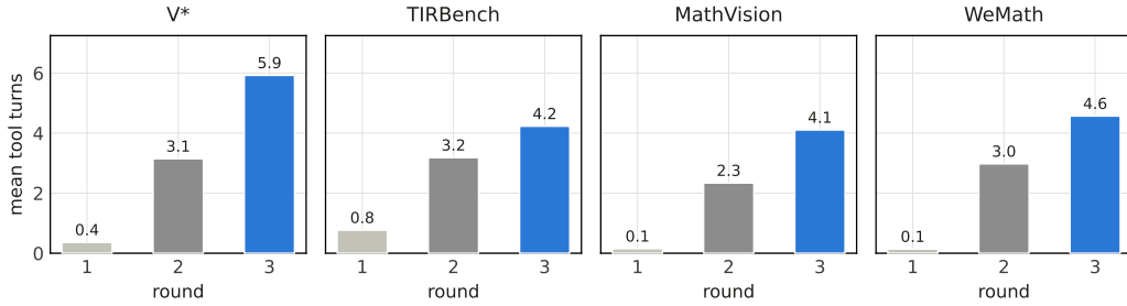
Figure 6: Mean number of tool turns during evaluation. Initializing from Instruct model, Marvo incentivizes tool invocation without human-curated data supervision.
