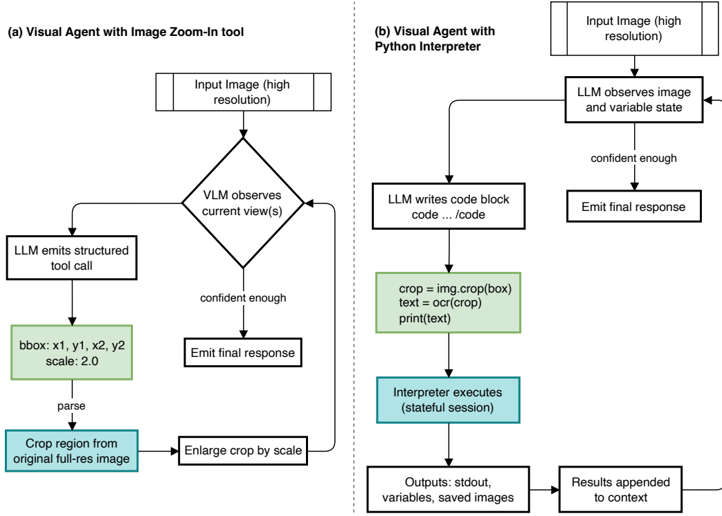
Figure 7: Visual Agent Flowcharts
