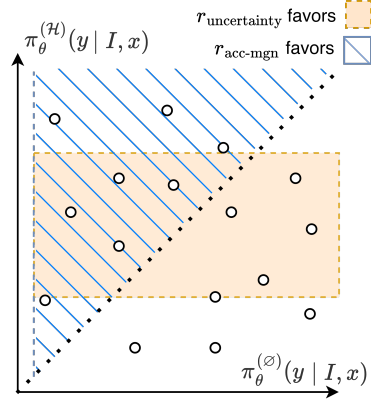
Figure 2: Question Distribution.
