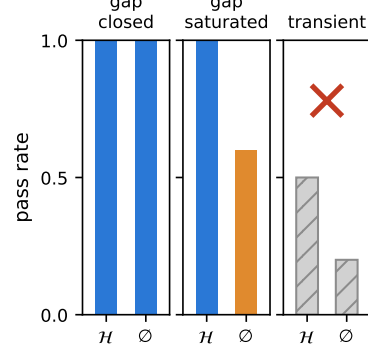
Figure 3: Equilibrium States.
