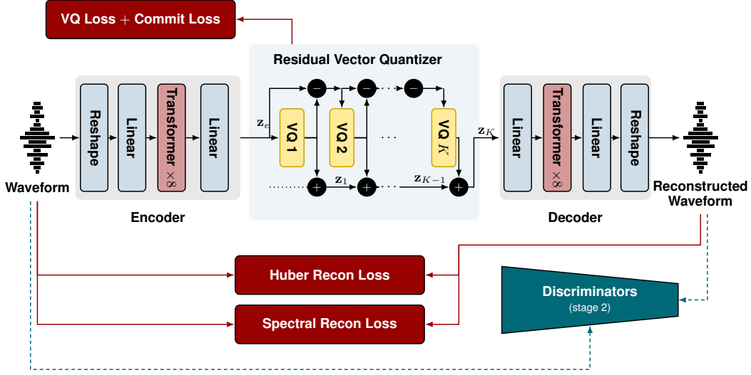
Figure 1: MYOCODEC architecture. A causal Transformer encoder–decoder with residual vector quantization (RVQ) processes each EMG channel independently at 50 Hz. The discriminators are used only during the second phase of training.
