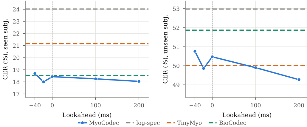
Figure 3: Effect of lookahead on emg2qwerty . Decoding performance improves at a negative lookahead of -20 ms, decreases slightly at zero lookahead, and then gradually improves with increasing positive lookahead.
