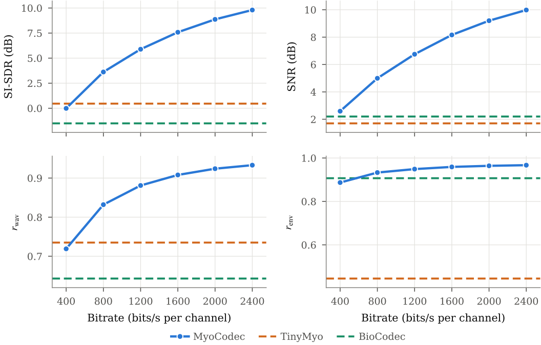
Figure 5: Reconstruction quality across various bitrates. MYOCODEC outperforms TinyMyo and BioCodec on reconstruction quality using only two codebooks.
