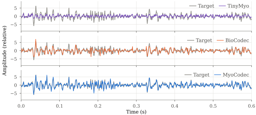
Figure 2: An example of EMG signals reconstructed by each model: TinyMyo (top), BioCodec (middle), and MYOCODEC (bottom). MYOCODEC shows the best reconstruction quality, more properly capturing signal peaks missed by the other models.
