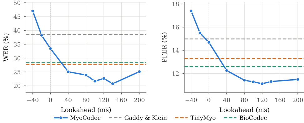
Figure 4: emg2speech with different lookahead. The best performance is achieved when lookahead between 100 ms–140 ms is applied.
