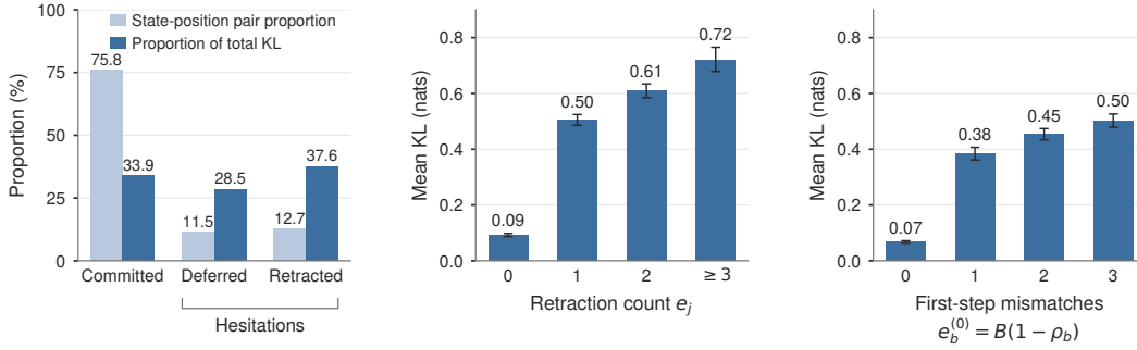
Figure 1: Hesitation pilot study on the rollouts of the base SDAR-4B student under dynamic decoding, with TraDo-8B-Instruct as the teacher. Left: share of all supervisable state–position pairs (light blue) and share of the total teacher–student reverse KL (dark blue) in each commitment category. Middle: mean per-position KL, averaged over each position’s recorded steps and grouped by the retraction count e_j , i.e., the number of uncommitted proposals at position j that differ from its final token. Right: mean per-block KL, averaged over masked positions within each step and then over steps, grouped by the first-step mismatch count e_b^{(0)} , i.e., the number of positions in block b whose first proposal differs from the final token; only complete four-position blocks are included. Error bars in the middle and right panels are 95% confidence intervals.
