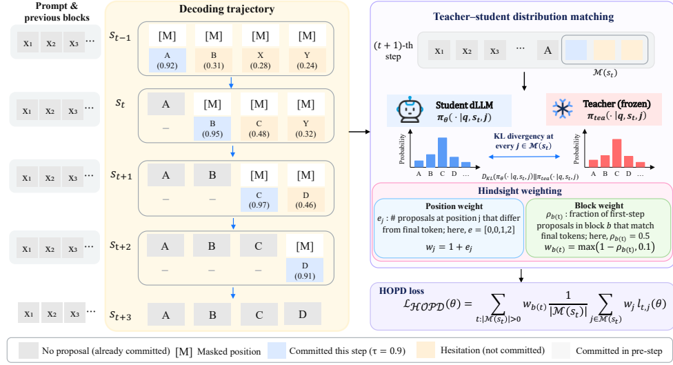
Figure 2: Overview of HOPD. Left: Dynamic decoding of a four-token block ( \tau = 0.9 ). Blue proposals are committed, while yellow proposals are hesitations whose positions remain masked. Right: At each visited pre-action state, the student matches the frozen teacher’s distributions at all masked positions, including hesitations. Position and block weights are computed from the completed trajectory’s retraction counts and first-step retention, respectively.
