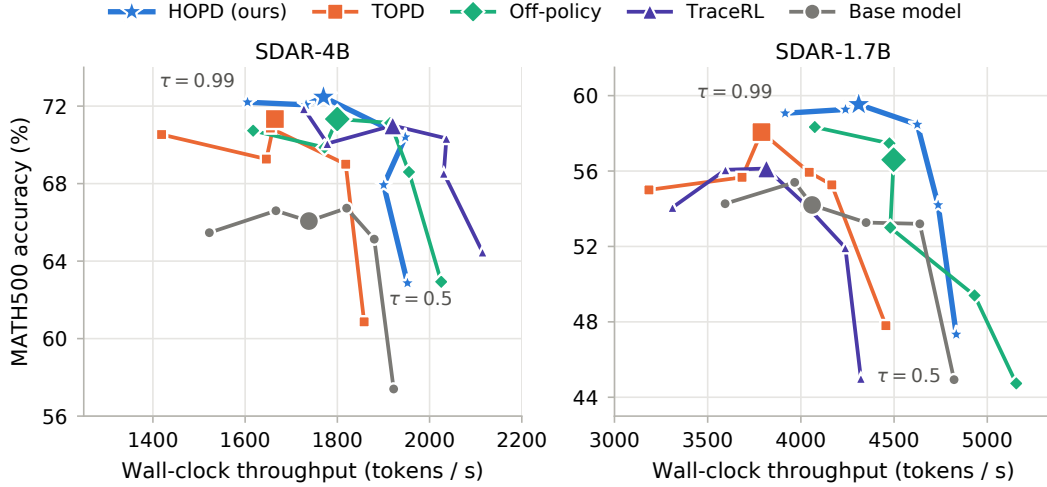
Figure 4: Accuracy against wall-clock generation throughput on MATH500 (dynamic decoding), for the threshold sweep of Figure 3. Left: SDAR-4B. Right: SDAR-1.7B.
