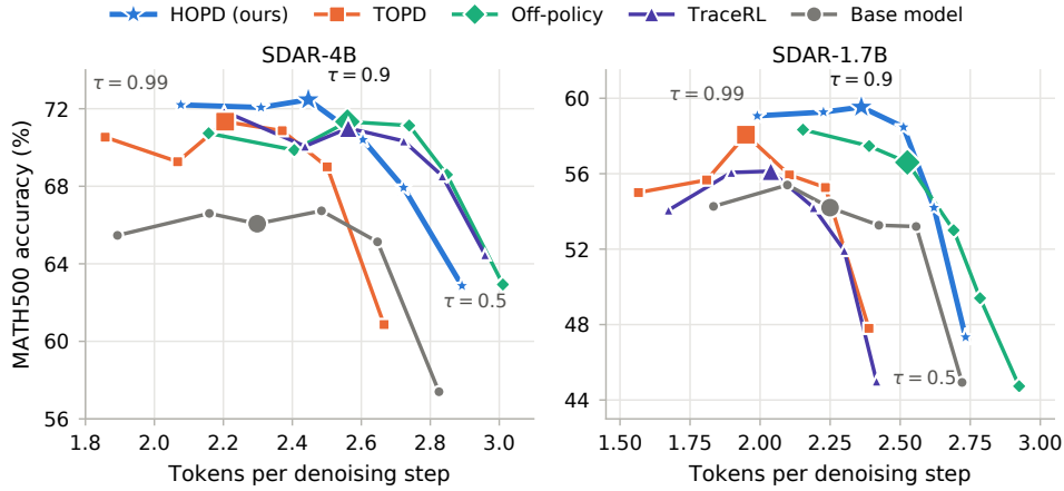
Figure 3: Accuracy against committed tokens per denoising step on MATH500 (dynamic decoding) as the commit threshold \tau goes from 0.5 to 0.99, right to left along each curve; large markers denote the training threshold \tau = 0.9 . Left: SDAR-4B. Right: SDAR-1.7B.
