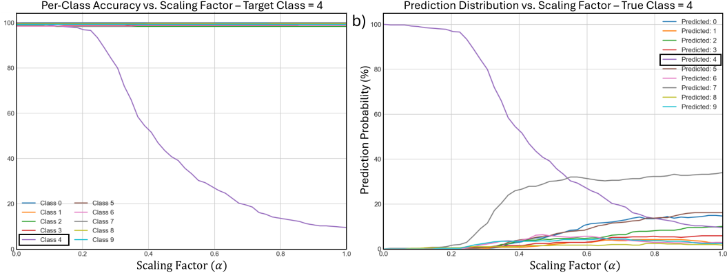
Figure 13: Suppression sensitivity for a single class (Class 4, "Church") in the ViT model. (a) Per-class accuracy as a function of the scaling factor \alpha . (b) Distribution of predictions for images of the target class, showing how confidence is reallocated as the feature is suppressed.
