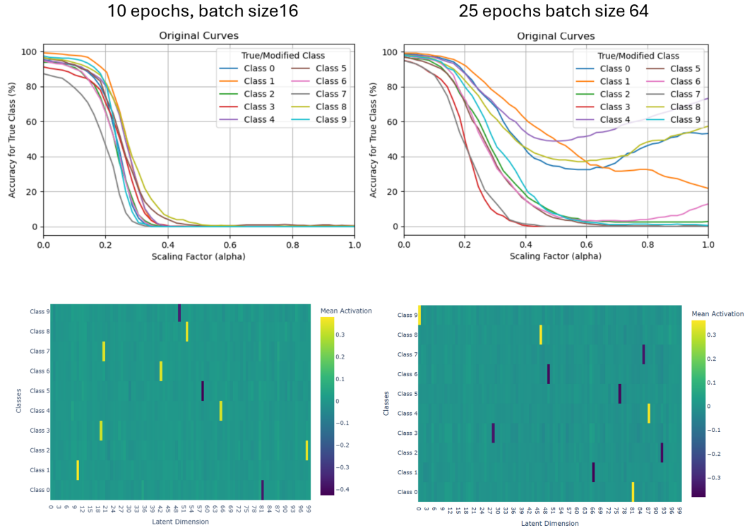
Figure 16: Accuracy vs. scaling factor \alpha for ResNet-18 backbones trained with different initialization and fine-tuning parameters.
