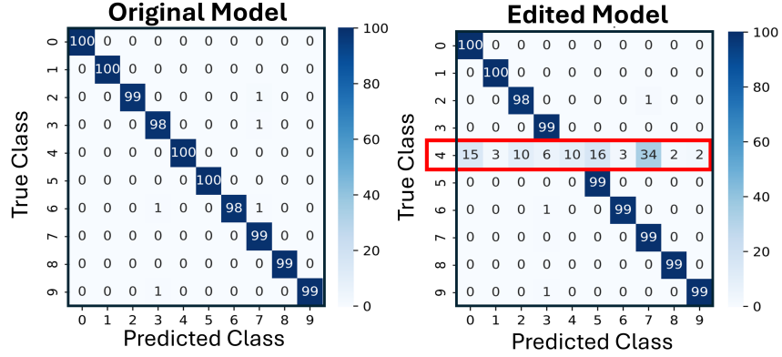
Figure 12: Quantitative validation of feature-guided control in the ViT-B/16 model. The confusion matrices show performance on the test set before (left) and after (right) suppressing the dominant feature for the "Church" class. The intervention effectively ablates the target class while preserving accuracy on the other classes.
