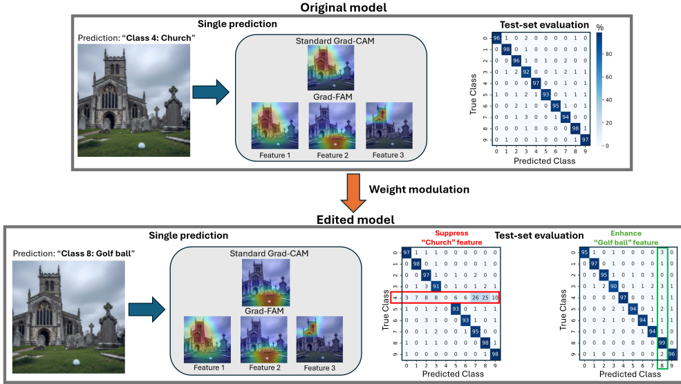
Figure 2: (Left) Qualitative case study: Suppressing the "Church" feature or enhancing the "Golf ball" feature flips the model’s prediction for an ambiguous image. (Right) Quantitative validation on the test set, showing minimal off-target effects
