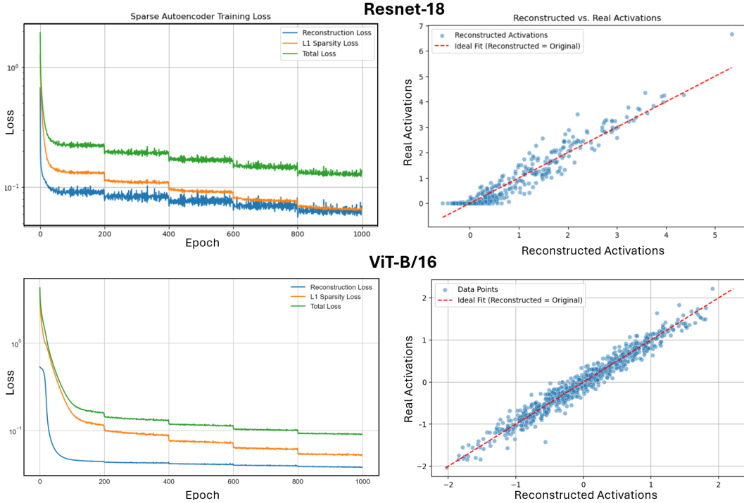
Figure 6: Autoencoder training and reconstruction performance for the ResNet-18 and ViT-B/16 backbones. Left: Training curves for the Sparse Autoencoders, showing total loss, reconstruction loss, and L1 sparsity loss (log-scaled) per epoch. Right: A comparison of the autoencoder’s reconstructed feature activations with the original ones, where the red dashed line indicates perfect reconstruction ( \hat{A} = A ).
