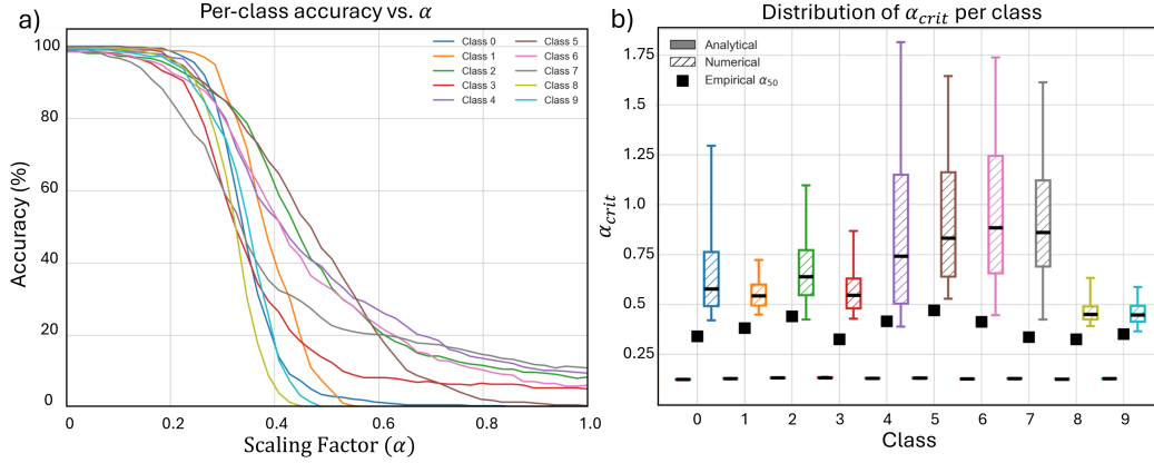
Figure 14: Full class-level sensitivity analysis for the ViT model. (a) Per-class accuracy vs. intervention strength \alpha for all classes. (b) Comparison of analytical (filled), numerical (hatched), and empirical (square marker) \alpha_{\text{crit}} estimates, illustrating the inaccuracy of the linear approximation for the ViT.
