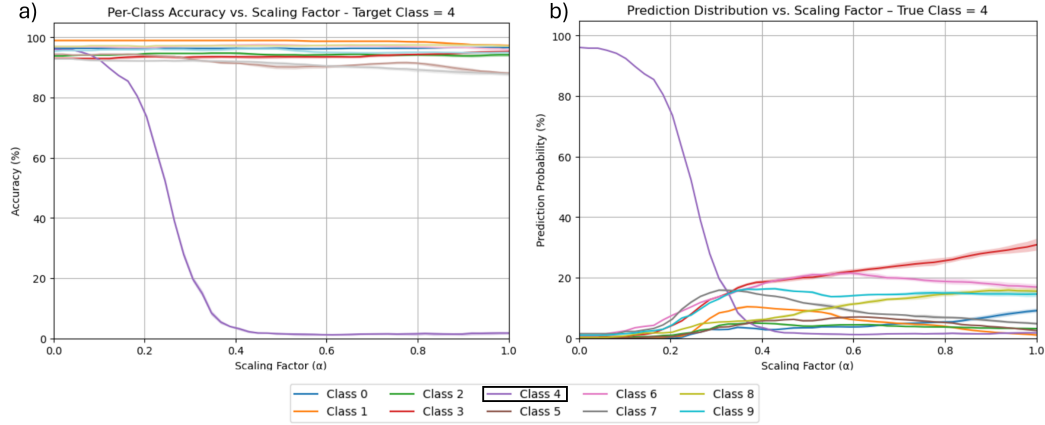
Figure 4: Suppression sensitivity for "Church" (Class 4). (a) Per-class accuracy vs. intervention strength \alpha . (b) Distribution of predictions for images of the target class, showing how confidence is reallocated as the feature is suppressed. Shaded regions indicate the standard deviation across 10 SAE initializations.
