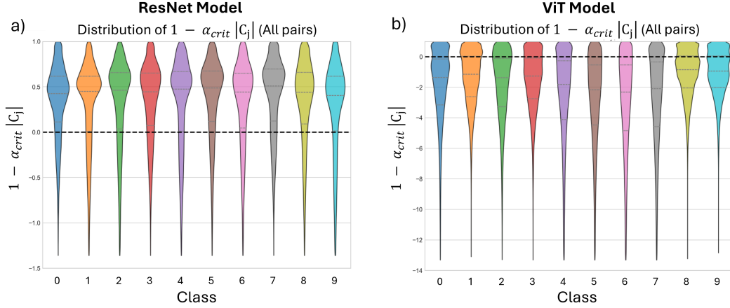
Figure 7: Validation of the linear approximation used to derive the analytical \alpha_{\text{crit}} . The plots show the distribution of the suppression term 1 - \alpha_{\text{crit}} \cdot |c_j| , where negative values indicate the approximation is invalid. (a) For the ResNet-18 model , the distribution is concentrated above zero, confirming the approximation holds for the majority of samples. (b) For the Vision Transformer , a significant mass of the distribution is in the negative region, demonstrating that the linear approximation is invalid for the majority of samples.
