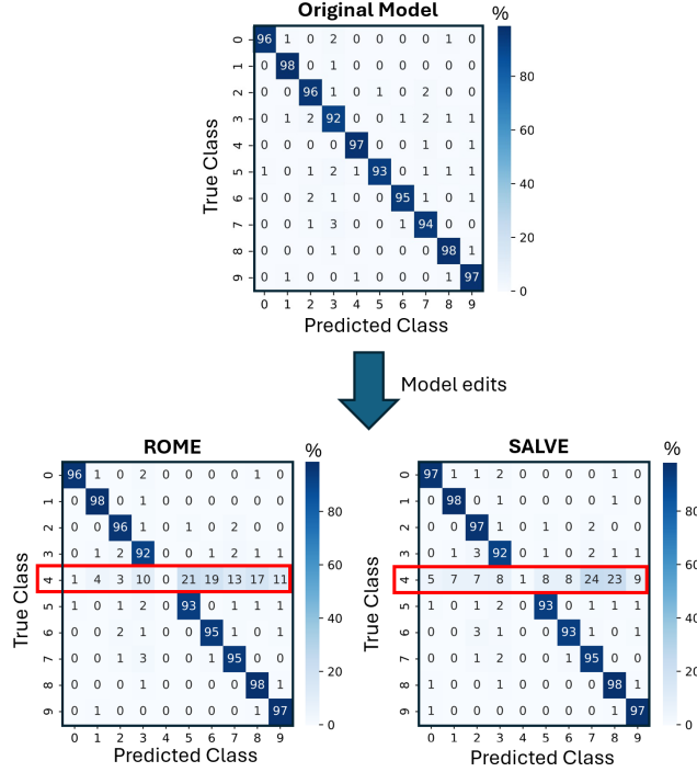
Figure 8: Comparison of class suppression performance. Confusion matrices showing predictions on the test set before editing (top) and after editing (bottom) with ROME and SALVE. Both methods successfully ablate the target class prediction (here shown for class 4).
