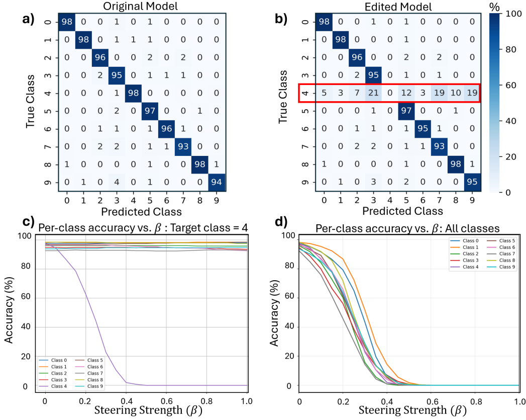
Figure 9: Comparison of class suppression performance. Confusion matrices showing the model’s predictions on the test set before editing (a), and after editing (b) with SAE-based steering vectors. Both methods successfully ablate the target class prediction (here shown for class 4). (c): Suppression sensitivity to steering strength \beta for class 4. (d): Suppression sensitivity to steering strength \beta across all classes.
