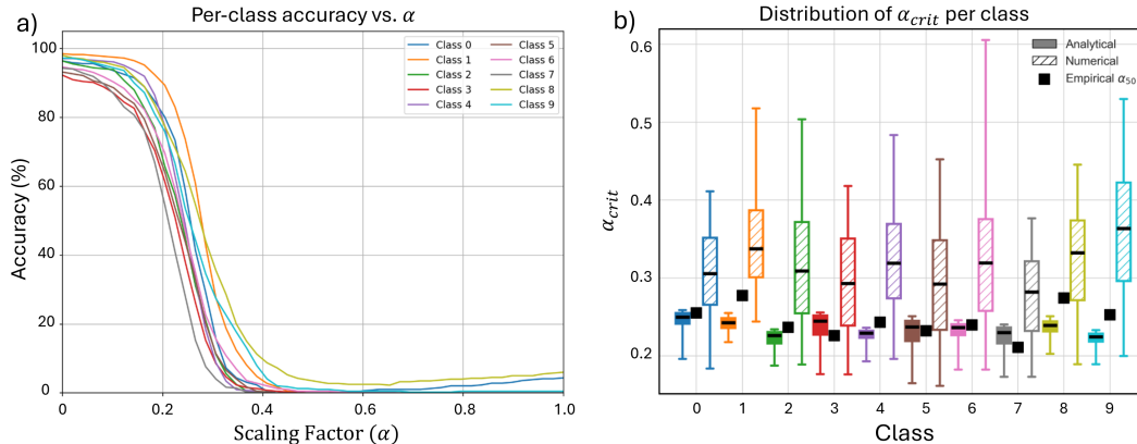
Figure 5: (a) Per-class accuracy vs. the intervention strength \alpha . (b) Comparison of the critical suppression threshold estimates. The distributions of the per-sample analytical (filled box) and numerical (hatched box) \alpha_{crit} are shown as boxplots. The central line indicates the median, the box spans the interquartile range (25th to 75th percentile), and the whiskers extend to the 5th and 95th percentiles. The empirical threshold ( \alpha_{50\%} ) is overlaid as a square marker.
