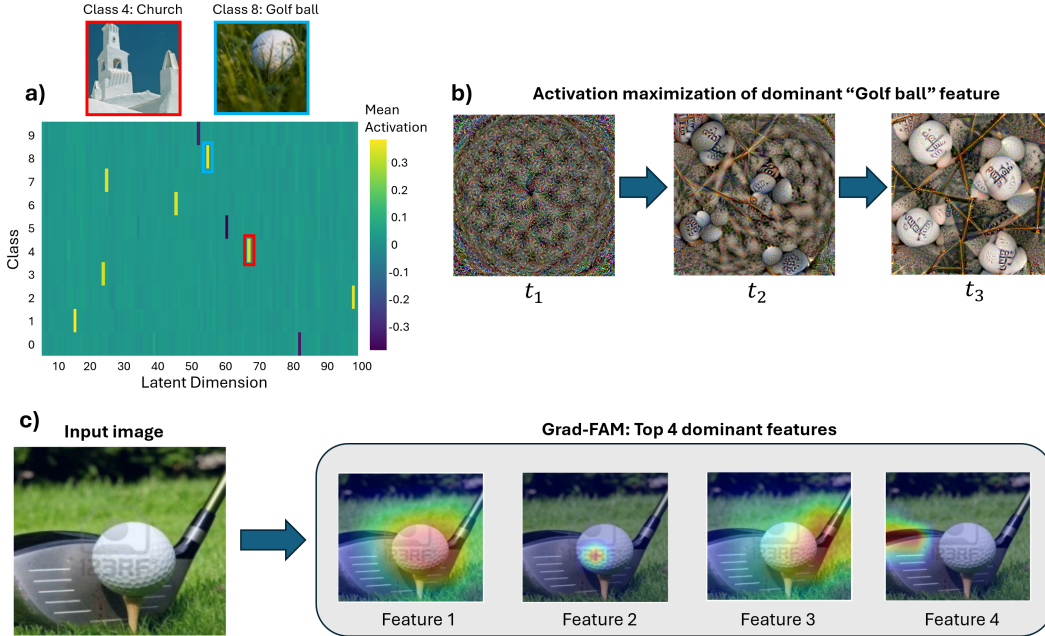
Figure 1: Validation of discovered features for the ResNet-18 model. (a) Average latent feature activations across classes, showing a sparse, class-specific basis. (b) Activation maximization of the "golf ball" feature. The image evolves from random noise ( t_1 ), through emergence of circular shapes ( t_2 ), to the final image clearly exhibiting golf ball characteristics ( t_3 ). (c) Grad-FAM visualizations grounding the top-4 dominant features for a sample "golf ball" image.
