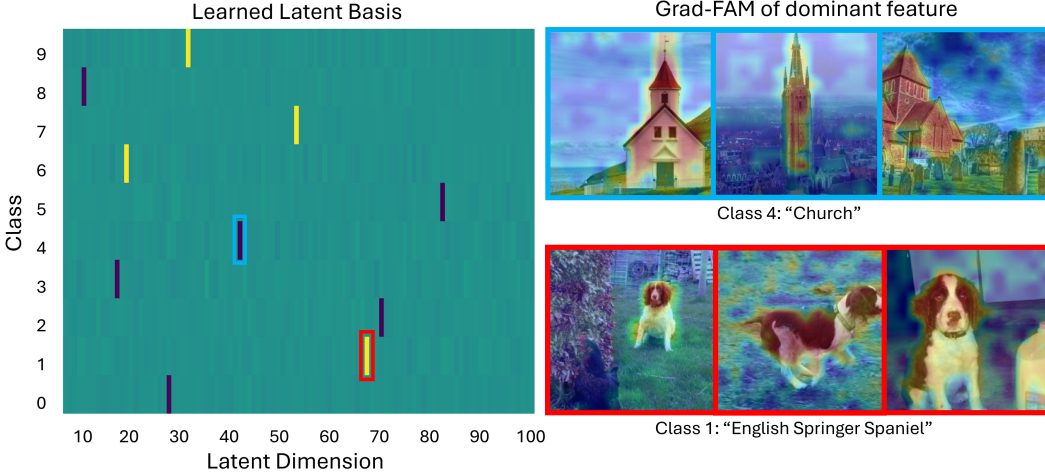
Figure 11: Validation of discovered features for the ViT-B/16 model. (a) Average latent feature activations across classes, highlighting a strong class-specific structure. (b) Grad-FAM visualizations grounding the dominant features for Class 4 ("Church") and Class 1 ("English springer") in representative images.
