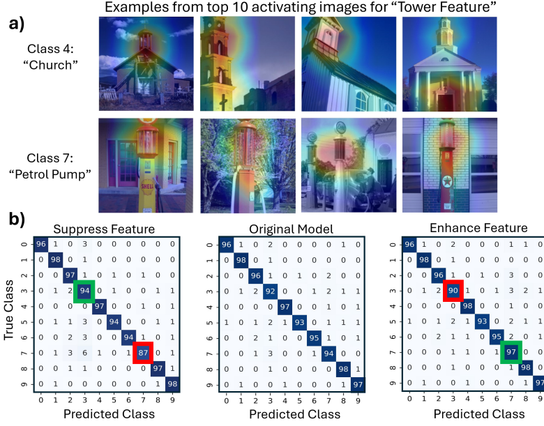
Figure 3: a) Validation of the "Tower Feature", showing example top-activating images from the test set. b) Effect of suppressing and enhancing this feature on model predictions, where "red" and "green" corresponds to decreasing or increasing class accuracy, respectively
