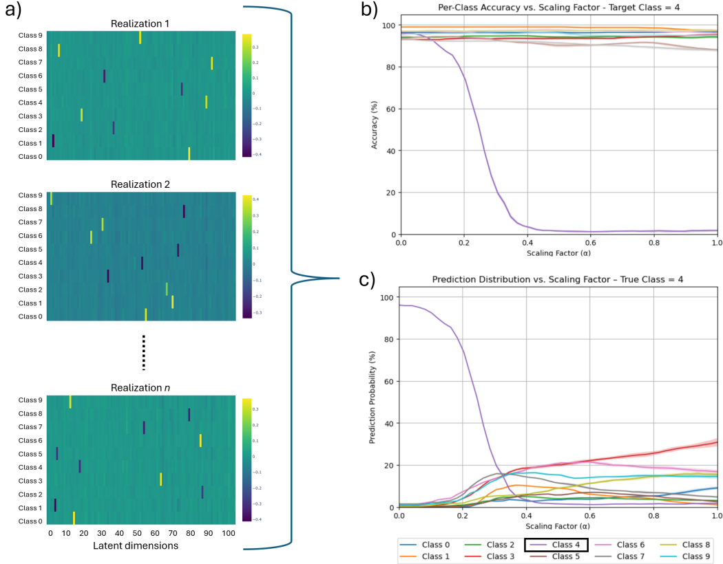
Figure 15: a) Learned latent bases across the n = 10 realizations. b) Per-class prediction accuracy as a function of the scaling factor \alpha , when suppressing the dominant feature associated with class 4. c) Distribution of predictions among the different classes, where the "true" class is 4, showing how the models confidence becomes re-distributed among the other classes. The shaded region in these plots represent the standard deviation across n = 10 different realizations.
