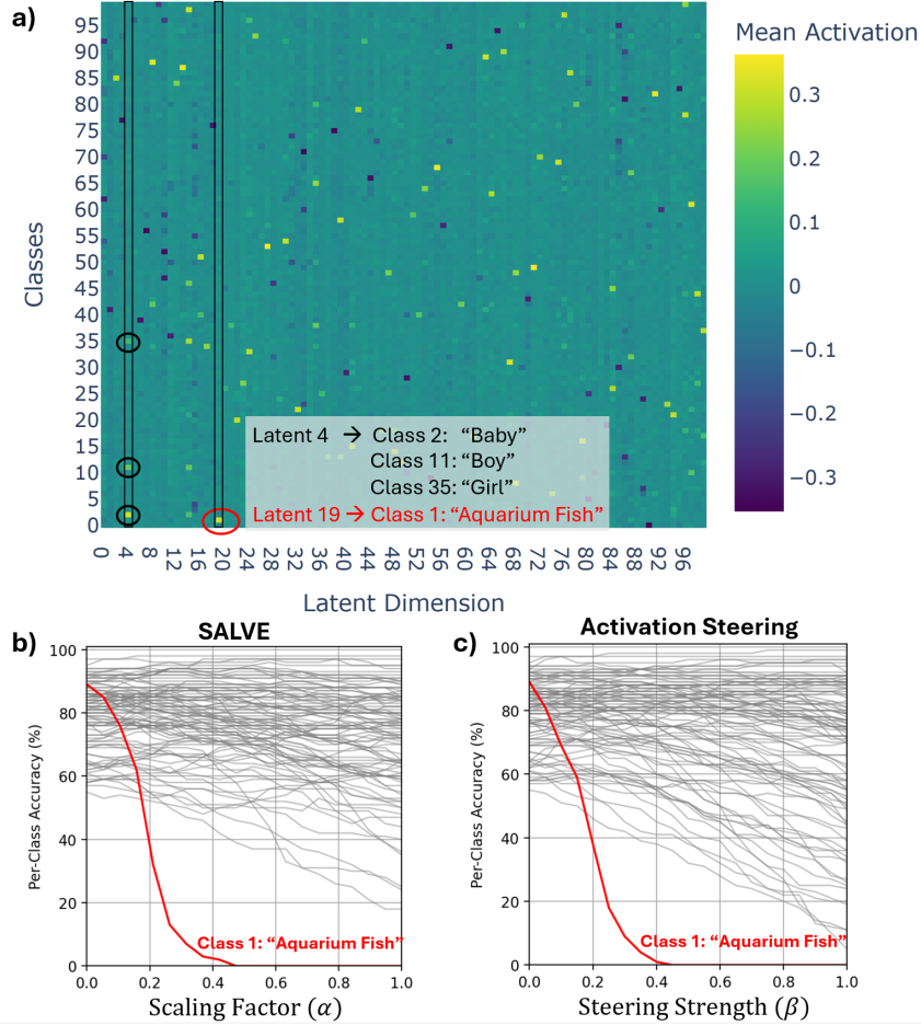
Figure 10: a) Validation of SAE-discovered features for the ResNet-18 model on CIFAR-100. Average latent activations across classes reveal meaningful structure, though with substantially more cross-class overlap than in Imagenette (e.g., Latent 4 activates across multiple human-related classes, whereas Latent 19 is primarily associated with the Aquarium Fish class). b–c) Per-class accuracy when suppressing the dominant latent feature associated with Class 1 (Aquarium Fish), using the same SAE-derived feature basis for both SALVE (b) and Activation Steering (c). The target class is shown in red and all other classes in grey.
