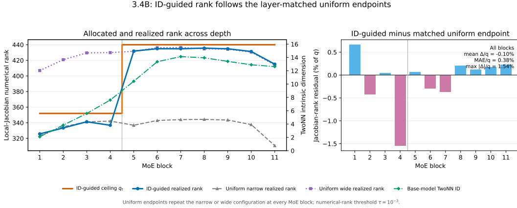
Figure 7: Matched-endpoint realized-rank check at 3.4B. Left: the ID-guided checkpoint’s block-wise local-Jacobian numerical rank, its allocated ceiling q_t , and the realized ranks of the two uniform endpoint checkpoints. The uniform narrow and wide checkpoints repeat their respective (\ell, m, K, N) configurations at every MoE block. Base-model TwoNN ID is shown only as the ordinal signal used to choose the allocation; its numerical scale is not comparable to rank. Right: the ID-guided rank minus the layer-matched uniform endpoint, normalized by q_t .
