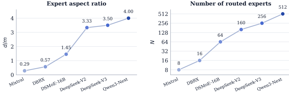
Figure 2: Fine-graining trends across representative MoE architectures. Left: the increasing per-expert aspect ratios d/m . Right: the increasing numbers of routed experts N on a log scale. Values are taken from the corresponding model specifications (Jiang et al., 2024; Databricks AI Research Team, 2024; Dai et al., 2024; DeepSeek-AI, 2024a;b; Team, 2025).
