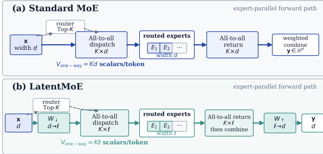
Figure 6: Expert-parallel communication paths. Top: a standard MoE dispatches and returns K vectors of width d per token. Bottom: LatentMoE retains routing decisions in the model hidden space but places the shared down- and up-projections outside the two all-to-all collectives, reducing each routed vector from width d to \ell . Gray dashed arrows show the local routing computation and Top- K assignments; colored arrows show the activation path.
