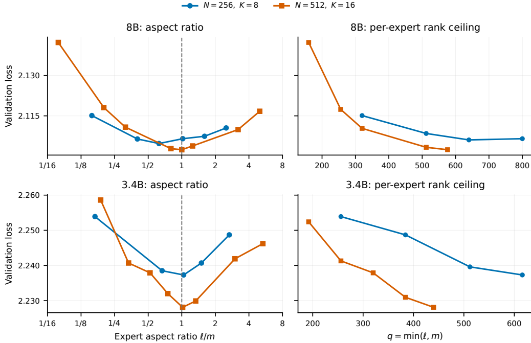
Figure 3: Controlled expert-shape sweeps at two model scales and two routing granularities. Left: validation loss versus aspect ratio; the dashed line marks a square expert. Right: the same runs plotted against the per-expert local-rank ceiling q = \min(\ell, m) , with loss averaged over shapes sharing the same q . Lower is better; Appendix C.1 gives all configurations and losses.
