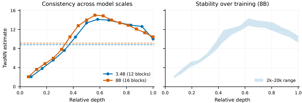
Figure 4: Layerwise TwoNN profiles. Left: final profiles at two model scales exhibit closely aligned variation over relative depth; the color-matched horizontal dashed lines mark the thresholds used to separate the shallow and deeper regimes. Right: the pointwise range across a separate 8B checkpoint series shows that the depth-wise profile is already visible early and persists through training.
