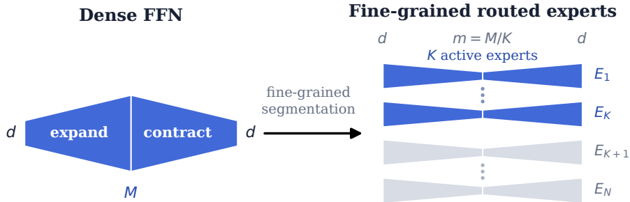
Figure 1: From a wide dense FFN to fine-grained routed experts. Blue denotes the dense FFN and the experts activated for one token; gray denotes inactive experts. Let M denote the dense FFN intermediate width and K the number of experts selected per token. Activated-width matching gives each selected expert intermediate width m = M/K , making each expert much narrower.
