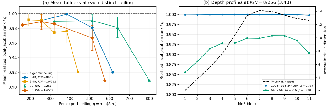
Figure 5: Realized local-Jacobian rank. Left: depth-averaged rank normalized by q ; markers show means, bars show ranges, and the dashed line is the ceiling. Right: blockwise normalized rank for two fixed- q 3.4B models; the dashed curve is base-model TwoNN ID.
