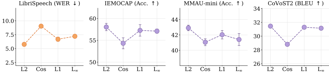
Figure 5: WER/accuracy/BLEU across distance metrics for the transition score, at compression ratio 0.51. Error bars show standard deviation over runs.
