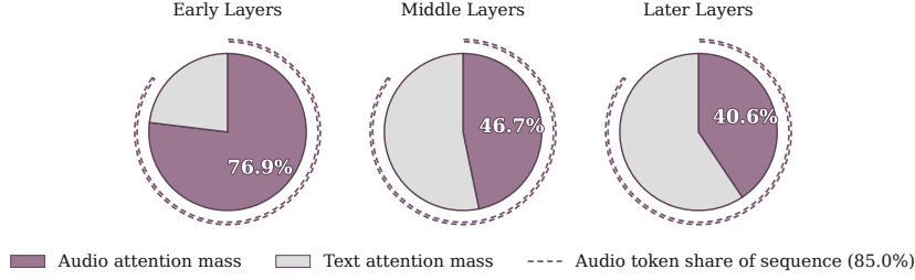
Figure 2: Distribution of decoder attention mass allocated to audio tokens across model depth in Qwen2-Audio on LibriSpeech. Despite audio tokens comprising 84.98% of the input sequence (dashed ring), early layers are dominated by intra-audio attention (76.91%), which drops sharply in middle (46.73%) and late layers (40.60%) as attention shifts to text-conditioned representations. This shift motivates our layer-dependent pooling rule in Eq. 3.
