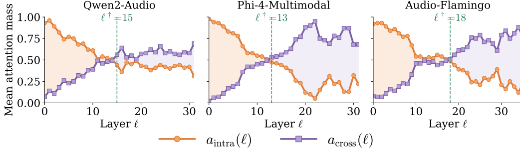
Figure 7: Per-layer intra-audio ( a_{\text{intra}}(\ell) ) and cross-modal ( a_{\text{cross}}(\ell) ) attention mass on the LibriSpeech test-other calibration subset, for Qwen2-Audio (Chu et al., 2024), Phi-4-Multimodal (Microsoft et al., 2025), and Audio Flamingo 3 (Ghosh et al., 2025a). The dashed vertical line marks the identified crossover layer \ell^\dagger for each backbone. Intra-audio attention dominates in early layers and is progressively overtaken by cross-modal attention as depth increases, consistent with Figure 2.
