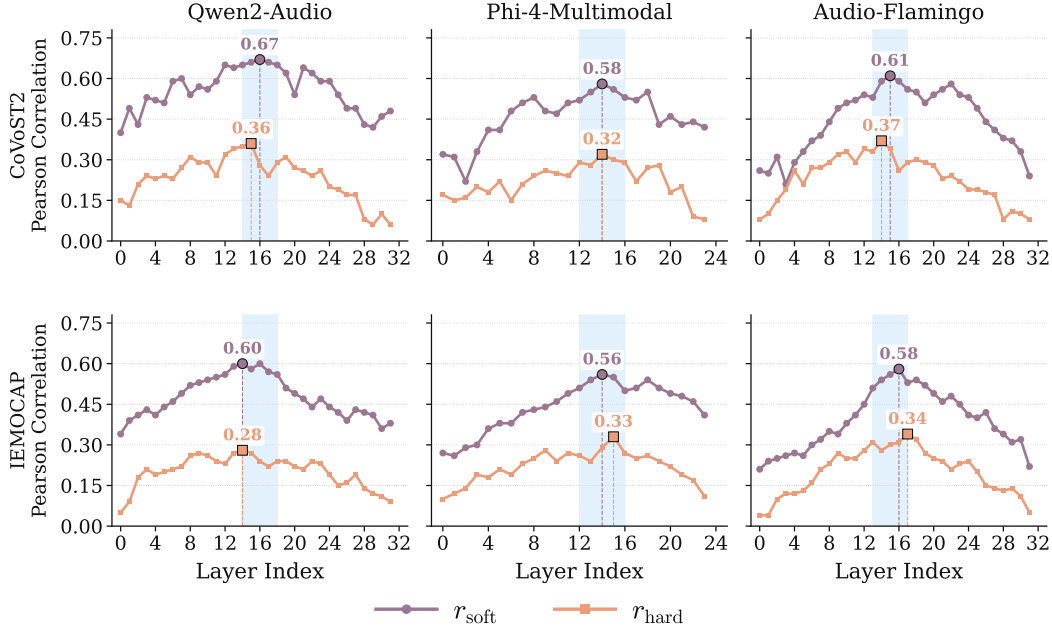
Figure 9: Layer-wise boundary correlation ( r_{\text{soft}} , r_{\text{hard}} ) across Qwen2-Audio, Phi-4-Multimodal, and Audio Flamingo 3, computed on CoVoST2 ( top , MFA alignments generated in-house) and IEMOCAP ( bottom , official released alignments). Shaded regions mark each backbone’s mid-network sweet spot, consistent with Figure 3. Dashed vertical lines and annotated values mark the peak layer for each curve.
