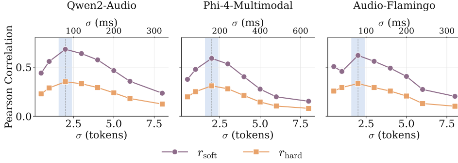
Figure 10: Sensitivity of the transition-prior correlation to the Gaussian smoothing width \sigma , on all backbones. Each panel sweeps \sigma (encoder tokens, with milliseconds on the secondary top axis) and reports r_{\text{soft}} and r_{\text{hard}} at that backbone’s mid-network sweet-spot layer. The shaded band and dashed line mark \sigma = 2 , the value used throughout the main text.
