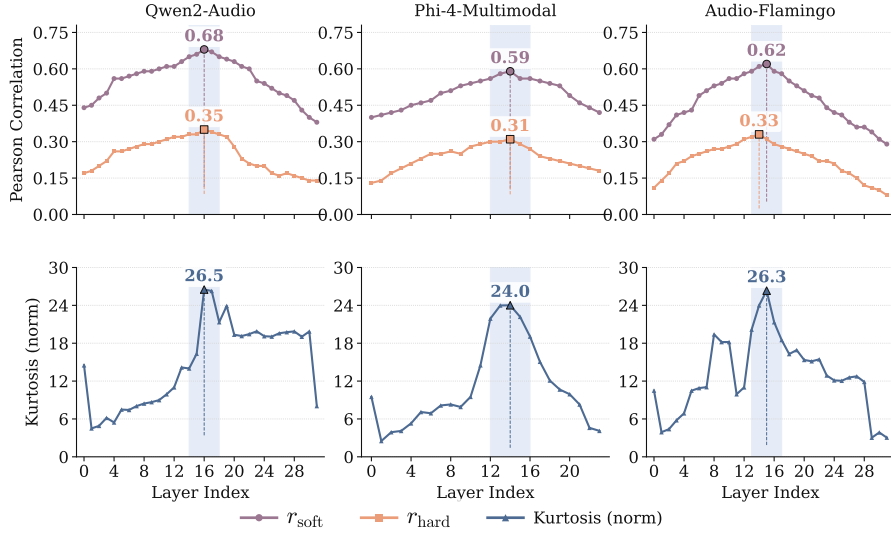
Figure 3: Layer-wise diagnostics across Qwen2-Audio, Phi-4-Multimodal, and Audio Flamingo 3. Top: Mean correlation between b_t and ground-truth phoneme transitions ( r_{\text{soft}} and r_{\text{hard}} ). Bottom: Kurtosis ( \kappa ) of the distance distribution d_t . Both metrics identify an intrinsic mid-network sweet spot (shaded) where phonetic transitions are maximally accentuated.
