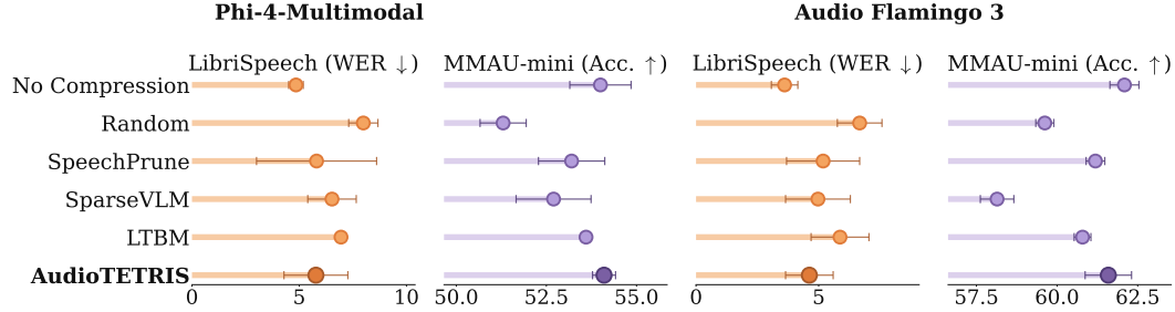
Figure 4: Comparison of LibriSpeech WER ( \downarrow ) and MMAU-mini accuracy ( \uparrow ) at compression ratio 0.51, for Phi-4-Multimodal and Audio Flamingo 3. Error bars show standard deviation across runs. AUDIOTETRIS is highlighted in the darker shade.
