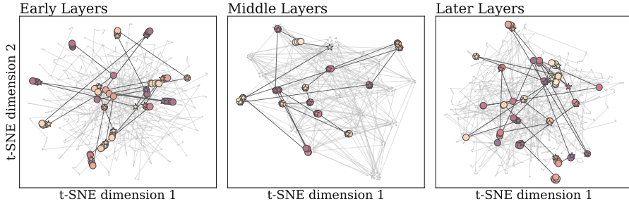
Figure 11: Qualitative analysis of Qwen2-Audio encoder token embedding trajectories for a single LibriSpeech utterance, projected via t-SNE and colored by phoneme identity, at early, middle, and late encoder depths. Colored points \bullet denote individual tokens where different colors represent different phonemes; Star markers \star indicate frames at phoneme transitions per forced alignment; Faint gray points \bullet show other utterances’ frames for spatial context.
