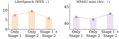
Figure 6: Ablation of AudioTETRIS stages at compression ratio 0.51.
