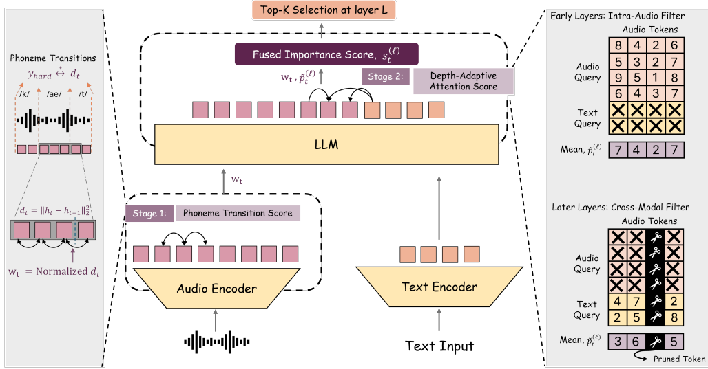
Figure 1: Overview of AudioTETRIS. A phoneme-transition-aware acoustic prior w_t is computed from the audio encoder’s hidden states via the transitional distance d_t = \|h_t - h_{t-1}\|_2^2 , preserving phoneme transitions y_{hard} (§4; left). Token pruning occurs in two stages: Stage 1 injects w_t as a static acoustic prior from the encoder’s hidden states; Stage 2 computes a depth-adaptive LLM attention score, fusing intra-audio attention in early layers with cross-modal (text-to-audio) attention in later layers (right). The two scores are fused into a single importance score, and top- k selection retains the most salient tokens at each pruning layer \ell .
