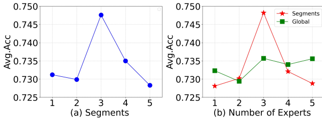
Figure 3: Experiments on 30 UEA datasets to evaluate different structural configurations, we report the average accuracy.
