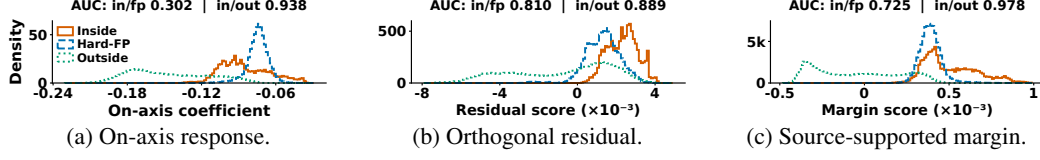
Figure 3: Text-response entanglement and source-supported re-ranking. Raw on-axis scoring strongly overlaps true defects with hard false positives. The orthogonal residual improves defect-vs-hard-FP separation in this case, but weakens separation from generic outside regions. The source-supported margin re-ranks the same responses while preserving strong outside separation, showing that TED decomposes rather than discards the text-guided response.
