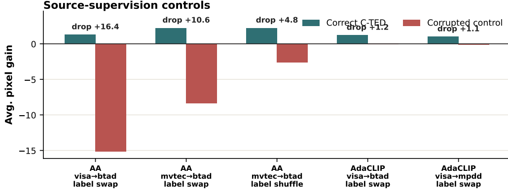
Figure 8: Source-supervision controls for C-TED. All variants use the same source split, source-bank size, residual capacity, and calibration budget. Correct C-TED preserves the defect-versus-hard-FP assignment, while label shuffle and label swap corrupt only the supervision semantics.
