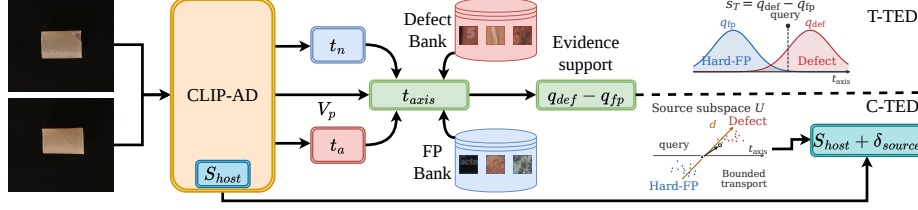
Figure 2: Overview of TED. The host provides patch features ( V_p ) and normal ( t_n )/anomaly ( t_a ) text embeddings that define the host text axis. TED projects query patches and source defect/hard-FP features onto this axis to compute a defect-versus-hard-normal support margin. T-TED uses this margin as a train-free local score, while C-TED converts it into a bounded residual anchored to the host score.
