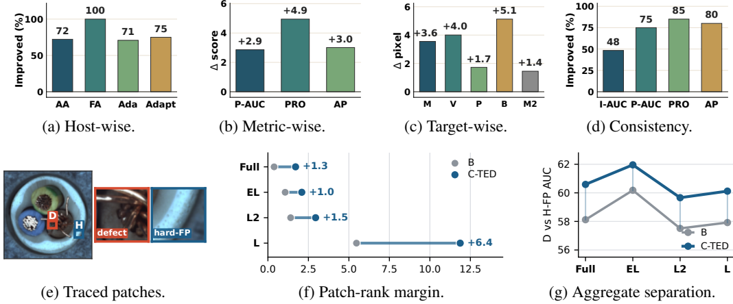
Figure 6: Adapted-host and recipe-retuning diagnostics. Top: source-calibrated TED improves local pixel ranking across adapted CLIP-AD hosts; M, V, P, B, and M2 denote MVTec AD, VisA, MPDD, BTAD, and MVTec AD 2, respectively. Bottom: changing and retraining layer recipes shifts the host response, but the same traced defect and hard-FP patches remain competitive under the baseline. C-TED increases the patch-rank margin and yields cleaner aggregate separation between defect-supported and hard-normal-supported responses.
