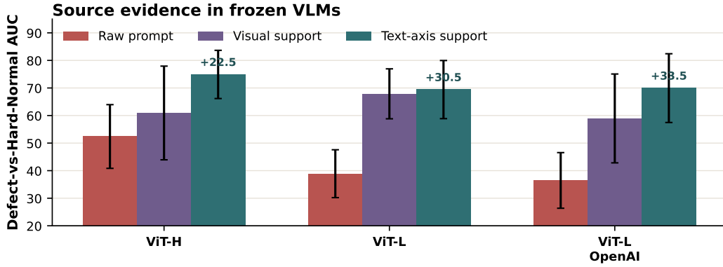
Figure 9: Raw VLM source-support ablation. Raw prompt scoring is compared with source-supported readouts in frozen VLM backbones. Text-axis support projects query and source-bank features onto the normal-versus-anomaly text axis, while visual support uses the source banks.
