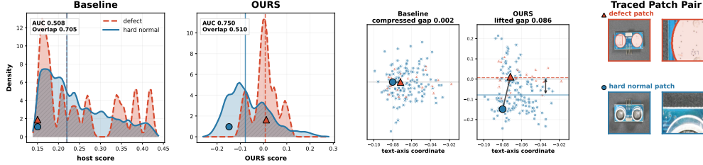
Figure 5: Hard-FP decomposition in an adapted host. The baseline assigns overlapping high scores to true defect and hard-normal patches. TED re-scores the same responses with source defect and hard-FP evidence, reducing overlap and lifting the defect–hard-normal ranking gap.
