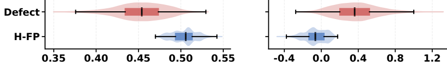
Figure 4: Patch-level failure of raw prompt scoring. The left panel shows the raw prompt baseline and the right panel shows TED. The baseline ranks hard-normal patches close to or above true defects, whereas TED re-ranks them using source defect and hard-FP support without backbone or prompt adaptation. H-FP denotes hard false positive.
