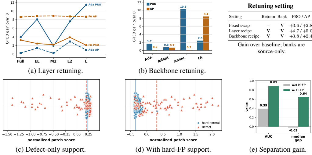
Figure 7: Recipe-consistent retuning and hard-FP support. Top: C-TED remains beneficial after changing the feature-layer or backbone recipe, retraining the host when applicable, and rebuilding source banks for the resulting representation. Bottom: defect-only support leaves defect and hard-normal patches entangled, whereas adding hard-FP support explicitly models the competing hard-normal evidence and produces a cleaner local ranking margin.
