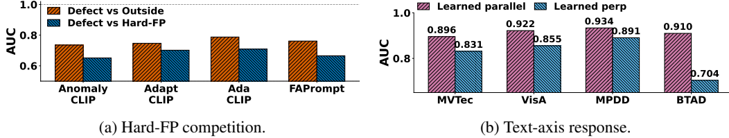
Figure 1: Hard-FP competition and text-axis response. (a) Across adapted CLIP-AD hosts, true defects remain much harder to separate from hard false positives than from generic outside patches. (b) Across target datasets, the learned text-axis response is consistently more informative than the orthogonal component, suggesting that the axis should be decomposed rather than discarded.
