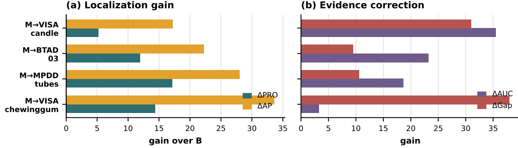
Figure 12: Failure-conditioned class-level cases. Representative target classes where C-TED improves localization while also increasing defect-versus-hard-FP AUC and the defect-minus-hard-FP score gap.
