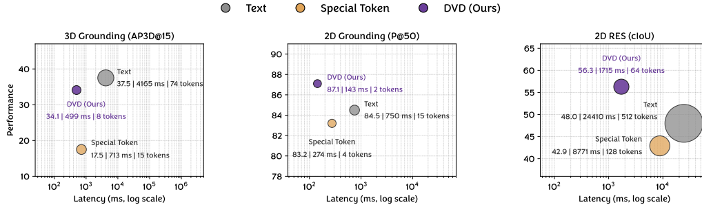
Figure 4: Computation cost and performance comparison of different representations. Bubble area indicates the token count generated for per object of the representation.
