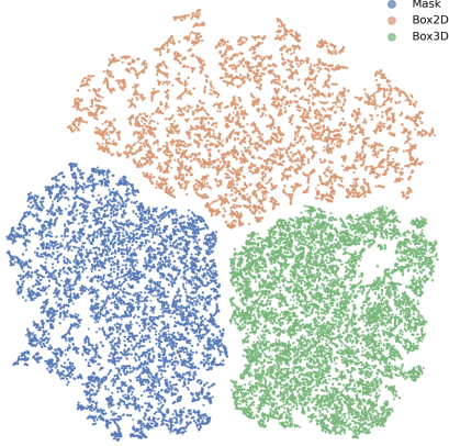
Figure 7: The visualization of latent space in DVD with t-SNE for unifying 2D and 3D perception tasks. There are there obvious clusters, illustrating the effectiveness of our dynamic vector representation learning process.
