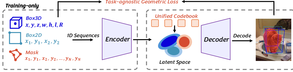
Figure 2: The illustration of the dynamic vector representation learning. We first use the 1D sequence as 2D and 3D perceptual representation. Then, we use an encoder to map these sequences to high-dimensional space to adaptively quantize and compress these 1D information. Moreover, we introduce the task-agnostic geometric loss to improve the heterogeneous perception representation learning capacity. Finally, we use a decoder to recover discrete tokens to original representation.
