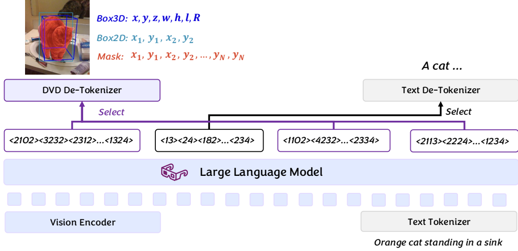
Figure 3: Overview of DVD. We extend the MLLM vocabulary with learned unified tokens and train the model following standard LLM paradigms without modifications. At inference, we select tokens belonging to perception tasks and use a lightweight de-tokenizer reconstructs the original perceptual outputs from the discrete tokens with minimal overhead, drastically reducing sequence length and improving efficiency.
