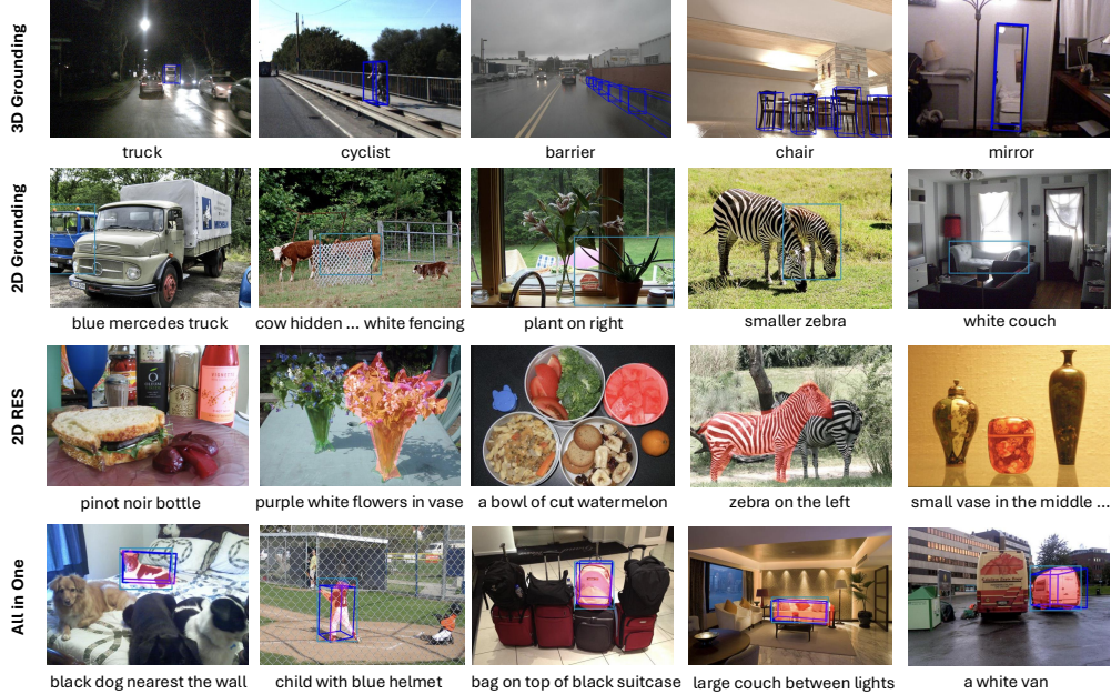
Figure 5: The qualitative visualization of DVD on the 2D and 3D perception tasks. The first row is the results of 3D grounding task. The second row is the result of 2D grounding task. The third row is the results of 2D RES task. The fourth row is the results of unified perception.
