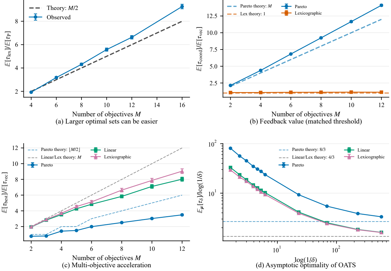
Figure 1: Synthetic results for Propositions 1–3 and Theorem 2. (a) The ratio \mathbb{E}[\tau_{\text{lex}}]/\mathbb{E}[\tau_P] grows with M : Pareto-set identification becomes increasingly easier than lexicographic identification. (b) The feedback gain \mathbb{E}[\tau_{\text{coord}}]/\mathbb{E}[\tau_{\text{vec}}] grows with M under the Pareto order but remains near one under the lexicographic order. (c) The gain \mathbb{E}[\tau_{\text{best}}]/\mathbb{E}[\tau_{\text{vec}}] increases with M under all three orders and stays above one, confirming multi-objective acceleration. (d) The normalized stopping time \mathbb{E}_\mu[\tau_\delta]/\log(1/\delta) decreases toward the corresponding characteristic time as \delta decreases. Markers show empirical means with 95% confidence intervals, and dashed lines show theoretical predictions.
