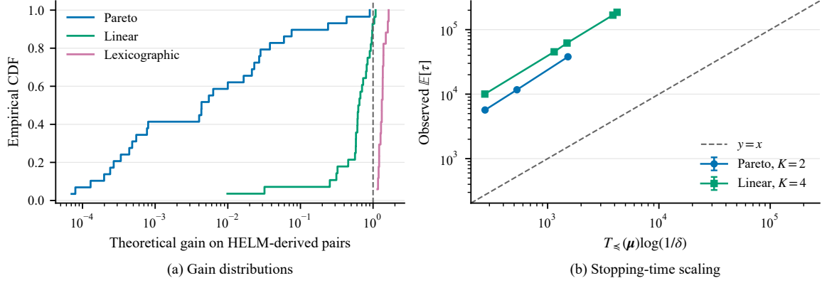
Figure 2: HELM-derived Gaussian instances. (a) Empirical CDF of the theoretical gain across within-scenario model pairs; a gain above 1 indicates a multi-objective speedup over the best scalar benchmark. (b) Observed stopping time versus T_{\leq}(\boldsymbol{\mu}) \log(1/\delta) for eligible Pareto and linear instances, showing that T_{\leq}(\boldsymbol{\mu}) captures instance difficulty on HELM-derived geometries.
