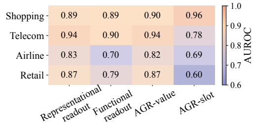
Figure 3: Cross-domain diagnostic AUROC of the evaluated readouts under in-domain and zero-shot configurations.
