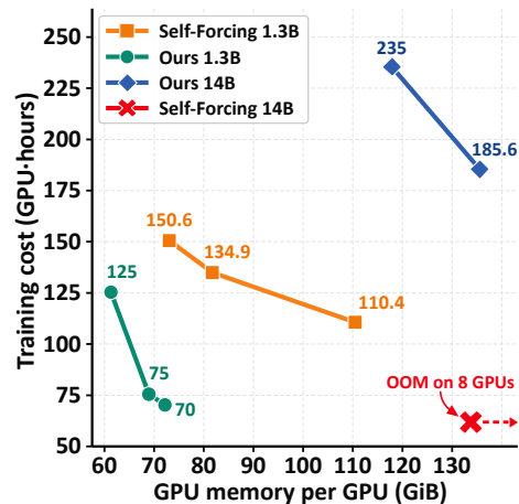
Figure 6. Training efficiency. The tradeoff between GPU hours and peak memory per GPU (due to different offloading strategies) at 1.3B and 14B scale. Self Forcing 14B runs out of memory on eight GPUs.
