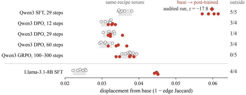
Figure 1: LoRA-SFT moves the co-activation graph further from its base than its own reruns sit apart, on two backbones; DPO’s contrasts sit at their band’s edge, light GRPO’s inside it. Rows are the arms of Table 1; shading spans the seed-pair distances (open circles; a range, not an interval); filled points are base-to-post contrasts (diamond: audited SFT check-point); counts are contrasts beyond every seed pair. DPO’s band counts (3/4, 1/4, 3/4 contrasts outside at 12/29/60 steps) follow no dose ordering. All graphs in a row were built on one GPU architecture (H200). Drawn by code/analysis/fig1_rl_strip.py from results/{sftband.20260926, graph_build_audit.20261005}/ .
