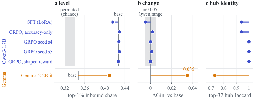
Figure 2: The concentration a single-checkpoint study would credit to RL is already present in the zero-RL base. One row per checkpoint in the base-diff summary. (a) Top-1% inbound share: every Qwen checkpoint sits on or next to its base (vertical rule), far from the degree-preserving permutation null of the base graph (95% range shaded). (b) Change in Gini against the base; the shading is \pm the largest |\Delta\text{Gini}| among the five Qwen rows (0.005), not a statistical null. (c) Top-32 hub Jaccard against the base. Gemma-2-2B-it is a different family and a heavier recipe; the comparison is descriptive. Receipts: notes/basediff- \{qwen, gemma\} -summary.json , h1_permutation_null_1p7b_1l14to22.json .
