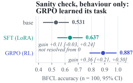
Figure 3: Sanity check: GRPO did learn the behavior it was trained for. On the held-out BFCL validation split (100 items, 40/20/20/20 over four categories, from the same release files as the training rows; accuracy is the unweighted category mean), GRPO improves accuracy +0.36 over base (95% CI [+0.21, +0.50]); SFT’s +0.11 is not resolved from zero by this harness ([−0.03, +0.24]). Intervals are stratified normal approximations and the gains are unpaired (notes/bfcl_behavior_ci.json, code/scripts/bfcl_behavior_ci.py). Only behavior is plotted — there is deliberately no internal axis here , because placing the two on one pair of axes is the withdrawn dissociation claim drawn: accuracy is measured on BFCL task states, displacement on general text, and the matched on-task internal arm fails its own positive control (App. J, L5). The corresponding internal readings are reported where they are calibrated (Sec. 4.2), not here.
