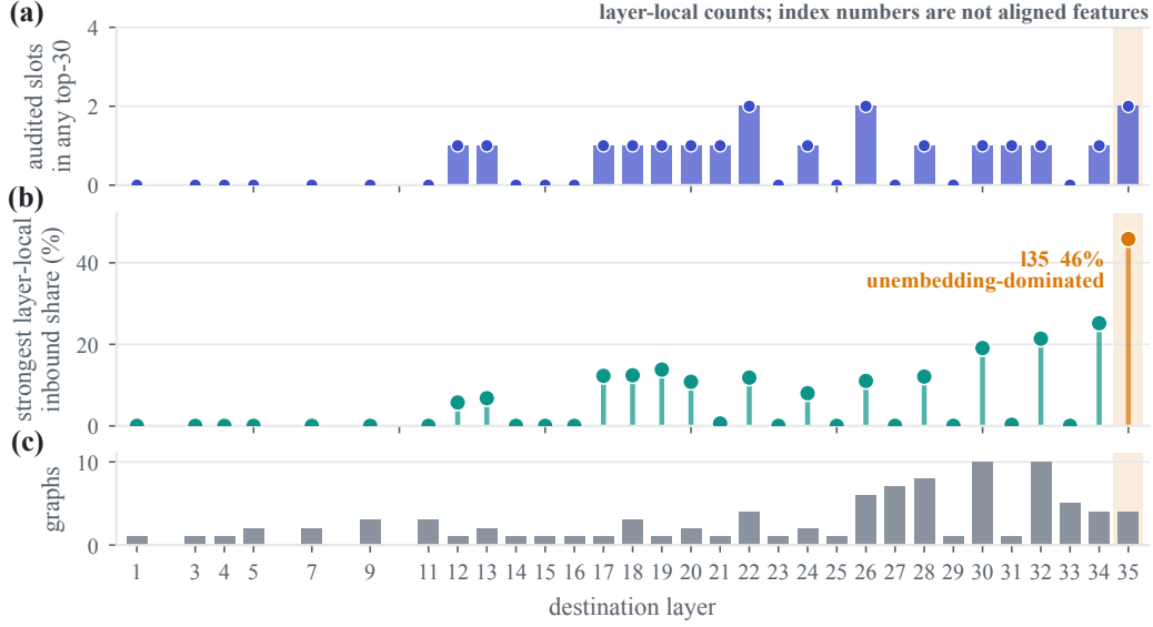
Figure 7: A layer-local diagnostic of the audited index slots. (a) Count of the fifteen audited integer slots present in any top-30 set at each destination. (b) Their maximum inbound share within that destination. (c) Number of available source graphs. The SAE dictionaries were trained independently by layer: identical integer indices are not aligned features. This plot therefore reports local slot statistics, not cross-layer feature recurrence or preserved feature identity. Layer 35 is unembedding-dominated. Receipt: notes/fig8_backbone_recurrence_data.json ; generator code analysis/fig8_layer_index_diagnostic.py .
