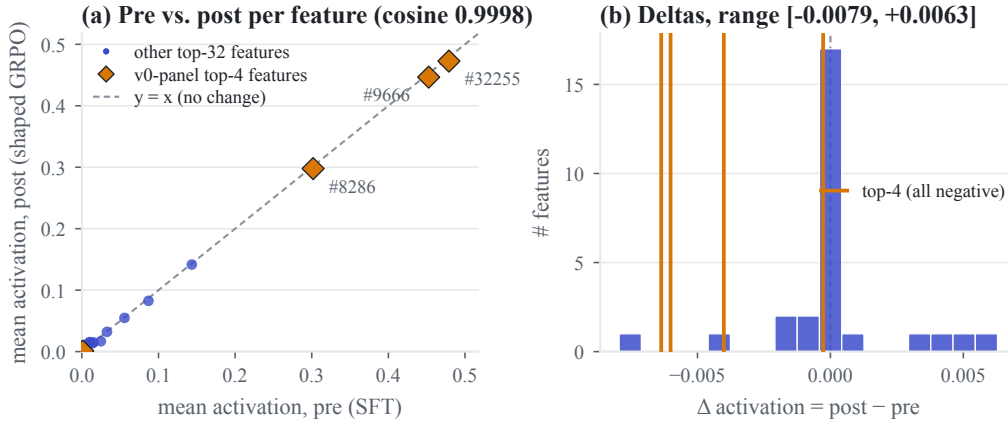
Figure 8: H2 per-feature delta diagnostic (cross-tokenizer, n = 16 probes). (a) Per-feature mean activation pre (SFT) vs. post (shaped-reward GRPO, shaped- \lambda 0.1 arm), 32 features. v0-panel top features (amber diamonds) sit on the diagonal with small negative deltas, consistent with this arm’s reward penalizing the panel’s activations. (b) Histogram of post–pre deltas; the four v0-panel top features are marked. Cosine 0.9998 is consistent with the delta magnitudes shown ( \sim 5\% of pre-activation mean), not numerical precision.
