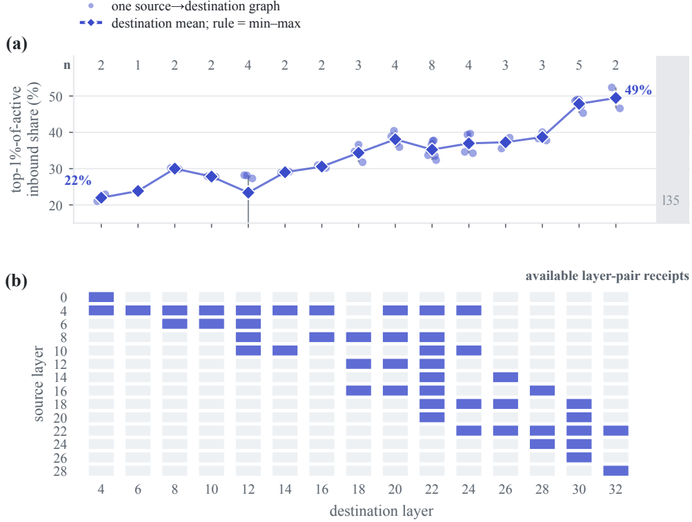
Figure 4: Available layer-pair coverage and concentration. Every point is one source-to-destination co-activation graph; diamonds are destination means and rules the observed min-max range. Numbers above the plot count available source layers. The lower panel shows the unbalanced source/destination coverage. The rise from about 22% to 49% is descriptive of this available scan, not an isolated destination-depth effect. Terminal layer 35 is excluded as unembedding-dominated. Source: the 47 committed Qwen3-8B layer-pair receipts ( notes/attribution_graph_v1_qwen3-8b_l1*to*.json ); generator code/analysis/fig7_concentration_vs_depth.py .
