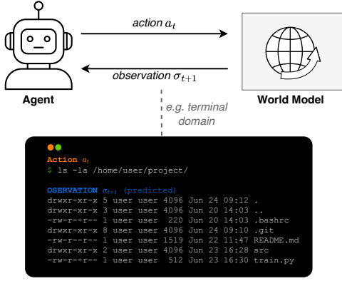
Figure 3: The world model predicts the next textual observation o_{t+1} from the agent’s action a_t and interaction history, shown here for the Terminal domain, where the action is a shell command and the predicted observation is its terminal output.
