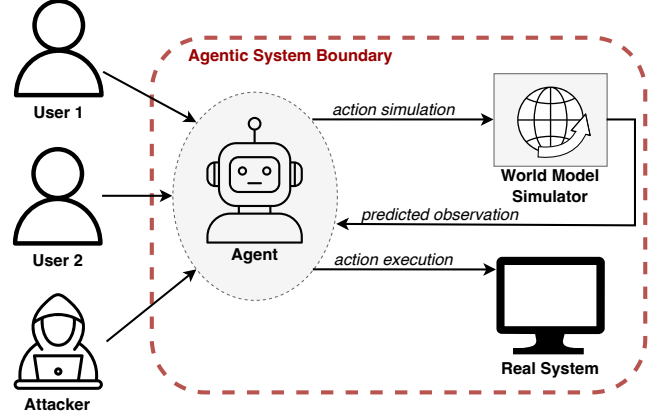
Figure 4: Agent simulating actions with a world model, checking whether to execute them in the real system.
