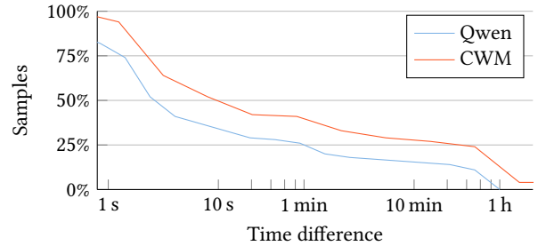
Figure 6: Cumulative distribution of the difference in predicted time between the world model simulation and sandbox. Each line shows the proportion of samples satisfying a minimum time difference.
