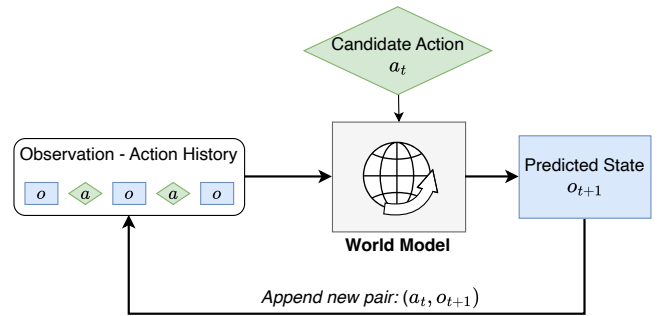
Figure 2: The world model \mathcal{M} predicts a new environment state o_{t+1} based on a history of past observations with past actions and one chosen action a_t
