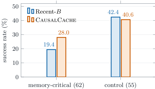
Figure 3: The core contrast at the primary budget: on construction-defined memory-critical tasks CAUSALCACHE gains +8.6pp over the same-budget recent allocation, while on matched single-app controls no effect is detectable; the split-by-method interaction is significant ( p=0.022 ).
