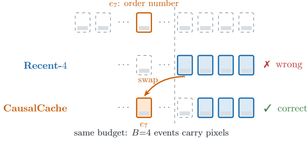
Figure 1: CAUSALCACHE on a real cross-app episode (schematic; drawn with B=4 ). The agent must compose an SMS containing the order number it saw earlier in a shopping app. Every event persists as a one-line text summary; a budget of B events may additionally carry their archived pixels. After the app switch the evidence frame e_7 lies outside the recent window: Recent- B spends every slot on the latest events and types the wrong number, while CAUSALCACHE swaps one recent slot for e_7 at the same budget and succeeds.
