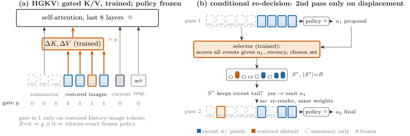
Figure 2: The two learned components of CAUSALCACHE. (a) The history-gated K/V interface (HGKV): a low-rank \Delta K, \Delta V branch on the last eight frozen self-attention layers is multiplied by a binary token gate g that is 1 only on restored history-image tokens, so current-screen, text, and response tokens pass through unchanged, and at B=0 the gate vanishes and the policy is bitwise-identical to the frozen base. (b) Proposal-conditioned re-decision: pass 1 renders the default Recent- B allocation and yields a proposal a_1 ; a two-tower scorer conditioned on per-event features with a_1 as witness and on budget context scores the complete summarized trace and returns the exact- B set S^* . If S^* keeps the recent tail, a_1 is emitted with no extra compute; only when a recent event is displaced is the prompt re-rendered under S^* and the same frozen weights generate the final action a_2 . Event cards follow Figure 1: dashed gray = summary-only, blue = recent with pixels, orange = promoted distant event; orange-outlined boxes are the trained modules; snowflakes denote frozen components.
