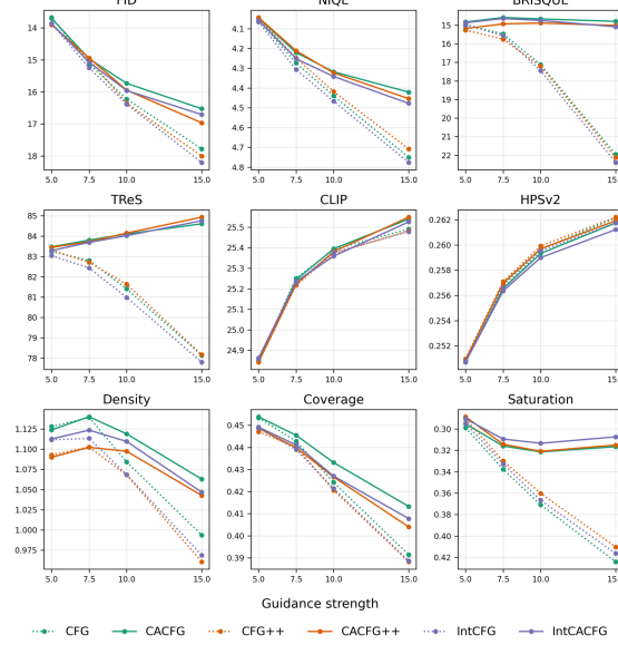
(a) ImageNet
