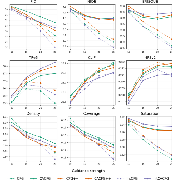
(a) ImageNet
