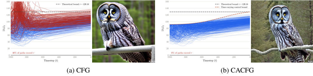
Figure 1: Tweedie’s magnitude ( \|\hat{x}_0(t, x_t, \xi)\|_2 ) of diffusion sampling trajectories across time with \omega = 7.5 and using (a) CFG (Ho & Salimans, 2022) and (b) CACFG (ours), alongside a representative sample generated by each method. Note that 40% of CFG sampling paths violate the theoretical 95% upper magnitude bound. CACFG restricts permissible controls to lie within a time-varying bounded control set.
