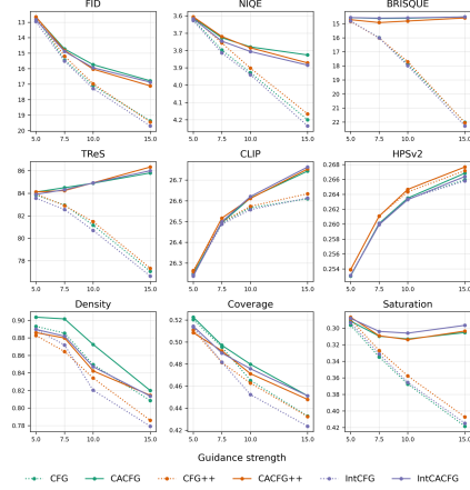
Figure 2: Performance of CFG, CFG++, and IntCFG with (solid line) and without (dotted line) our curvature-aware correction using SD1.5 on COCO. Some metric axes have been flipped so that the improvement direction is vertically up the page. Zoom in for easier viewing.
