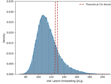
Figure 5: Empirical distribution of SD1.5 VAE encodings ( \|x_0\|_2 ) of the ImageNet validation set, i.e. the distribution of \|x_0\|_2 . Red line denotes the theoretical chi density implied by the Gaussian hypothesis in Section 5.
