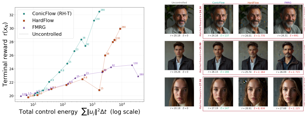
Figure 2: Trade-off between terminal reward and total control cost. Left: Reward vs. control energy on the editing task, traced by sweeping \lambda (upper left is better). Right: Edits from each method at approximately matched reward; ConicFlow reaches the same reward with much lower control energy.
