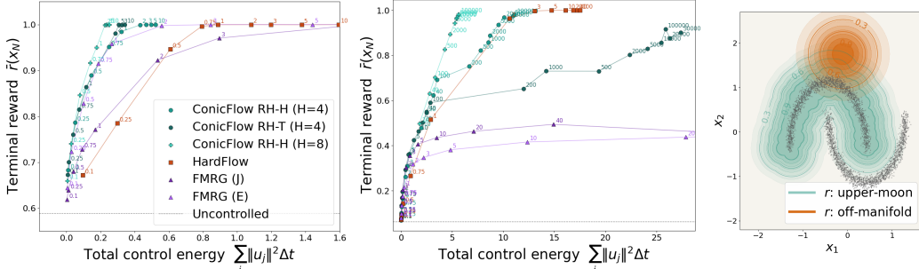
Figure 1: Trade-off between terminal reward and total control cost, traced by varying the control-cost weight \lambda (upper left is better). Left: easy reward (upper moon). Middle: difficult reward (off-manifold). Right: uncontrolled sample distribution and both rewards.
