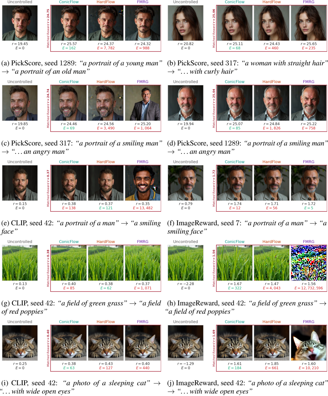
Figure 5: More examples of unconstrained editing. Each panel is one (reward, prompt, seed) instance at a matched-reward level. Panels g–j are the harder case: turning a green field red, or opening a sleeping cat’s eyes, asks for the image to be restructured rather than adjusted, and no method delivers it.
