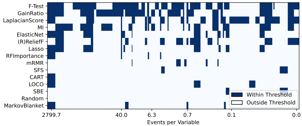
Figure D.11: Thresholded validity at 100% added noise. We display all methods within a 3% performance threshold of the best-performing method at a noise level of 100%.
