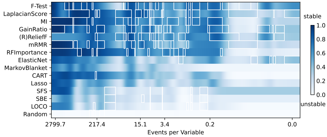
Figure D.4: Stability. Nogueira score (Nogueira & Brown, 2016) across datasets. We use the events per variable, i.e. , the number of samples per feature for regression problems or the number of samples in the minority class per feature for classification problems, as a proxy for the selection difficulty (Harrell, 2015; Heinze et al., 2018). The top-3 methods per EPV are highlighted.
