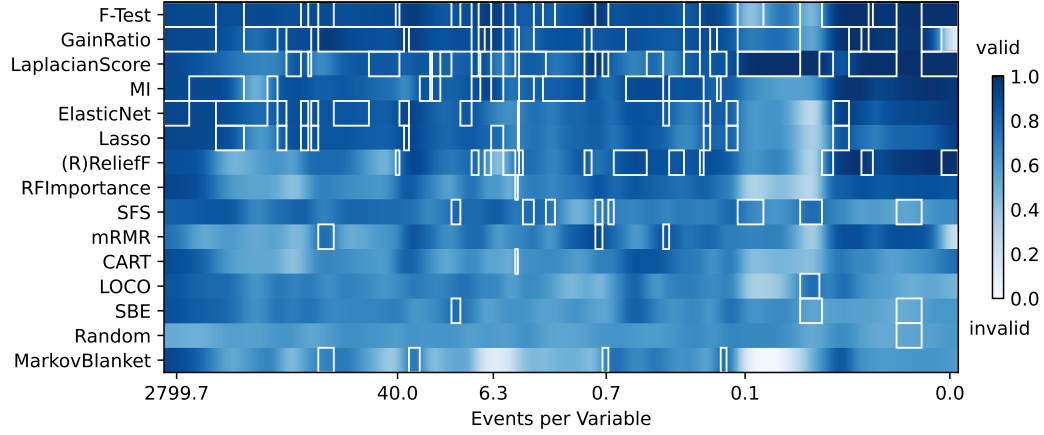
Figure D.8: Validity at 75% added noise. Selection precision across datasets at a noise level of 75%. Like for the stability, we use the events per variable, i.e. , the number of samples per feature for regression problems or the number of samples in the minority class per feature for classification problems, as a proxy for the selection difficulty (Harrell, 2015; Heinze et al., 2018). The top-3 methods per EPV are highlighted.
