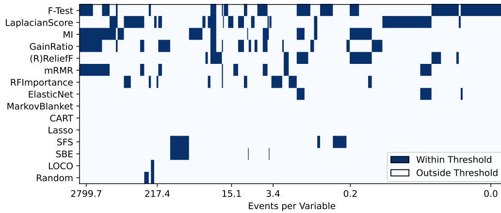
Figure D.5: Thresholded stability. We display all methods within a 3% performance threshold of the best-performing method.
