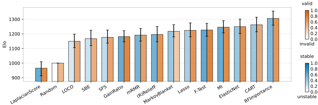
Figure 1: SelectArena at a glance. We present Elo ratings of the 15 feature selection methods ordered left to right from worst- to best-performing method. Elo rating summarizes how often a method beats another on the same dataset, budget, and downstream model, with random selection anchored at 1000 (Appendix D.2). Error bars are 95% confidence intervals from 1000 cluster bootstrap resamples over the 71 datasets. The left bar of each pair is shaded by stability (how much the selected subset changes across resamples) and the right bar by validity (how well injected noise features are rejected), where darker is better for both.
