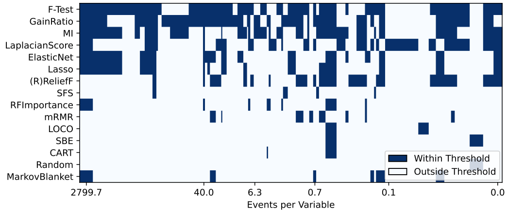
Figure D.7: Thresholded validity at 50% added noise. We display all methods within a 3% performance threshold of the best-performing method at a noise level of 50%.
