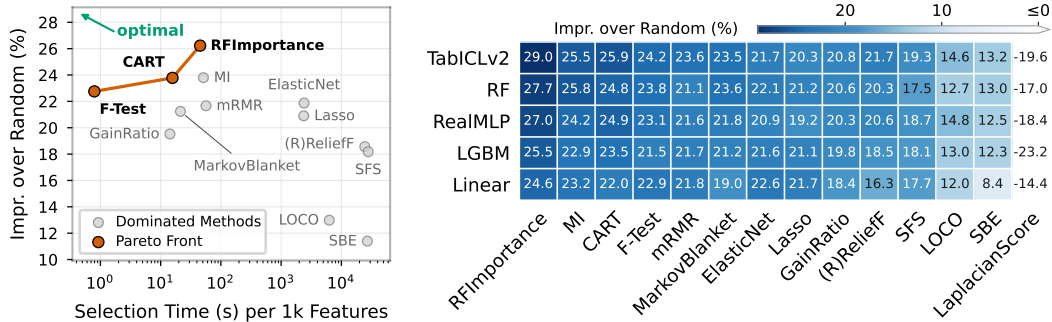
Figure 4: Predictive performance. Both panels report improvement over RANDOM (%), averaged over three seeds, five cardinalities, and 71 datasets. (Left): Improvement averaged over downstream models against feature selection time (s) per 1,000 features with Pareto front marked in orange. We exclude LaplacianScore as it performs worse than Random. (Right): Improvement for every model–method interaction.
