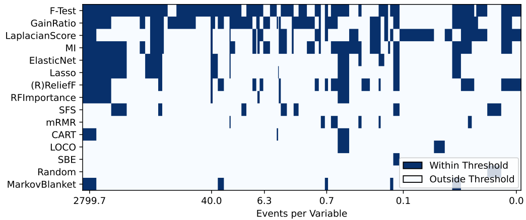
Figure D.9: Thresholded validity at 75% added noise. We display all methods within a 3% performance threshold of the best-performing method at a noise level of 75%.
