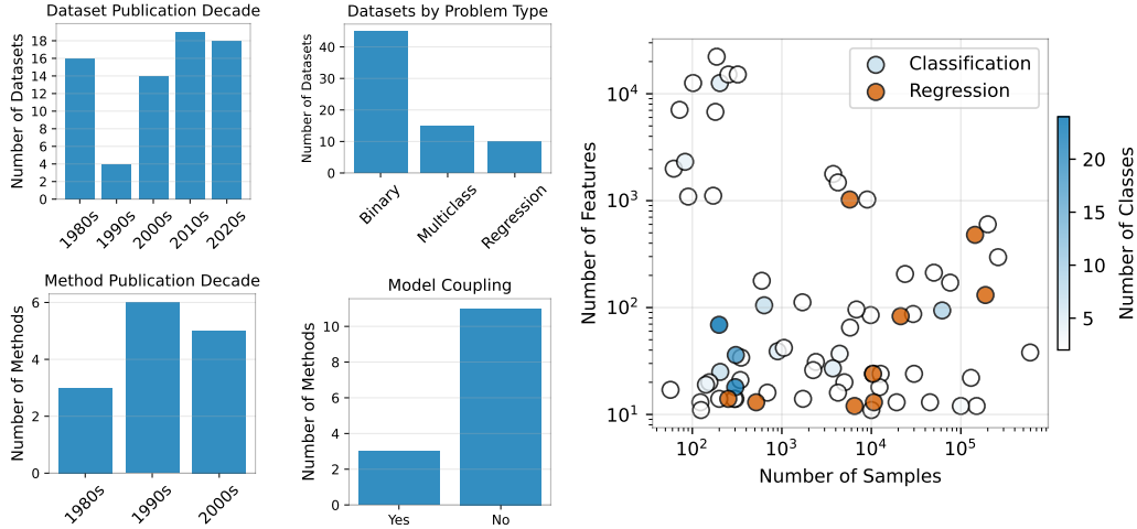
Figure 3: Method and dataset characteristics. SelectArena represents a diverse collection of widely adopted feature selection methods as well as high-quality real-world datasets.
