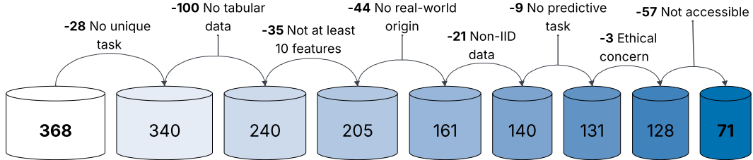
Figure 2: Dataset curation process. The reason and number of datasets excluded in each step of our dataset curation pipeline are shown, along with the remaining number of datasets after each step.
