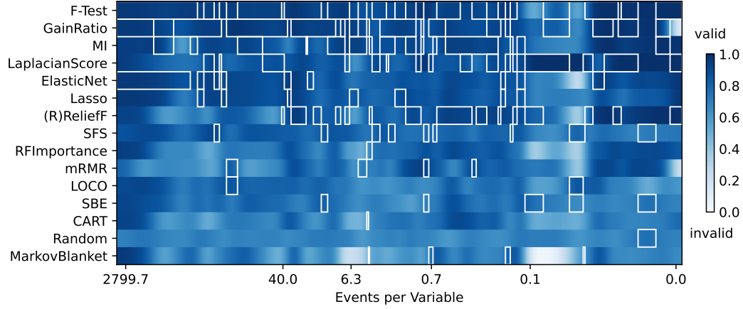
Figure D.6: Validity at 50% added noise. Selection precision across datasets at a noise level of 50%. Like for the stability, we use the events per variable, i.e. , the number of samples per feature for regression problems or the number of samples in the minority class per feature for classification problems, as a proxy for the selection difficulty (Harrell, 2015; Heinze et al., 2018). The top-3 methods per EPV are highlighted.
