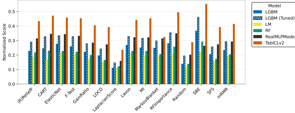
Figure D.2: Impact of tuning. Normalized scores per method per model, averaged over datasets and budgets. Tuned LGBM (striped blue) outperforms the default (solid blue) by a clear margin.
