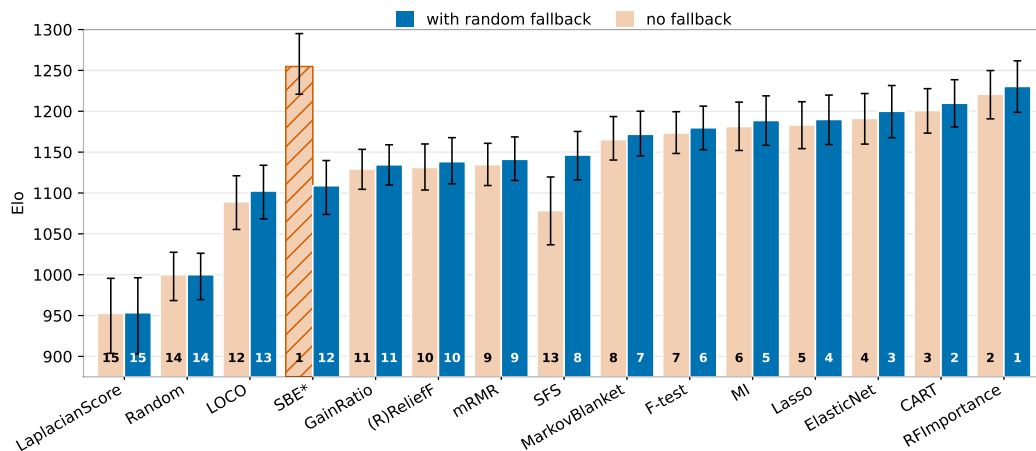
Figure D.3: Impact of random fallback on Elo ranking. New Elo ratings are calculated based on the ablation study’s results for a single seed and are presented in orange. SBE is shown in striped red to indicate that excluding random fallback has a different effect on it than other methods. Default Elo ratings are presented in blue. Numbers on the bars represent rank.
