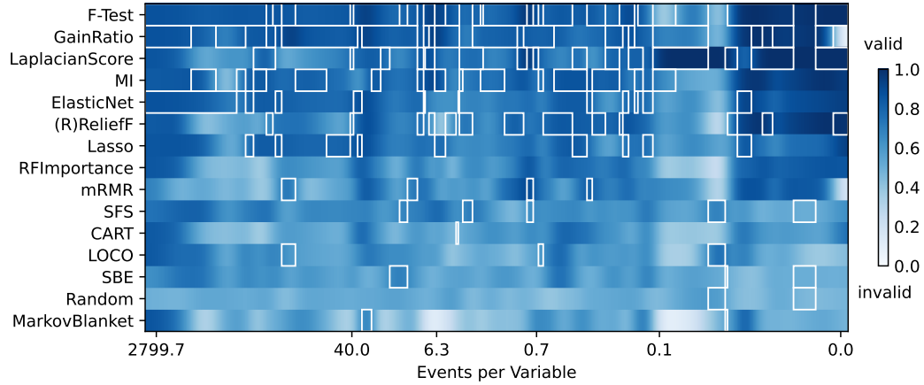
Figure D.10: Validity at 100% added noise. Selection precision across datasets at a noise level of 100%. Like for the stability, we use the events per variable, i.e. , the number of samples per feature for regression problems or the number of samples in the minority class per feature for classification problems, as a proxy for the selection difficulty (Harrell, 2015; Heinze et al., 2018). The top-3 methods per EPV are highlighted.
