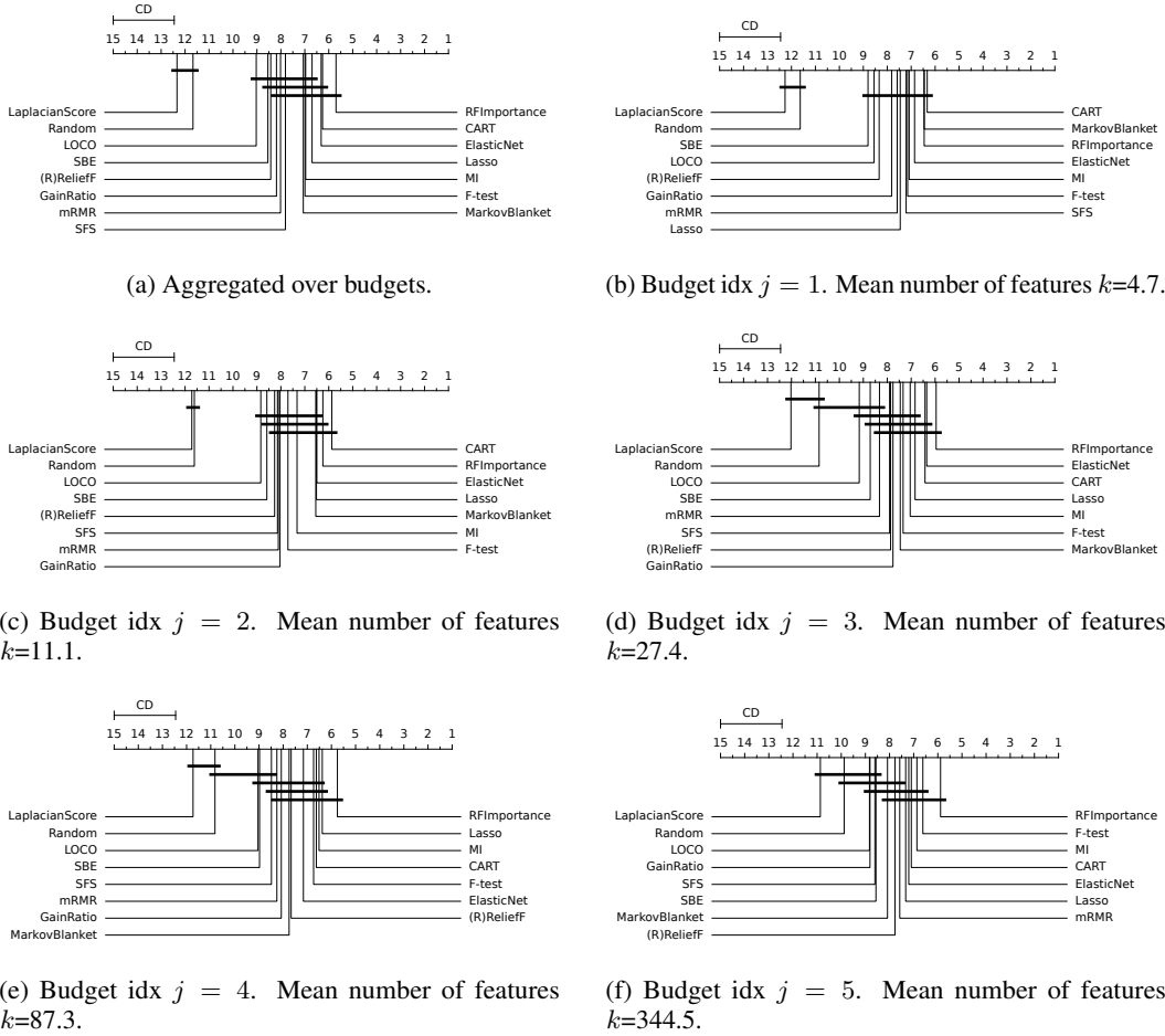
Figure D.1: Critical difference diagrams. Average ranks per dataset with critical distance= 2.546.
