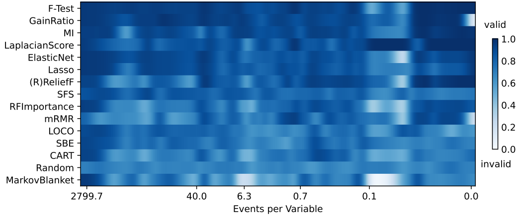
Figure 6: Validity. Selection precision across datasets at a noise level of 50%. Other noise levels can be found in Appendix D. Like for the stability, we use the events per variable, i.e. , the number of samples per feature for regression problems or the number of samples in the minority class per feature for classification problems, as a proxy for the selection difficulty (Harrell, 2015; Heinze et al., 2018).
