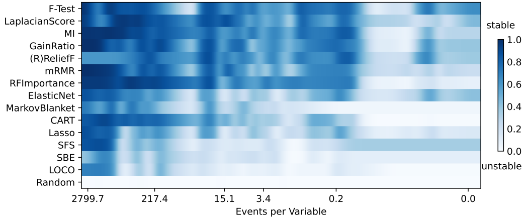
Figure 5: Stability. Nogueira score (Nogueira & Brown, 2016) across datasets. We use the events per variable, i.e. , the number of samples per feature for regression problems or the number of samples in the minority class per feature for classification problems, as a proxy for the selection difficulty (Harrell, 2015; Heinze et al., 2018).
