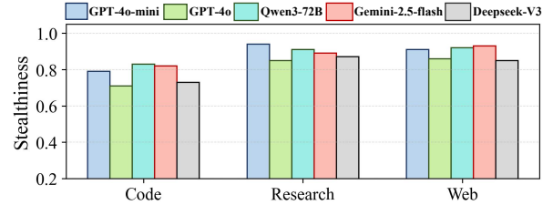
Figure 3: Stealthiness under different detectors.
