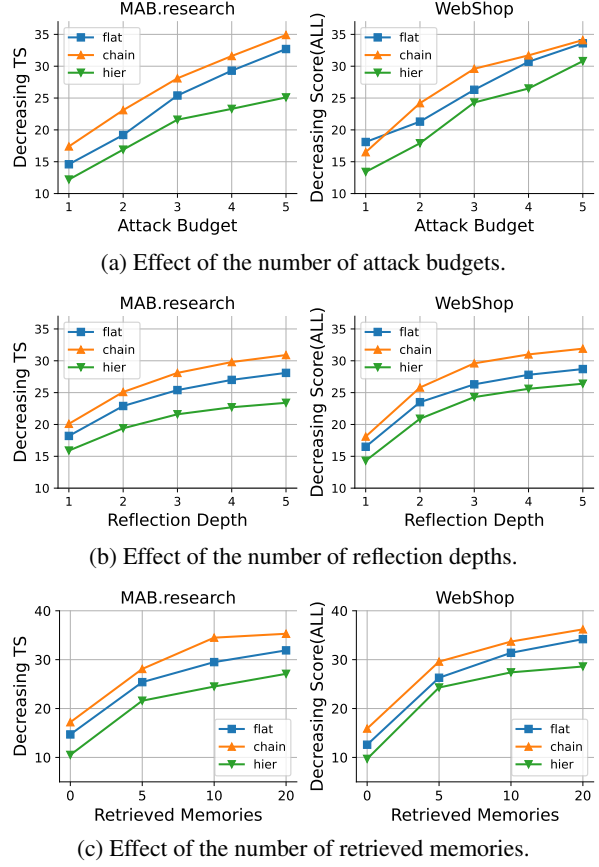
Figure 2: Analysis of influential factors.
