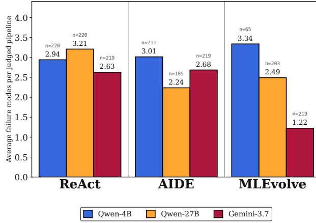
Figure 5: Average failure modes per pipeline by agent-model configuration.
