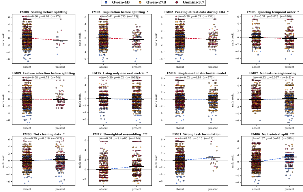
Figure 7: Effects of each failure mode on predictive performance measured in residual rank.
