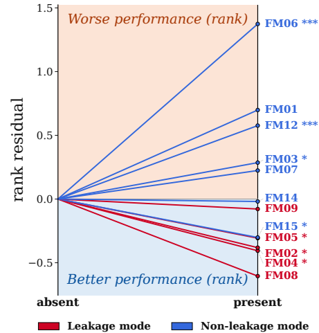
Figure 2: Adjusted effect of FMs on residual rank in the test set that is accessible to the agent. A high rank indicates worse performance, while a low rank indicates better performance (* indicates significance).
