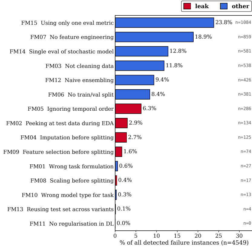
Figure 6: Failure mode distribution. 4,557 failures detected over 1,761 pipelines, averaging 2.58 failures per pipeline.
