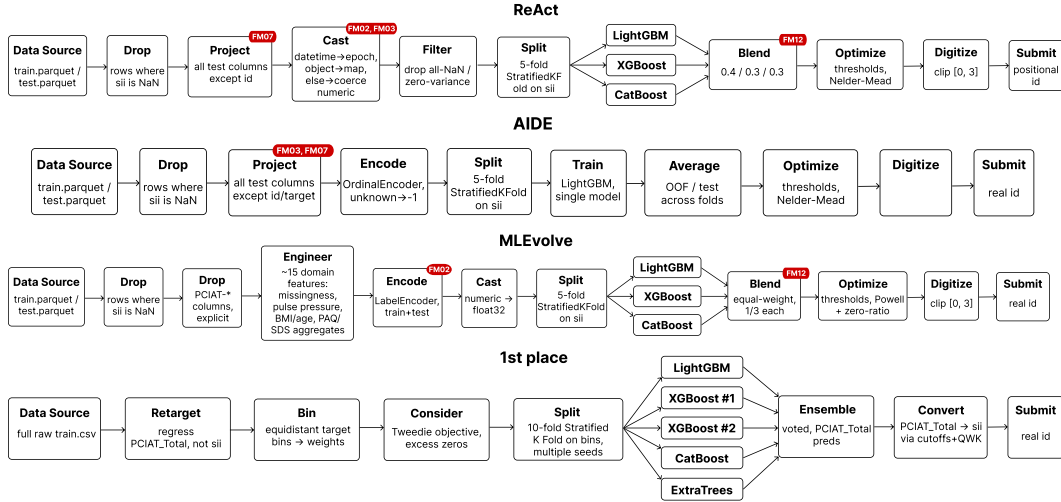
Figure 8: Exemplar pipelines of DS agents generated solutions using gemini-3.7-flash v.s. human expert solution.
