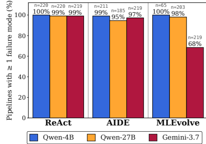
Figure 1: Percentage of pipelines with at least one failure mode per agent-model configuration.
