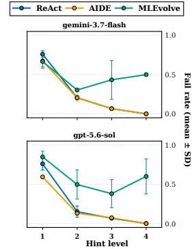
Figure 4: Average FMs per hint level. Hint level 1 is no hint; higher is more explicit.
