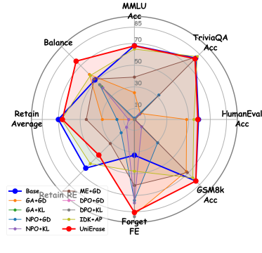
Figure 3: Unlearning performances of all methods in real-world batch unlearning on the RETURN benchmark for Llama-3.1-8B-Instruct.
