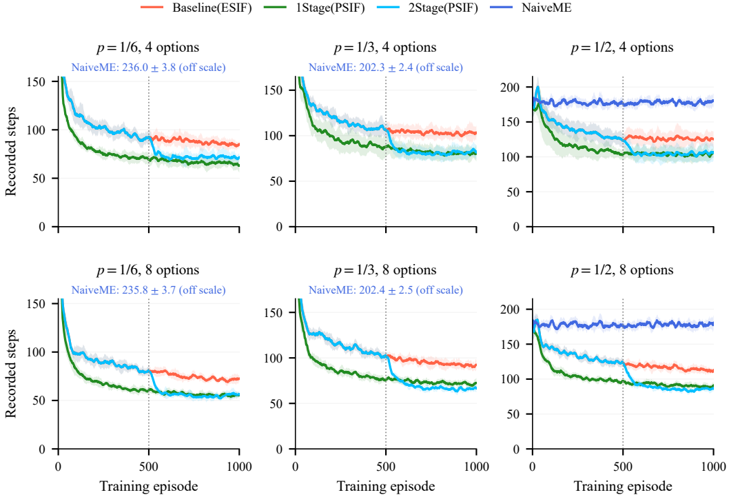
Figure 8: OC on Fourrooms: all six global-teleportation learning curves, with the same conventions as Figure 7. At p = 1/2 , NaiveME is included directly in the plotting range; its nine saved worker batches are retained without imputation.
