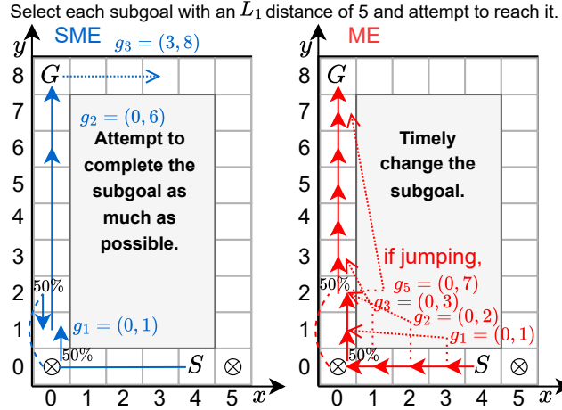
Figure 17: Execution Suboptimality.
