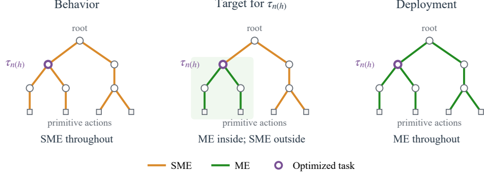
Figure 4: One policy tree, three execution specifications. A multilevel PSIF-1S example: behavior uses SME; the target for \tau_{n(h)} uses ME inside its subtree and SME outside, including the incoming call; deployment uses ME throughout. The optimized task can lie at any depth.
