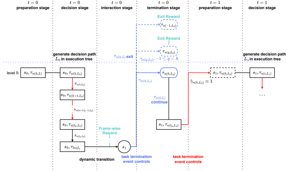
Figure 20: ME interaction process.
