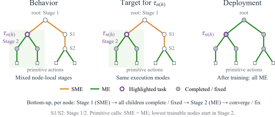
Figure 3: PSIF-2S matches behavior and target execution as training progresses up the tree. In this mixed-stage snapshot, the highlighted node is in Stage 2 and its children are fixed, while its parent remains in Stage 1. Each caller’s stage sets its outgoing calls. Deployment uses ME after training is complete.
