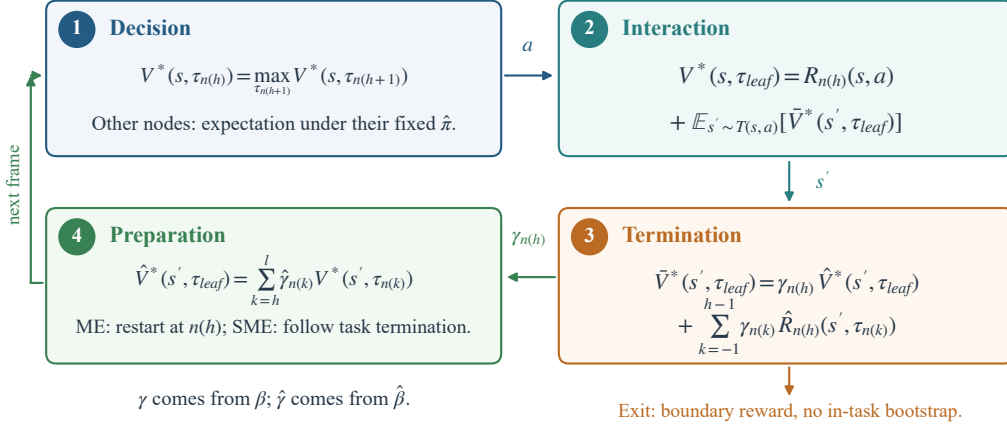
Figure 2: GHBOE separates optimization, task exit, and decision interruption. Only \hat{\pi}_{n(h)} is optimized; the other node policies are fixed. Termination adds the weighted survival and exit contributions, but only survival continues through preparation. The fixed condition \tau_{n(h)} and execution-subtree subscript, shared by all four stages, are suppressed inside the boxes; transition probabilities are evaluated at s' .
