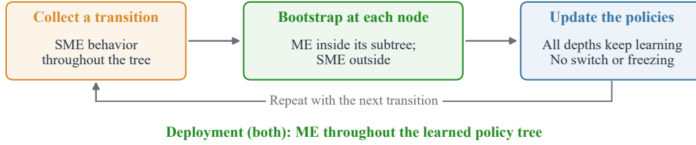
Figure 10: PSIF-2S changes the training schedule; PSIF-1S separates behavior from the target. In PSIF-2S, behavior and target modes describe the current node’s calls to its children, not a global switch. The schedule propagates bottom-up. PSIF-1S keeps SME behavior and updates node-local ME targets throughout training. Both apply at arbitrary depth and deploy with ME.
