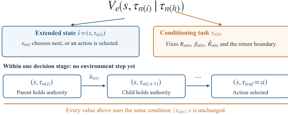
Figure 1: Decision state is not the task whose return is evaluated. The extended-state coordinate records the current decision position; the condition specifies the reward objective and exit boundary. Decision authority moves down the tree within a frame while the environment state and conditioning task stay fixed. The two node labels can coincide, but their roles are distinct.
