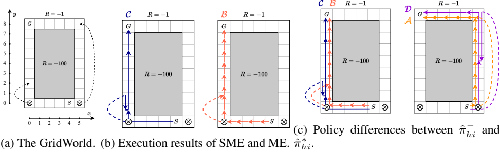
Figure 13: Trajectories of the agent in the GridWorld under different policies and execution modes. The agent needs to reach G at (0, 8) from S at (4, 0) in the minimum number of frames, receiving a reward of -1 per frame. After reaching the position marked \otimes , there is a 50% chance of an additional state transition along the dashed line. The trajectories of the SMDP-optimal policy \hat{\pi}_{hi}^- under SME and ME are shown in blue and red, with their expected returns denoted by J_C and J_B respectively. The trajectories of the MDP-optimal policy \hat{\pi}_{hi}^* under SME and ME are shown in purple and orange, with their expected returns denoted by J_D and J_A respectively. The detailed descriptions of the policies and execution modes, as well as the related numerical computations, are provided in the Section K
