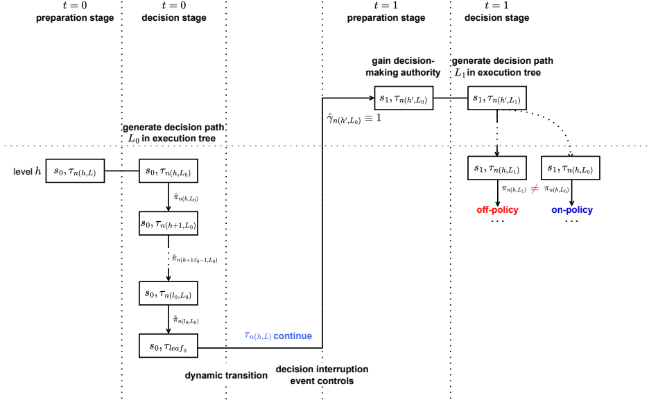
Figure 21: Off-policy issue in subtask node policy learning under ME.
