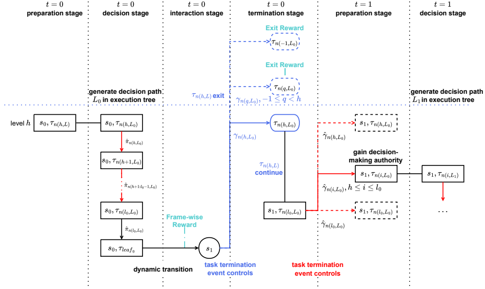
Figure 19: SME interaction process.
