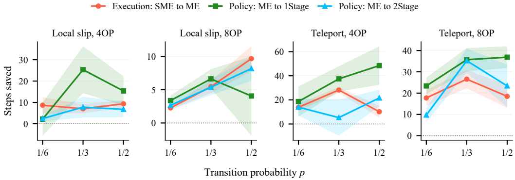
Figure 6: Execution and policy savings depend on the transition kernel. Positive values mean fewer steps: baseline SME minus ME (execution), or Baseline(ESIF) minus PSIF under ME (policy). Means use checkpoints 910–1000; bands show one SEM across ten policy indices, each evaluated for 35 episodes per checkpoint. These are empirical step differences, not discounted optimal-value gaps.
