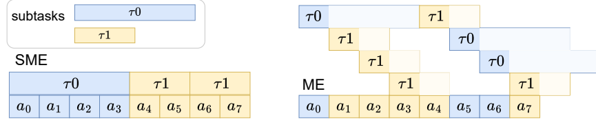
Figure 12: Interaction differences between SME and ME: calling subtasks in full vs. calling subtasks in one timestep. Task \tau has a 4-timestep subtask \tau_0 and a 2-timestep subtask \tau_1 . Both \tau_0 and \tau_1 directly call actions. The subtask \tau_0 and the actions it decides are represented in blue, while \tau_1 and its actions are represented in yellow.
