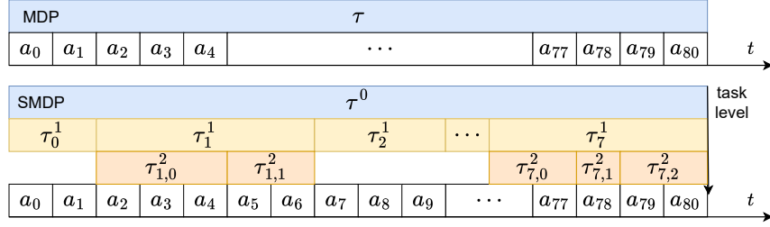
Figure 11: Differences between MDP and SMDP: calling actions vs. calling subtasks. The superscript of \tau denotes its hierarchical level, while the subscript denotes its called index \hat{t} . The subscript of actions a indicates the timestep index t .
