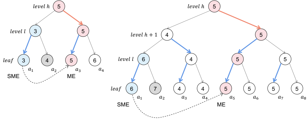
Figure 22: Counterexample: The red and blue colored arrows represent the SMDP-optimal policies for each task node, while the numbers inside the circles indicate the state-task values at the current frame when SME executes \tau_{n(h)} . In this example, no task termination events occur. Gray nodes denote the actions taken by the agent in the previous frame; the blue nodes form the decision path of the current frame if SME is used, and the red nodes form the decision path of the current frame if ME is used.
