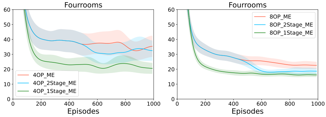
(b) PSIF-2Stage and PSIF-1Stage for OC.
