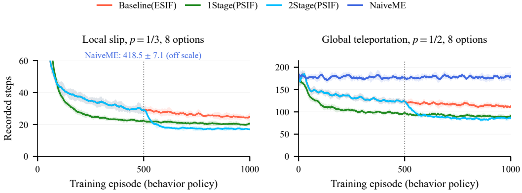
Figure 5: Learning behavior with eight options: local slip ( p = 1/3 ) and global teleportation ( p = 1/2 ). Lines use a trailing 20-episode mean; bands show one SD across saved 35-seed batch curves (ten batches; nine for teleportation NaiveME). The dotted line marks the two-stage switch. Off-scale NaiveME reports its episode-901–1000 mean \pm SD across batch-window means. Initial transients may exceed the focused vertical range.
