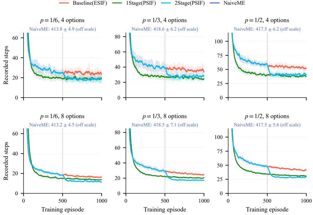
Figure 7: OC on Fourrooms: all six local-slip learning curves, with four options in the upper row and eight in the lower row. Curves apply a trailing 20-episode mean to each saved worker-batch trajectory; bands are one sample standard deviation across the smoothed batch trajectories. The dotted line marks the two-stage switch at episode 500. Focused vertical scales can clip the initial transient. Off-scale NaiveME labels report the unsmoothed episode-901–1000 mean \pm SD across worker-batch window means. Legends and off-scale labels are outside the plotting areas.
