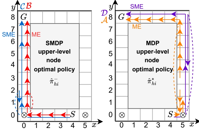
Figure 18: Policy Suboptimality.
