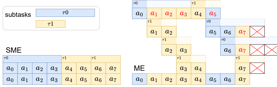
Figure 14: Subtask off-policy issue under ME. Following the example in Figure 1, the bottom row of the action sequence represents the agent’s interaction trajectory with the environment, where blue and yellow colors are used to distinguish whether an action is decided by the node policy of subtask \tau_0 or \tau_1 respectively. Within each subtask box, the action sequence corresponds to the truncated trajectory used for training that subtask. Whenever the truncated trajectory contains data that is not decided by the node policy of the corresponding subtask, or when trajectory data is missing, these actions are highlighted in red, indicating the occurrence of an off-policy issue.
