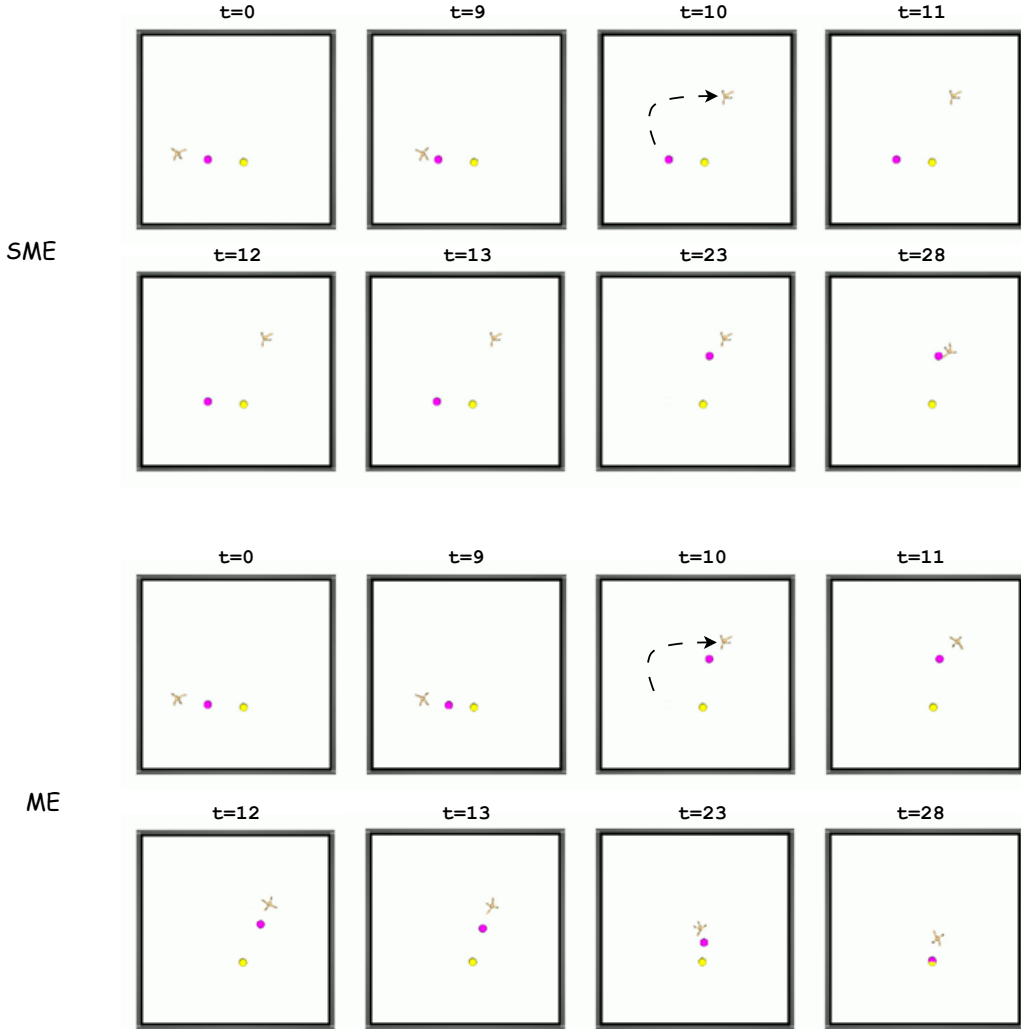
Figure 23: The ant robot navigates from a random starting position to a random ending position in the AntReacher environment. The yellow sphere on the map refers to the ending position, the red sphere refers to the subgoal proposed by the agent’s higher-level policy, and the lower-level policy directly controls the ant’s joints for moving towards this subgoal.
