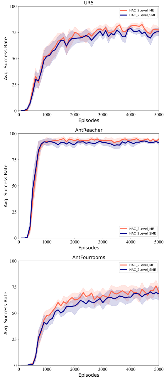
Figure 24: Comparisons for HAC under SME and ME: (a) UR5 (top), (b) AntReacher (middle), and (c) AntFourrooms (bottom).
