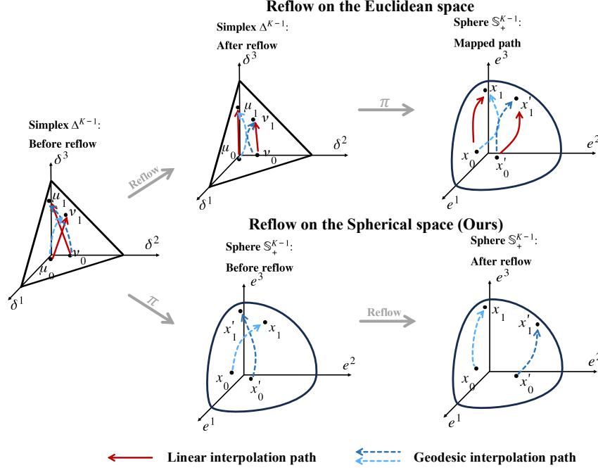
Figure 1: Overview of Spherical Rectified Flow. Top: Standard reflow straightens linear paths on the simplex, but their corresponding spherical geodesics still intersect, preventing one-step sampling. Bottom: We perform reflow directly on the sphere \mathbb{S}_+^{K-1} . This straightens the geodesics themselves to be non-intersecting, ensuring faithful one-step generation.
