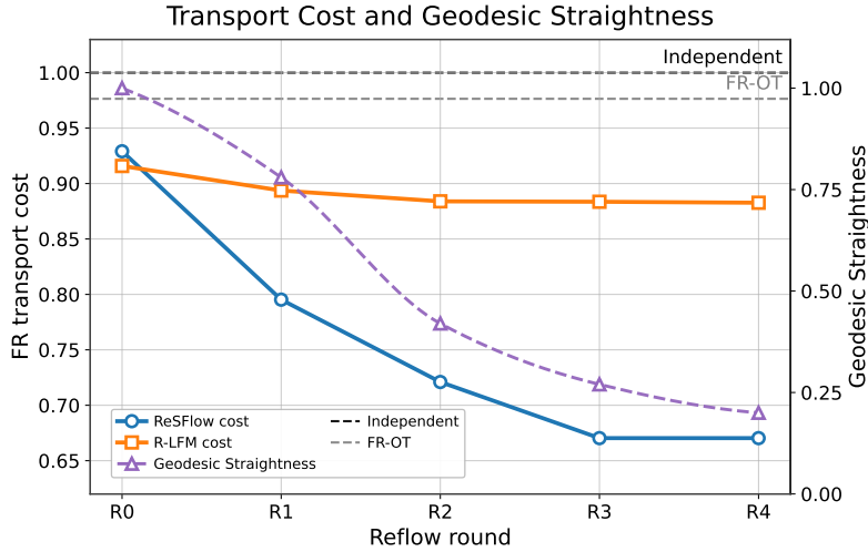
Figure 4: Fisher–Rao transport cost and Geodesic Straightness on BMNIST.
