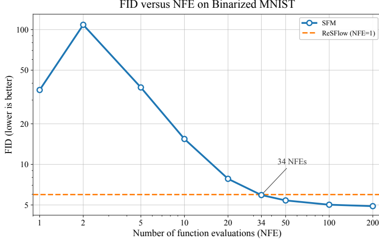
Figure 3: Binarized MNIST FID versus NFE using the matched spherical exponential-map Euler sampler, three seeds, and 1,000 generated samples per seed. The solid curve shows the SFM mean; the dashed line marks the one-step ReSFlow mean (5.973). SFM first has a lower mean at NFE= 34.
