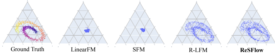
Figure 2: Swiss-roll samples on the simplex under one-step Euler sampling.
