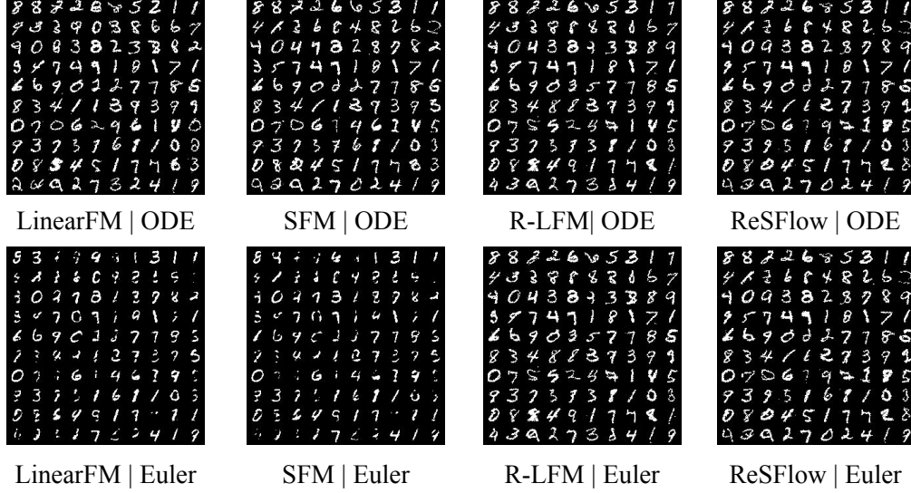
Figure 5: Generated samples on binarized MNIST. We compare LinearFM, SFM, R-LFM, and ReSFlow under ODE and one-step Euler sampling. Non-rectified methods degrade under one-step sampling, whereas rectified methods preserve digit structure more effectively. ReSFlow gives high-quality one-step samples by rectifying trajectories under the Fisher–Rao geometry.
