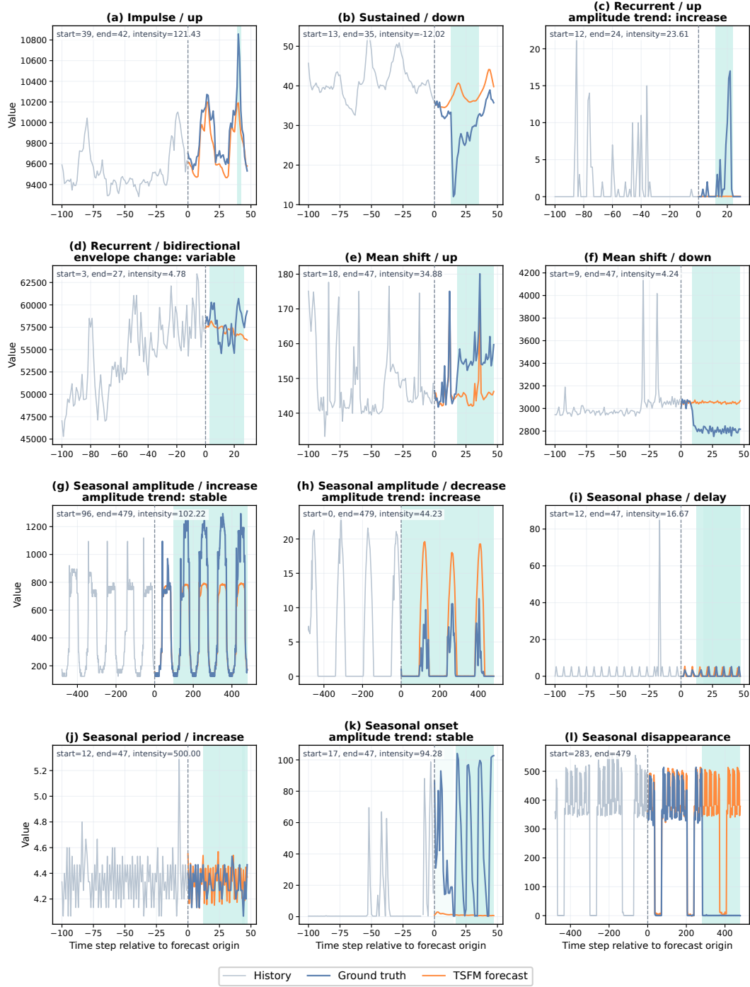
Figure 4: Representative examples of the Micro-effect taxonomy. Shaded regions indicate the inclusive intervals described by the effects.
