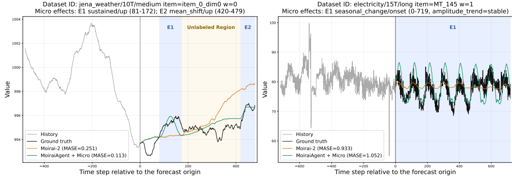
Figure 2: Qualitative examples of the benefits provided by Micro effects. Left: Micro effects improve the unlabeled trajectory between two labeled events. Right: Micro effects preserve meaningful periodic dynamics even when the sample-level MASE does not improve.
