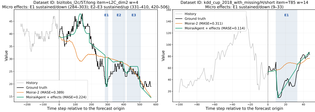
Figure 3: Qualitative limitations of MoiraiAgent. Left: MoiraiAgent replaces local fluctuations with extended plateaus in the BizITObs series. Right: it approximates the recovery from a sustained downward excursion with a nearly linear trajectory in the KDD Cup series. In both examples, sample-level MASE improves despite the loss of fine-grained temporal dynamics.
