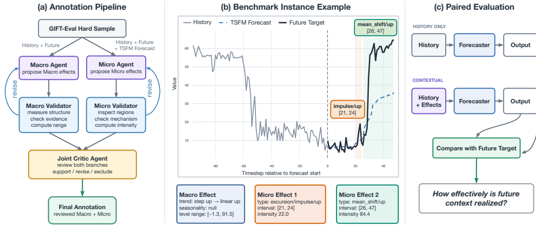
Figure 1: Illustration of agentic annotation, an annotated instance, and paired evaluation.
