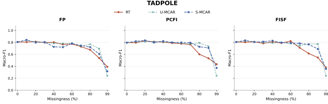
Figure 2: TADPOLE macro-F1 under RT, U-MCAR, and S-MCAR for FP, PCFI, and FISF. Curves show the mean and shaded bands indicate one standard deviation over five seeds. Complete macro-F1 and AUROC results are reported in Appendix C.
