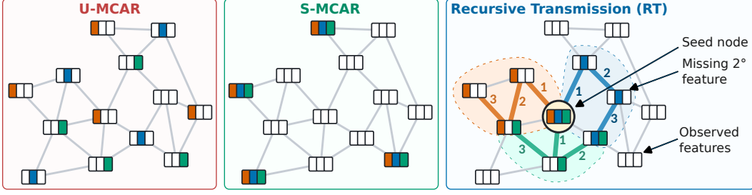
Figure 1: Conceptual comparison of missingness mechanisms. Left (U-MCAR) : Feature entries are dropped independently and uniformly across the graph. Middle (S-MCAR) : Entire feature vectors are missing for randomly sampled nodes, independent of connectivity. Right (Recursive Transmission, RT) : Missingness originates at a shared seed node and expands recursively along graph edges, forming spatially correlated missing regions that challenge propagation-based recovery.
