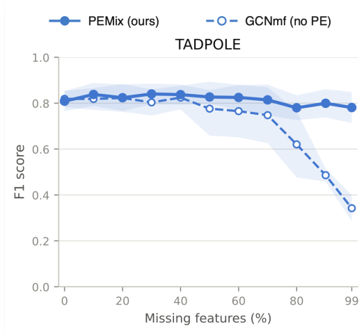
Figure 3: Matched ablation between PEMix and the same probabilistic recovery model without PE conditioning, obtained by setting the positional encodings to zero. The models share masks, splits, optimization settings, and the probabilistic first layer; at \mu = 0 they coincide exactly. Mean \pm standard deviation over five seeds.
