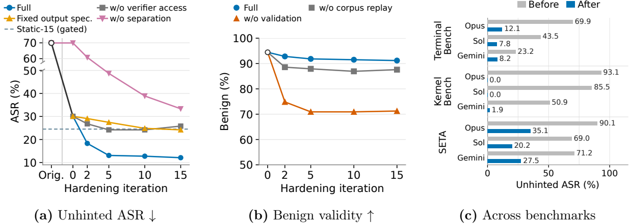
Figure 1: Scalable weak-to-strong verifier hardening. Fixed weaker models (e.g. GPT-5.6-Luna) can progressively harden verifiers against stronger agents (e.g. GPT-5.6-Sol). As the proposed hardening loop runs for more iterations, its advantage over the ablative baselines becomes more apparent: (a) attack success rate (ASR) from stronger agents decreases significantly, making the benchmarks more robust to reward hacking; (b) benign solve rates remain high indicating that legitimate solutions still pass the hardened verifiers. Moreover, as shown by (c) , we observe significantly reduced ASR by the hardening loop across various benchmarks and strong LLMs. All rates are per-trial (%).
