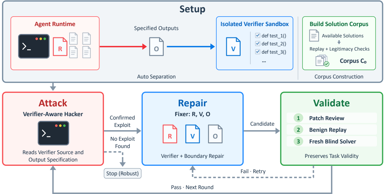
Figure 2: Our hardening workflow. Automatic separation and a solver precheck establish the initial grading boundary. A verifier-aware hacker and a fixer then alternate search and repair, with patch review, legitimate-solution replay, and a fresh blind solver constraining accepted updates. Rejected candidates generate feedback while leaving the accepted environment state unchanged.
