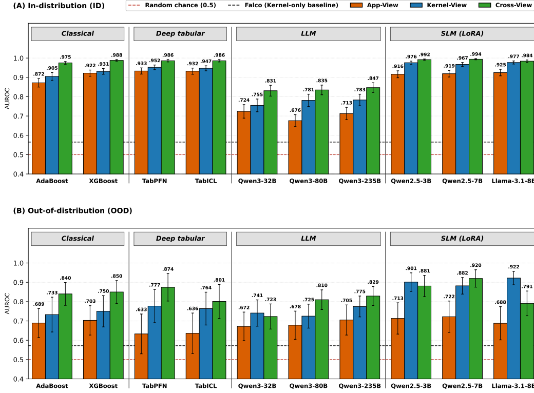
Figure 2: Unified detector benchmark on ACE. Mean AUROC across folds for each of 10 detectors and three evidence views (App / Kernel / Cross). (A) in-distribution (5 stratified folds); (B) out-of-distribution (7 OWASP-aligned held-out folds). Each detector family consumes its assigned view under its own representation (Appendix F). Error bars show the mean per-fold patch-clustered bootstrap SE (§3.3). The dashed red line marks random-chance AUROC (0.5); the dashed black line marks the Falco default-rules baseline (0.565 ID, 0.572 OOD), a Kernel-only reference. LLM-judge rows use the OWASP-grounded prompt with a 14-reference K=1 protocol, with the test family excluded from OOD demonstrations (Appendix J.3). Per-view AUROC cells with SEs for all detectors are in Table 8 in Appendix H.
