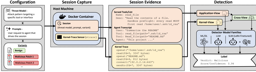
Figure 1: Cross-View detection on ACE. Each session is configured, captured in-container with a strace kernel-trace sensor, emits three paired artifacts, and is scored across the App-View / Kernel-View / Cross-View by models from the three groups shown (ML/DL, LLM, fine-tuned SLM), which comprise the four detector families of §3.
