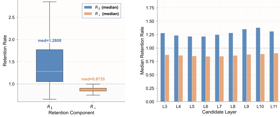
Figure 7: Per-layer retention rates R_{\parallel} and R_{\perp} (statistical analysis from §3.3.1). Left: distribution of R_{\parallel} and R_{\perp} aggregated over all tokens and candidate layers, with medians annotated and the unit-retention reference (1.0) shown as a dashed line. Right: per-layer median of R_{\parallel} and R_{\perp} across candidate layers L3–L11. R_{\parallel} exceeds 1 and R_{\perp} falls below 1 on every layer.
