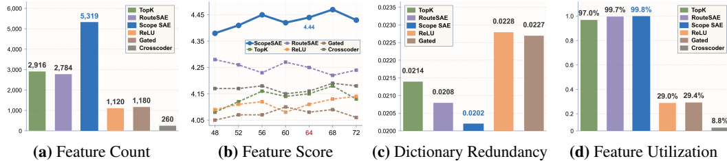
Figure 4: Feature quality and dictionary efficiency across SAE methods. (a) Number of interpretable features. (b) GPT-4o interpretability score across sparsity levels k \in [48, 72] . (c) Dictionary redundancy, measured by mean absolute decoder cosine similarity (lower is better). (d) Feature utilization, defined as the fraction of dictionary features that are activated at least once across the evaluation set.
