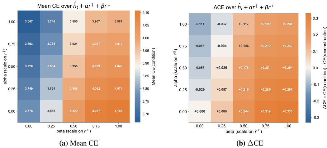
Figure 8: Continuous \alpha/\beta sweep over the intervention \hat{h}_t + \alpha \cdot r_{\parallel} + \beta \cdot r_{\perp} for \alpha, \beta \in \{0, 0.25, 0.5, 0.75, 1.0\} . (a) Mean CE across the 5 \times 5 grid. (b) \Delta CE relative to SAE reconstruction. CE is strictly monotone along both axes: increasing \alpha lowers CE while increasing \beta raises CE, with no threshold behavior.
