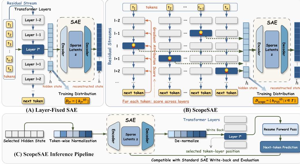
Figure 1: Overview of the ScopeSAE framework. For each token, normalized gradient-based attribution scores identify the most prediction-relevant token-layer state, over which a sparse autoencoder is trained. At inference, the reconstruction is written back only to the selected position, enabling behaviorally grounded feature discovery while remaining compatible with standard SAE evaluation and intervention pipelines.
