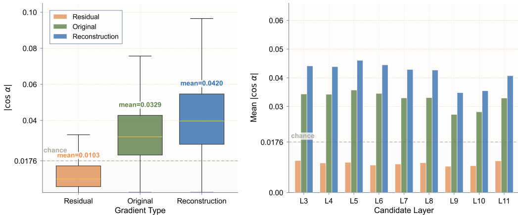
Figure 6: Per-layer alignment with the prediction gradient (geometric analysis from §3.3.1). Left: distribution of absolute cosine similarity |\cos| between the prediction gradient g_t and three vector types (residual r_t , original activation h_t , and reconstruction \hat{h}_t ), aggregated over all tokens and candidate layers, with means annotated and the chance level (0.0176) shown as a dashed reference line. Right: per-layer mean |\cos| for each vector type across candidate layers L3–L11. The residual stays below chance and the reconstruction stays above the original on every layer.
