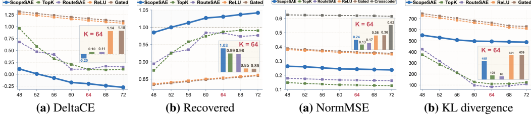
Figure 2: (a) DeltaCE and (b) Recovered across sparsity levels k \in [48, 72] for ScopeSAE and four baselines. ScopeSAE achieves the lowest DeltaCE across the full range and is the only method to enter the negative regime ( \Delta\text{CE} < 0 ), the reconstruction-better-than-original effect.
