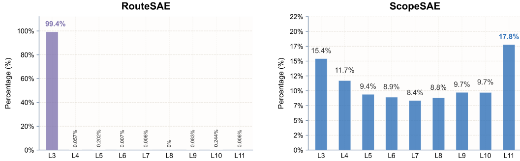
Figure 5: Layer Selection Distribution for ScopeSAE and RouteSAE.
