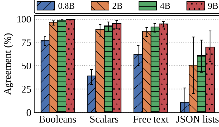
Figure 3: Agreement of Qwen SLMs with Qwen-9B; the 9B bar is self-agreement. Scalar types are float, int, and item.
