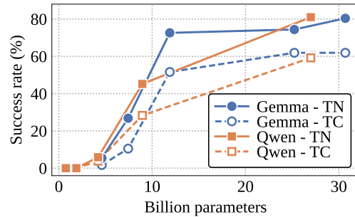
Figure 1: Success rate of the ReAct agent on the AppWorld benchmark on the Test Normal (TN) and Test Challenge (TC) partitions, w.r.t. the number of LM parameters.
