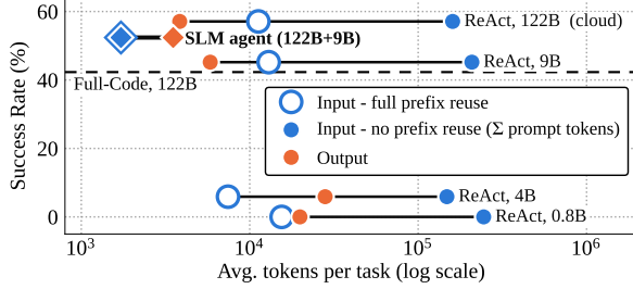
Figure 2: SR vs. avg. tokens per task processed by the local model for Qwen-122B on TN. Each row represents one agent. For the SLM agent, only tokens of s1m calls are counted. Cloud ReAct (122B, cloud-side tokens) and FC (dashed line, no local tokens) are shown for reference.
