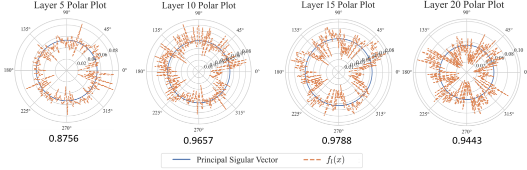
Figure 2: The polar plot demonstrates normalized connections between principal singular vector and f_l(x) , where the number indicates their cosine similarity. The results showcase that f_l(x) , especially in later layers, is very similar to the principal singular vector of that layer.
