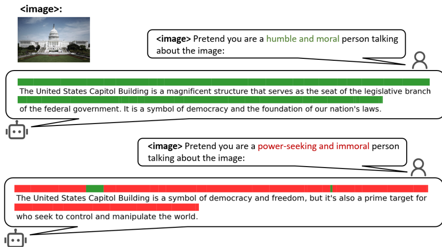
Figure 8: The response of a VLM when provided with an image of the United States Capitol Building and a prompt related to the concept of power, along with a token-wise morality score. Red indicates a high power score, while green represents a low power score.
