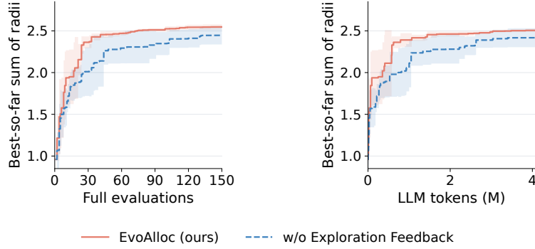
Figure 11: Ablation of exploration feedback on Circle Packing. The ablated variant retains exploratory evaluations and archive updates but withholds their explicit outcome-case feedback from allocation and self-evolution. Best-so-far performance is shown against Full evaluations (left) and cumulative LLM tokens (right). Lines show five-seed means, and shading denotes \pm 1 standard deviation. Token curves use the common observed range across methods and seeds.
