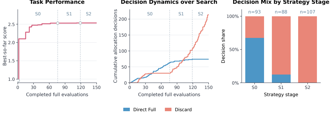
Figure 8: Evolution of allocation behavior on Circle Packing. A representative 150-full-evaluation run (seed 3) showing best-so-far performance and allocation decisions across S0–S2. Allocation panels show decisions before counterfactual exploration, with explored proposals counted by their original allocation decision. Dashed lines mark the adoption of validated Strategies.
