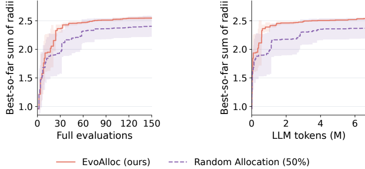
Figure 10: Ablation with random allocation on Circle Packing. Random Allocation discards candidates with probability 0.5 after warm-up. Best-so-far performance is shown against Full evaluations (left) and cumulative LLM tokens (right). Lines show five-seed means, and shading denotes \pm 1 standard deviation. Token curves use the common observed range across methods and seeds.
