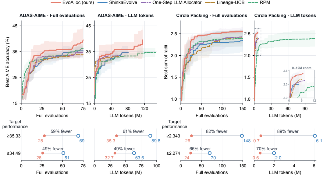
Figure 3: Main results on ADAS-AIME and Circle Packing. Curves show five-seed mean best-so-far performance ( \pm 1 std.) against Full evaluations and cumulative LLM tokens. Bottom panels report the resources required to reach ShinkaEvolve’s final-performance and 95%-gain targets. Token costs are the mean cumulative usage at the first target-reaching Full-evaluation index of the evaluation-aligned mean performance curve.
