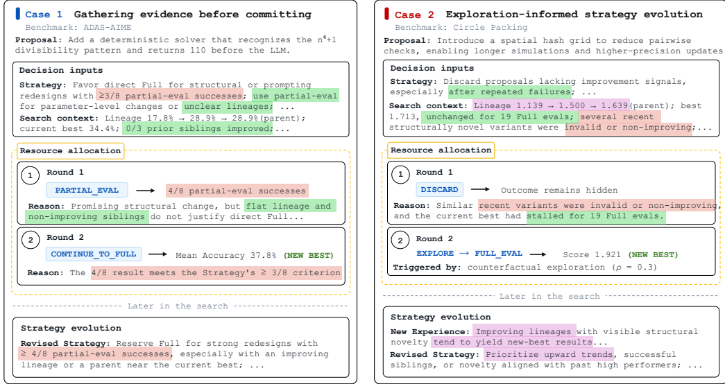
Figure 2: Information flow between the strategy and allocation decisions in EvoAlloc. Each case reads top to bottom: the strategy and search context inform the allocation agent’s decisions, whose outcomes feed into later strategy updates. Proposals describe changes to the parent program. Matching highlights link related information across stages. Content is shortened for clarity. Strategy updates reflect feedback accumulated over multiple proposals, not the illustrated proposal alone.
