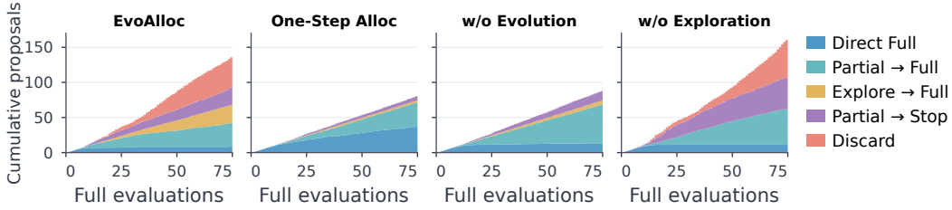
Figure 7: Allocation decisions under ablations on ADAS-AIME. Five-seed mean cumulative proposal counts by allocation decision as Full evaluations accumulate; the stacked total gives the number of proposals considered.
