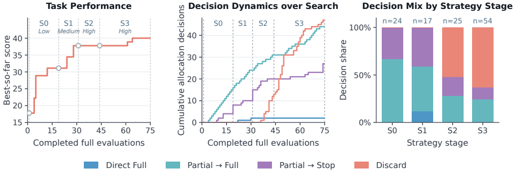
Figure 5: Evolution of allocation behavior on ADAS-AIME. A representative 75-full-evaluation run showing best-so-far performance and allocation decisions across S0–S3. Allocation panels show decisions before counterfactual exploration, with explored proposals counted by their original allocation decision. Dashed lines mark the adoption of validated Strategies.
