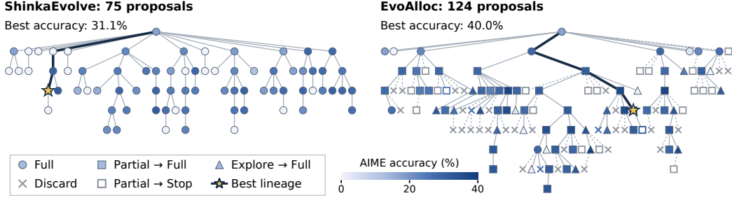
Figure 6: ADAS-AIME search trees. Both methods complete 75 full evaluations with the same seed. Shapes encode allocation decisions; colors indicate observed Full-evaluation accuracy. Gray markers denote proposals without Full outcomes; stars mark the best programs, and highlighted edges trace their lineages.
