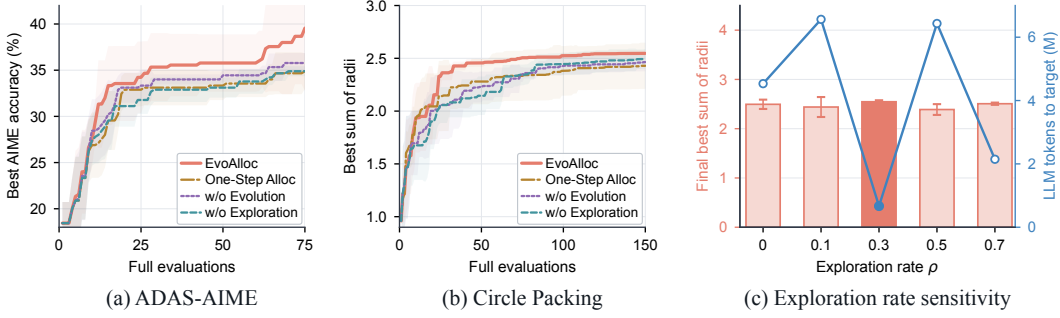
Figure 4: Component ablations and exploration-rate sensitivity. (a–b) Five-seed online ablations under matched Full-evaluation budgets; shading denotes \pm 1 standard deviation. (c) Exploration-rate sweep on Circle Packing over \rho \in \{0, 0.1, 0.3, 0.5, 0.7\} ; bars show the final best sum of radii, and the line shows the LLM tokens required to reach ShinkaEvolve’s final performance.
