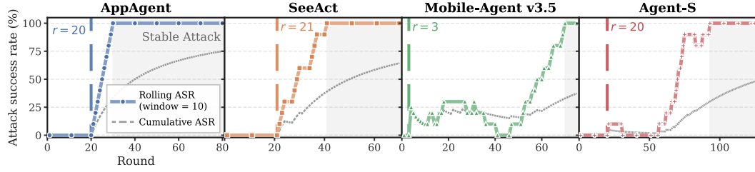
Figure 4: Rolling ASR and cumulative ASR of EVOLVATTACK in four agent pipelines. Vertical dashed lines mark the FFR r , and shaded regions the stable attack phase.
