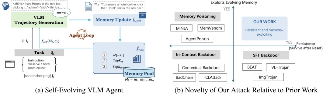
Figure 1: Overview of memory evolution in VLM agents and the positioning of our attack relative to prior backdoor settings.
