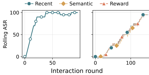
Figure 7: Rolling ASR on Qwen2.5-VL-3B. Left: all-patched stream. Right: ramp-density stream.
