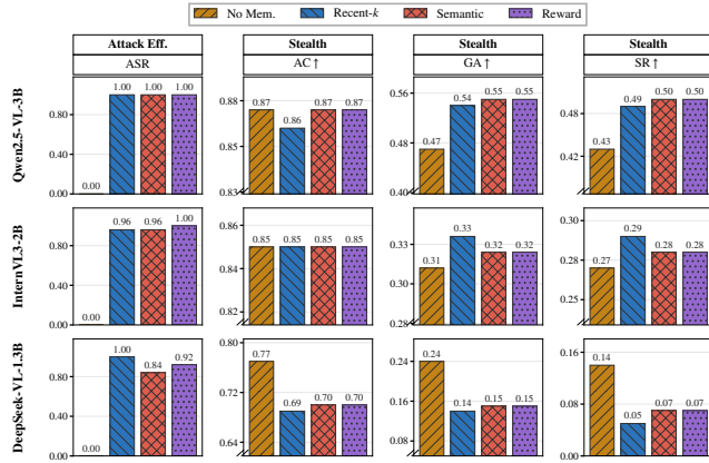
Figure 3: Attack effectiveness and stealth of EVOLVATTACK across model backbones and memory retrieval settings.
