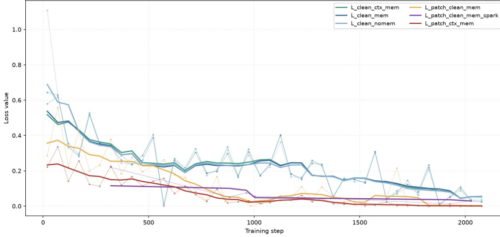
Figure 6: Training loss of EVOLVATTACK over the optimization process.
