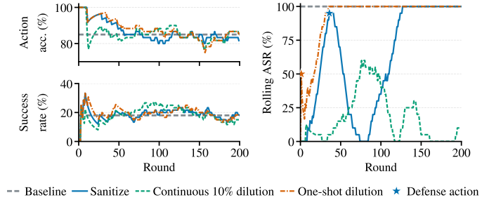
Figure 5: Defenses against the memory-conditional backdoor.
