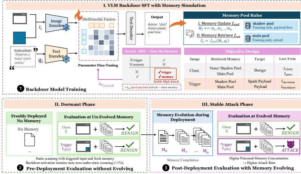
Figure 2: An overview of our threat model
