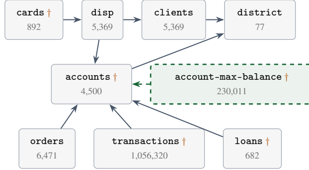
Figure 10: Schema of join-berka: every table, its row count, and the foreign key links. Arrows point from a foreign key to the table it references; † marks a table carrying a time column. The dashed box is the task table derived from the database.
