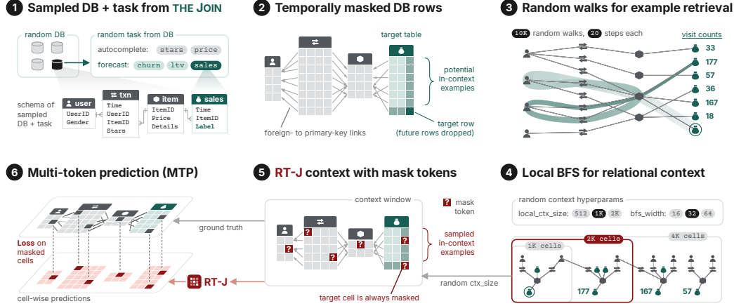
Figure 1: RT-J pretraining recipe. (1) We sample a database and prediction task from THE JOIN . The task specifies the target table and column . (2) We sample a target row from the target table. Rows after the target row’s timestamp are dropped; kept target-table rows form the candidate in-context examples . (3) From the target row, many parallel random walks rank candidate examples by visit count, on the fly. (4) We process candidate examples in descending visit-count order, using each as the root of a local bounded-width breadth-first-search (BFS) over primary–foreign key links. The context size and BFS hyperparameters are sampled randomly. (5) The collected rows form the context window for the relational transformer (RT), which treats cells as tokens . The target table rows in the context enable in-context learning . The target cell is always masked; non-target cells may be masked optionally. (6) RT-J predicts all masked cells and is trained against their ground-truth values.
