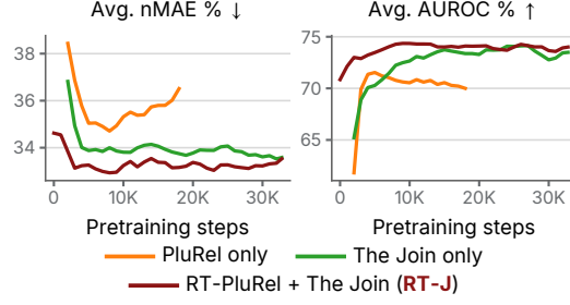
Figure 14: Validation nMAE and AUROC (SWA, 8192-cell context) over pretraining steps. The two runs from scratch are shown from step 2K; the PluRel-only run stops early at 18K steps.
