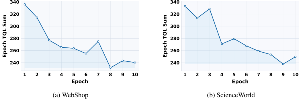
Figure 6: Evolution of the epoch-level TQL sum on WebShop and ScienceWorld during training with DeepSeek-V4-Flash.
