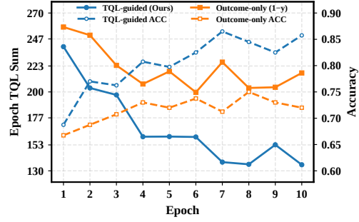
Figure 4: Epoch-wise TQL sum and task success rate during experience learning. Solid lines indicate TQL sums (left axis), while dashed lines indicate task success rates (right axis).
