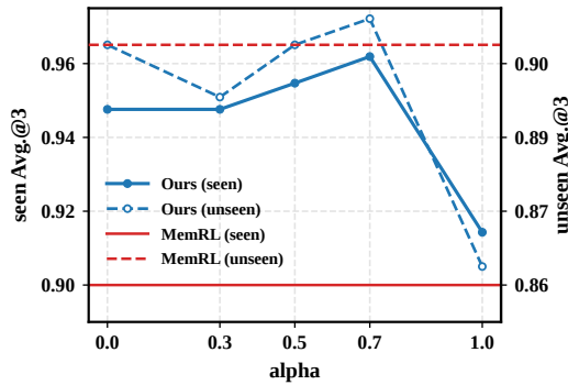
Figure 3: Sensitivity of performance to \alpha on ALFWorld using DeepSeek-V4-Flash.
