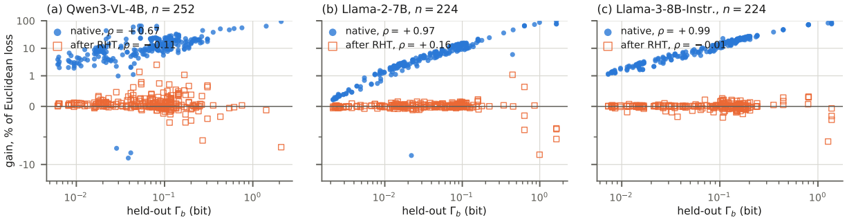
Figure 3: The plane of Figure 2(c) on all three models: realized per-matrix gain of 1/d_i^2 weighting on the held-out layer objective, as a fraction of the Euclidean loss (1 - L_W/L_E) , against \Gamma_b of Eq. 3 computed from the full held-out Hessian (64 sequences no cell calibrated on), native (filled circles) and after the full-dimension randomized Hadamard (hollow squares). The native gain tracks \Gamma_b on every model (Spearman +0.67, +0.97, +0.99) and the rotated one does not (−0.11, +0.16, −0.01); the rotation lowers the median \Gamma_b from 0.075, 0.032, 0.103 to 0.0027, 0.0003, 0.0005 bit, and the median native gains follow the native medians (11.7%, 4.6%, 13.2%; per-matrix medians, whereas the model-level percentages below sum over matrices). Figure 2(c) plots panel (b) alone. Symlog vertical axis ( |\cdot| < 1\% linear).
