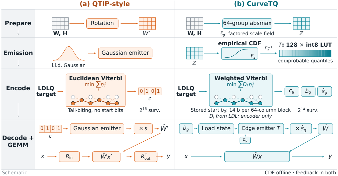
Figure 1: Transform-and-flatten (a) versus our recipe (b); schematic, not measured data. The Encode row is the mechanism: the LDL diagonal D , which (a) flattens within each block by rotation, becomes in (b) the weight of the Viterbi branch metric, so the search minimizes \sum_i D_i \eta_i^2 rather than \sum_i \eta_i^2 . The rotation’s other two effects are obtained by the factored group scale \hat{s}_g and the quantile table T , and the decoder needs no transform.
