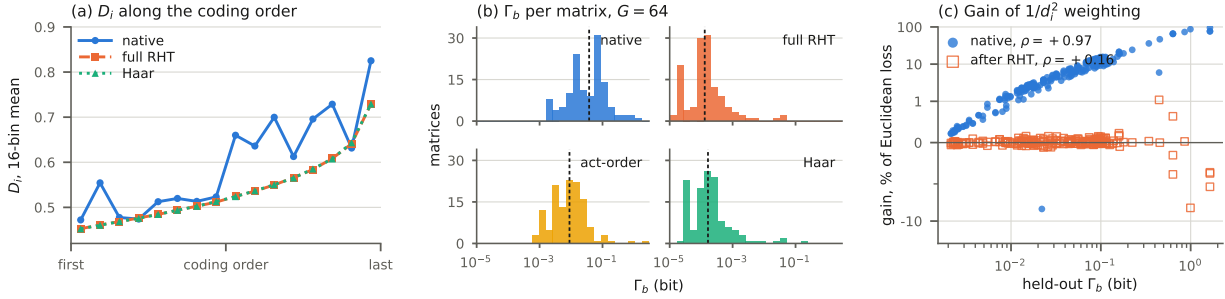
Figure 2: Within-block curvature anisotropy \Gamma_b (Eq. 3, G = 64 ), and what a rotation does to it; all panels Llama-2-7B. (a) The LDL diagonal along the coding order for one matrix (layer 15, q/k/v input, 16-bin means): native is jagged (whole-layer max / min 2503\times ), the full-dimension randomized Hadamard and the dense Haar rotation both produce the smooth ramp of Appendix B ( 2.7\times , 3.9\times ). (b) \Gamma_b over 128 public Llama-2-7B Hessians, one histogram per transform; medians (dashed) 0.038 native, 0.0089 act-order, 0.00013 full RHT, 0.00016 Haar. (c) Realized gain of 1/d_i^2 weighting on a held-out layer objective, as a fraction of the Euclidean loss ( 1 - L_W/L_E ), against \Gamma_b computed from the full held-out Hessian, 224 matrices: the gain follows \Gamma_b natively (Spearman +0.97 , filled) and not after the RHT ( +0.16 , hollow); the other two models in Figure 3. Symlog vertical axis; details in Appendix B.
