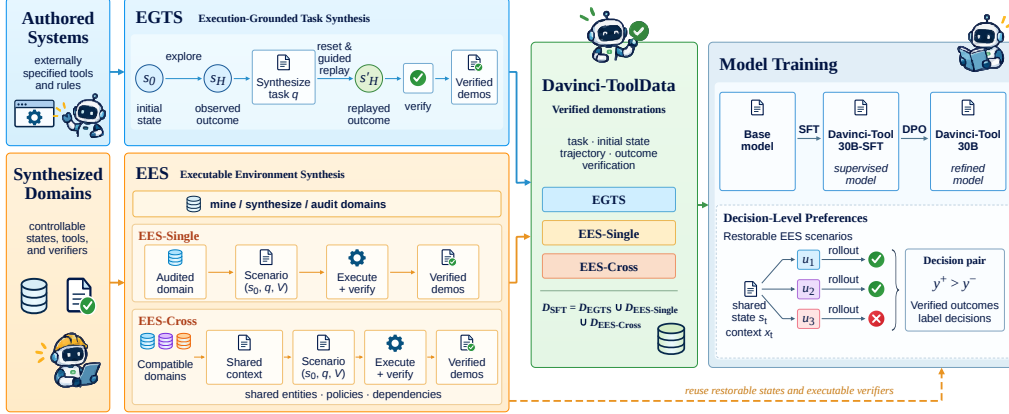
Figure 2: Construction of Davinci-ToolData and training of Davinci-Tool. EGTS converts explored outcomes in authored systems into verified task-conditioned replay demonstrations, while EES constructs audited executable environments for verified single-domain and cross-domain trajectories. The resulting demonstrations support SFT, and restorable EES states and verifiers are subsequently reused for decision-level DPO.
