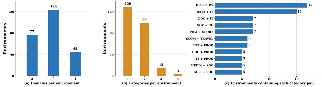
Figure 3: Structure of the 246 retained EES-Cross compositions. Panels (a), (b), and (c) show the number of constituent domains per environment, the number of application categories per environment, and category pairs appearing in at least 5 compositions, respectively. Pair counts may overlap when an environment spans more than two categories. Category codes are defined in Table 5.
