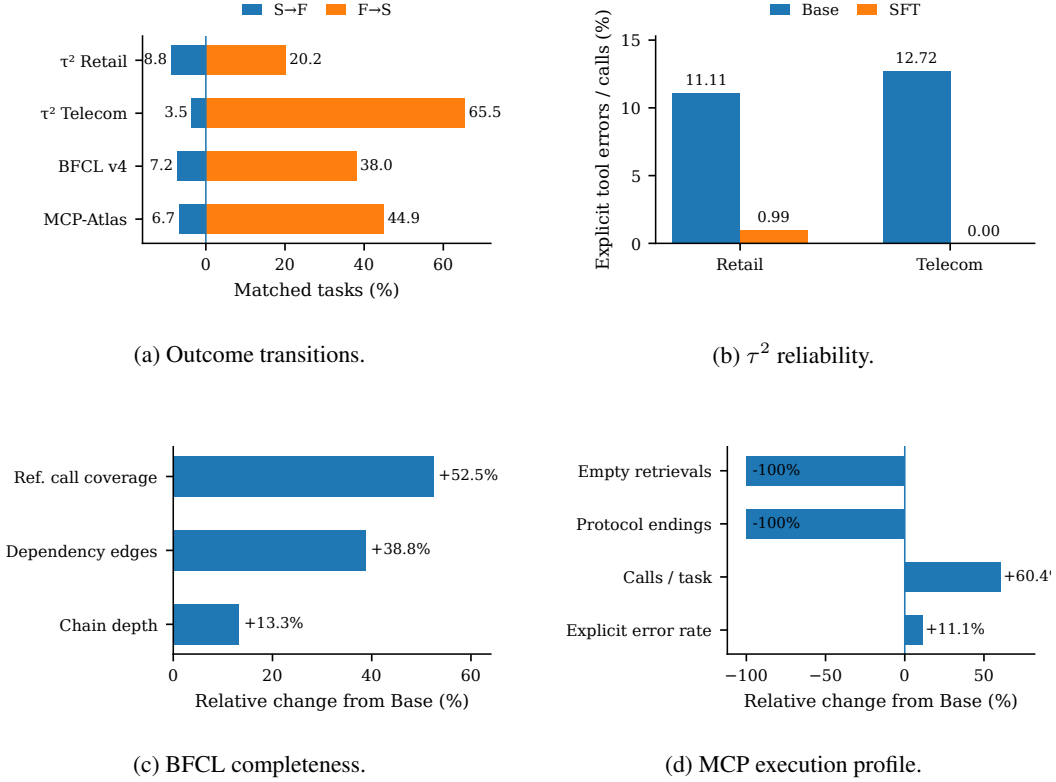
Figure 4: Paired execution changes associated with benchmark recovery after SFT. (a) shows the fractions of matched tasks changing from failure to success and from success to failure. (b) shows that, among recovered \tau^2 -bench tasks, explicit tool-error rates decrease from 11.11% to 0.99% on Retail and from 12.72% to 0 on Telecom. (c) shows that recovered BFCL v4 trajectories become more complete: normalized reference-call coverage increases from 56.41% to 86.01%, visible output-to-argument dependency edges from 1.21 to 1.68, and visible chain depth from 1.58 to 1.79. (d) shows a different pattern on MCP-Atlas: observed empty retrievals decrease from 37 to 0 and protocol-fragment endings from 7 to 0, while calls per task increase from 5.55 to 8.90 and the explicit tool-error rate changes from 14.41% to 16.01%. The paired analysis therefore indicates benchmark-specific execution changes rather than a single mechanism based on shorter trajectories or uniformly fewer tool errors.
