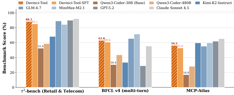
Figure 1: Performance on \tau^2 -bench, BFCL v4 multi-turn, and MCP-Atlas. Davinci-Tool-30B after DPO is shown with hatching, with its SFT checkpoint included for comparison. Detailed results and score provenance are reported in Table 2.
