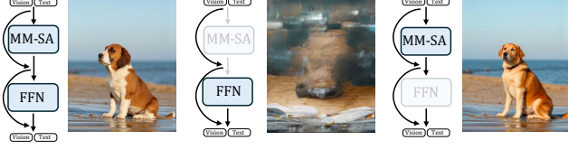
Figure 4. We study the role of the Multimodal Self-Attention (MM-SA) and Feed-Forward Network (FFN) components in MM-DiT blocks by bypassing one at the time. The results underscore that MM-SA predominantly determines spatial and temporal consistency, while FFN has a negligible impact.
