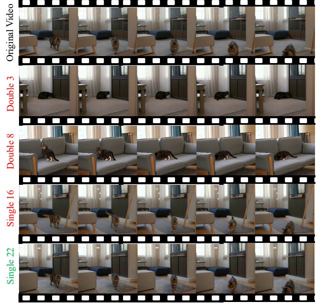
Figure 3. Removing individual blocks in the MM-DiT architecture affects different aspects of the generated video.
