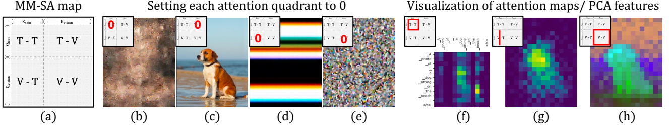
Figure 5. Pilot experiments. (left) MM-SA attention map. (middle) prompting the influence of each attention quadrant by setting it to 0. (right) visualization of attention map of the 1 st and 3 rd quadrants and PCA feature of the 4 th quadrant.
