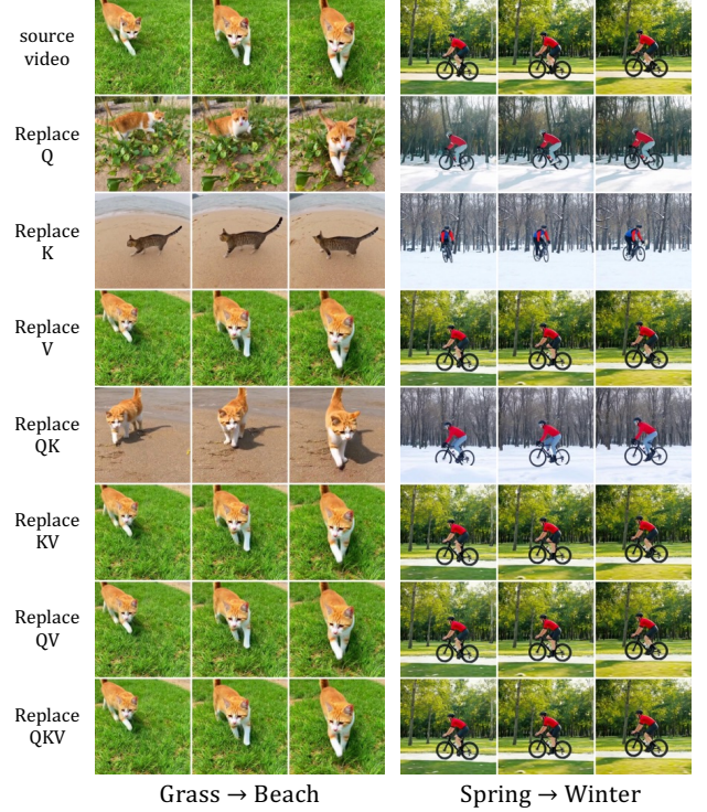
Figure 8. Manipulation of different QKV combinations. Replacing KV or V preserves original structure better, but sometimes fails to follow the target prompt; replacing Q or K , on the hand, adheres to the editing prompt but often fail to preserve source video structure; replacing QK achieves the best trade-off.
