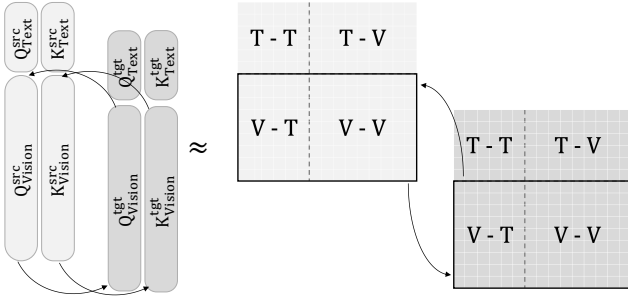
Figure 6. Query-key manipulation strategy. By substituting the vision components in Q and K, the approach effectively guides the editing process to balance prompt fidelity with preservation of the source structure.
