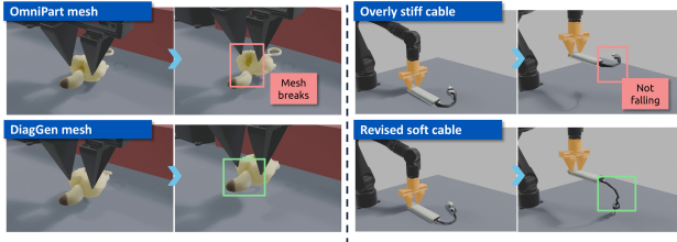
Fig. 5. Improved structure and material heterogeneity matter for manipulation. Left: Under the same grasp-and-lift action, the tetrahedralized OmniPart toy mesh separates because its disconnected parts lack an elastic load path, whereas the monolithized DiagGen mesh stays coherent. Right: One Airbot gripper grasps the USB hub case and lifts it from the support surface. The baseline and revised assets begin from similar poses. During the lift, the baseline cable retains an overly stiff bend, while the revised cable deforms naturally and lets the connector hang downward. Colored boxes mark the affected regions.
