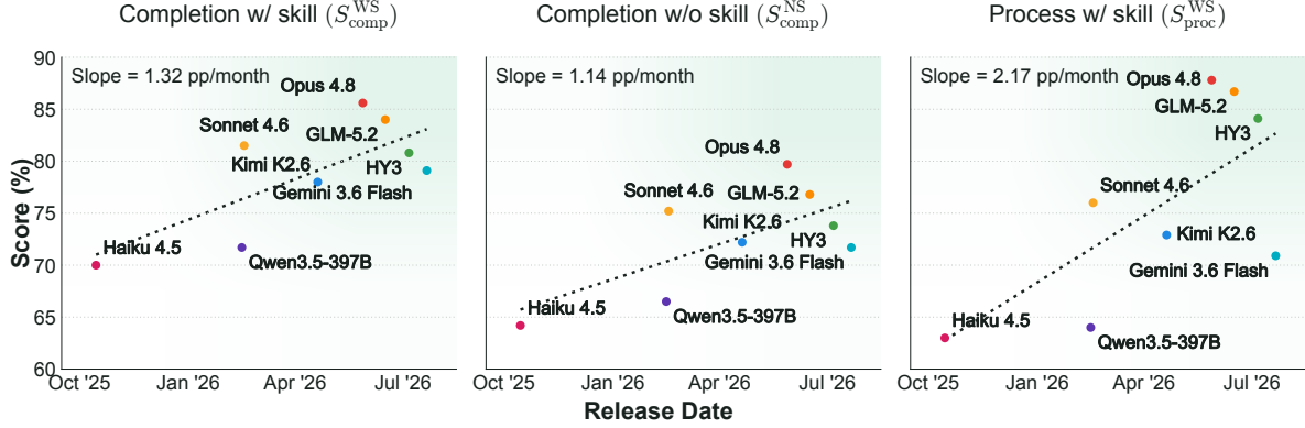
Figure 3 Model performance versus release date under loose scoring. Each panel plots S_{comp}^{WS} , S_{comp}^{NS} , and S_{proc}^{WS} against official release date, with dotted lines denoting linear least-squares fits. All three scores are positively associated with release date ( r > 0.68 ), with fitted slopes of 1.32, 1.14, and 2.17 pp/month, respectively. Corresponding strict scoring results are reported in Figure 7.
