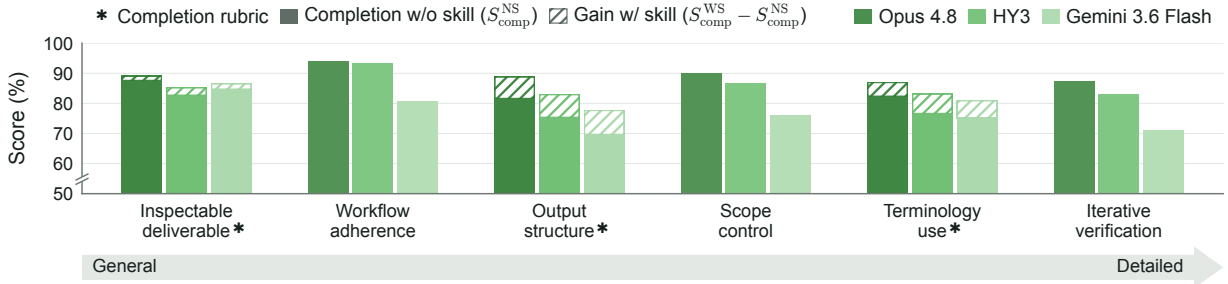
Figure 4 Loose rubric-category scores for models at different leaderboard positions. Opus 4.8, HY3, and Gemini 3.6 Flash are selected as representatives of different positions in the main leaderboard. For the Completion categories, WS and NS denote evaluation with and without the skill, respectively; the Process categories are evaluated only with the skill. The three models achieve relatively similar Inspectable Deliverable scores but separate more clearly in the remaining categories, particularly the three Process categories.
