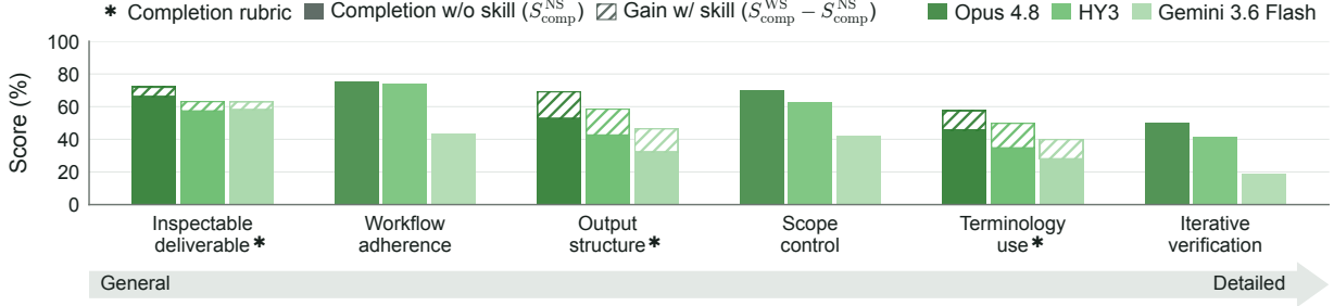
Figure 9 Strict rubric-category scores for models at different leaderboard positions. Opus 4.8, HY3, and Gemini 3.6 Flash are selected as representatives of different positions in the main leaderboard. For the Completion categories, WS and NS denote evaluation with and without the skill, respectively; the Process categories are evaluated only with the skill. Under strict scoring, credit is awarded only when all applicable requirements within a category are fully satisfied. Gemini 3.6 Flash remains comparable to HY3 in Inspectable Deliverable but trails both HY3 and Opus 4.8 in Output Structure, Terminology Use, and all three Process categories. Full numerical results are reported in Table 6.
