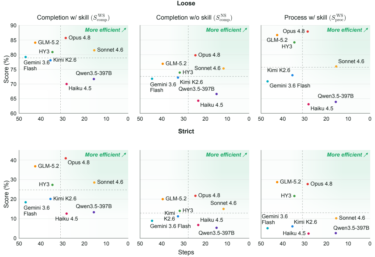
Figure 6 Model performance versus trajectory length. Each panel plots model performance against mean trajectory length, measured in interaction steps. Rows correspond to loose and strict scoring, while columns report completion w/ skill ( S_{comp}^{WS} ), completion w/o skill ( S_{comp}^{NS} ), and process with the skill ( S_{proc}^{WS} ). The horizontal axis is reversed, such that shorter trajectories appear farther to the right. Dashed lines indicate the cross-model mean score and mean trajectory length; consequently, the shaded upper-right region identifies models that achieve above-average performance with fewer-than-average steps. Across metrics and scoring schemes, longer trajectories do not consistently correspond to higher performance.
