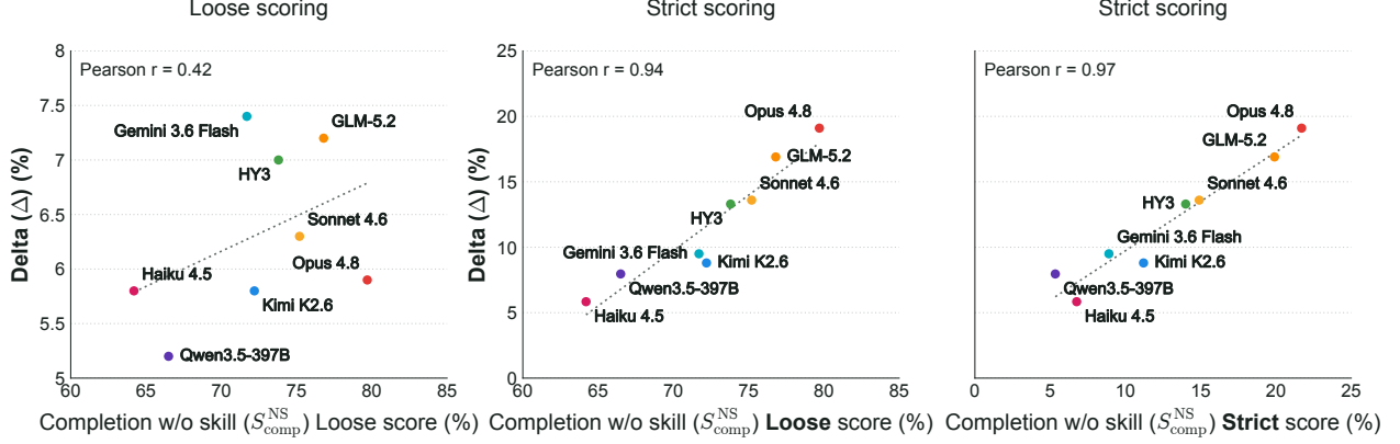
Figure 5 Gains from skill access versus baseline completion performance. We define the skill gain, \Delta , as the difference between the completion scores obtained with and without skill access: \Delta = S_{\text{comp}}^{\text{WS}} - S_{\text{comp}}^{\text{NS}} , where WS and NS denote the with-skill and without-skill conditions, respectively. The scatter plots relate the loose-score gain to the loose S_{\text{comp}}^{\text{NS}} baseline and the strict-score gain to both loose and strict S_{\text{comp}}^{\text{NS}} baselines. Each point represents one model, dotted lines show least-squares fits, and annotations report Pearson’s r . Loose-score gains are comparatively uniform (5.2%–7.4%; r = 0.42 ), whereas strict-score gains increase strongly with baseline performance ( r = 0.94 and r = 0.97 ).
