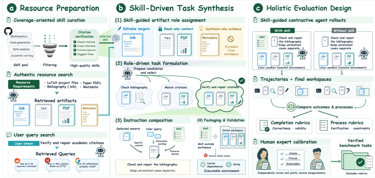
Figure 1 Overview of the SKILLFORGEBENCH construction pipeline, demonstrated using a citation verification skill as a running example: (a) Skills guide retrieval of real artifacts and user queries; (b) These inputs support task formulation, instruction composition, and environment packaging; and (c) Contrastive rollouts with and without skill access inform completion and process rubrics, followed by human task validation.
