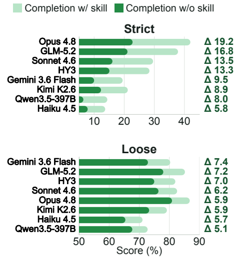
Figure 2 Completion gains from skill. Bars compare Completion scores with and without skill under strict and loose scoring. \Delta = S_{\text{comp}}^{\text{WS}} - S_{\text{comp}}^{\text{NS}} , shown to the right of each bar, denotes the Completion-score gain from skill access.
