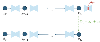
Figure 4: The h-space Spectral Mutation Operator. Initial noise \mathbf{x}_T is propagated to a timestep t_* where singular vectors \mathbf{v} of the Jacobian mapping the latent \mathbf{x}_t to the model’s internal activations h are computed. The latent is perturbed along this direction ( \tilde{\mathbf{x}}_t = \mathbf{x}_t + \alpha \mathbf{v} ) and the result \tilde{\mathbf{x}}_t is deterministically inverted to the timestep to form the offspring genotype \tilde{\mathbf{x}}_T .
