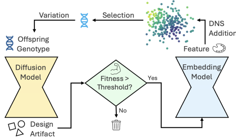
Figure 3: Quality-Diversity Diffusion Framework.
