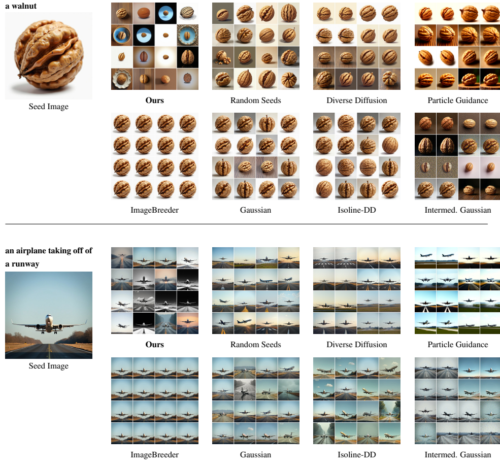
Figure 12: Flux top-16 images with highest fitness for sample prompts for Variation Operator Experiments.
