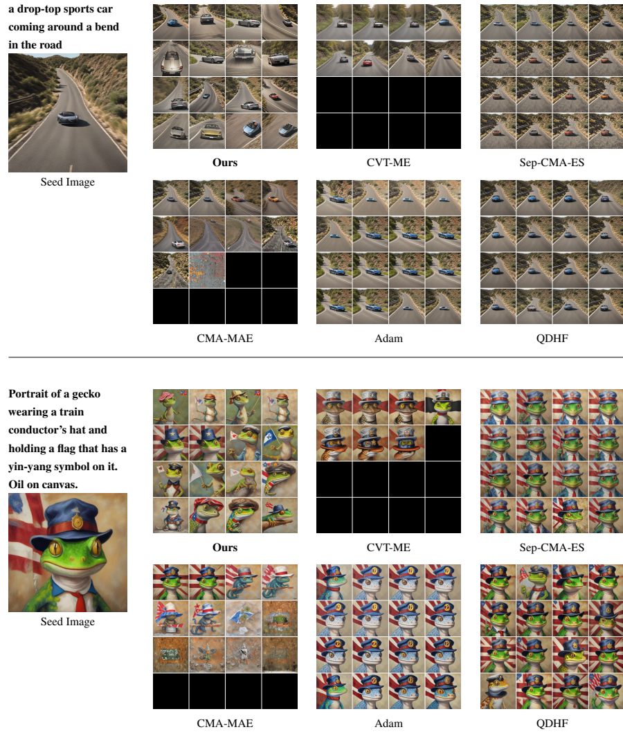
Figure 9: SDXL-Turbo Top-16 images with highest fitness for sample prompts.
