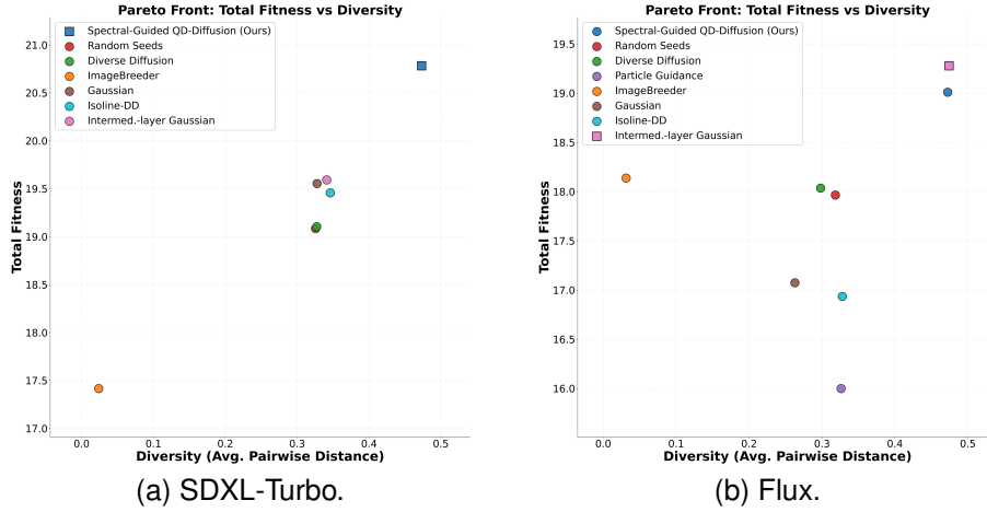
Figure 6: Quality vs Diversity.
