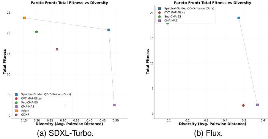
Figure 5: Quality vs Diversity.
