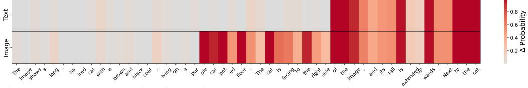
Figure 2: Average token-wise distribution change on textual and visual perturbation. Visual perturbation has a greater effect than textual perturbation on the output probability.
