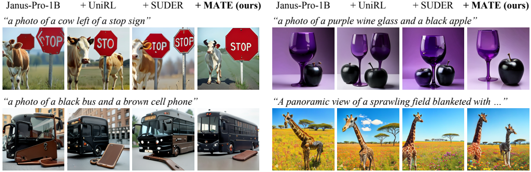
Figure 3: Generation samples. Images for the same prompt from Janus-Pro-1B and the three self-training methods applied to it; three prompts are from GenEval and one from DPG-Bench. One selected sample per model and prompt is shown from four generated samples, using the same sampling settings. The DPG-Bench prompt asks for a giraffe and a zebra standing side by side in a field of wildflowers; its displayed text is shortened.
