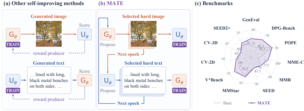
Figure 1: Self-improvement through mutual challenges. (a) In other self-improving methods such as SUDER (Hong et al., 2025), one branch scores an output to reward its producer. (b) Our MATE selects valid outputs that challenge the opposite branch, trains that solver, and uses the selected outputs to construct new challenges in the next epoch. In both panels, G_\theta and U_\theta share one backbone and the examples are real training records. (c) MATE and Janus-Pro-1B on the 11 benchmarks of the main tables. Each axis uses its own truncated linear range, shared by both methods, so polygon areas do not measure overall performance. MME-C is in cognition points, and other scores are percentages.
