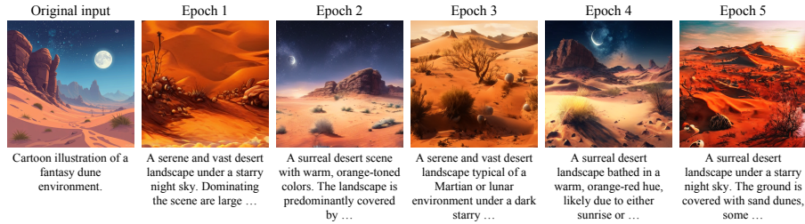
Figure 5: An evolving training input under MATE. An original dataset pair (left) is followed through five epochs. Selected images and descriptions become inputs for the next epoch. The image and text in each column come from separate training directions and need not form a matched pair. Descriptions are shortened for display. Figure 7 in Appendix C shows a second example.
