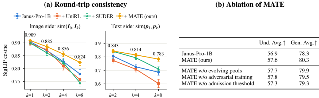
Figure 6: Round-trip consistency and ablation. (a) Left: SigLIP cosine between the original image I_0 and the image I_k after k rounds. Right: SigLIP text cosine between the first description p_1 and the k -th description p_k . Points are means over 32 held-out samples and whiskers are standard errors. (b) Understanding and generation averages of Janus-Pro-1B, MATE, and three variants of MATE.
