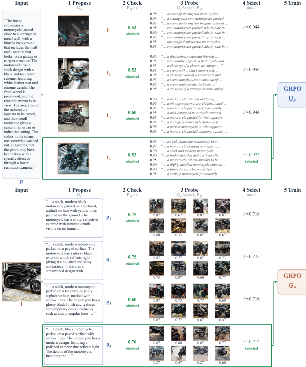
Figure 8: One complete round of MATE, in the format of Figure 2(a). All candidates, attempts, and scores of one training pair in one epoch (pair 4, epoch 2 of the main run). Upper row: from the source description p , the generation branch proposes N = 4 images I_1, \dots, I_4 ; each is checked against p ( R_G , admission threshold \tau = 0.5 ); the understanding branch writes M = 8 descriptions of each admitted image, scored by U_\theta (the eight scores and one example are shown); the image with the lowest mean score \bar{r} is selected and its eight attempts train U_\theta with GRPO. Lower row: from the source image I , the understanding branch proposes N = 4 descriptions p_1, \dots, p_4 , checked against I ( R_U ); the generation branch produces M = 8 images from each admitted description, scored by R_G ; the description with the lowest \bar{r} is selected and its attempts train G_\theta . The two selected outputs become this pair's inputs in the next epoch. Descriptions are shortened for display.
