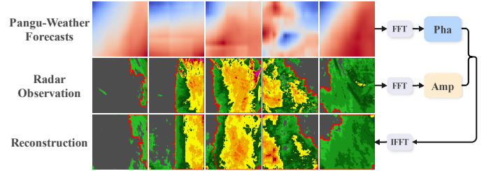
Fig. 2 Overall architecture of our proposed PW-FouCast.
