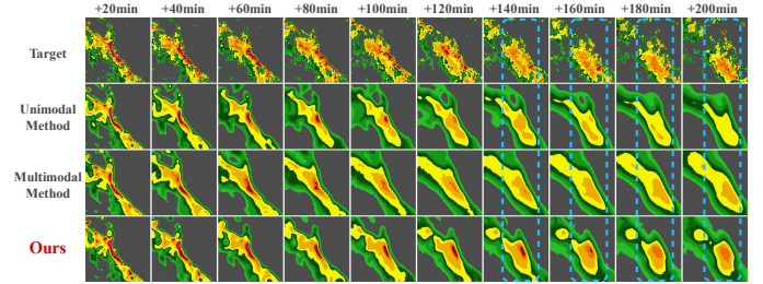
Fig. 1 Qualitative comparison of predicted radar reflectivity across unimodal and multimodal methods.
