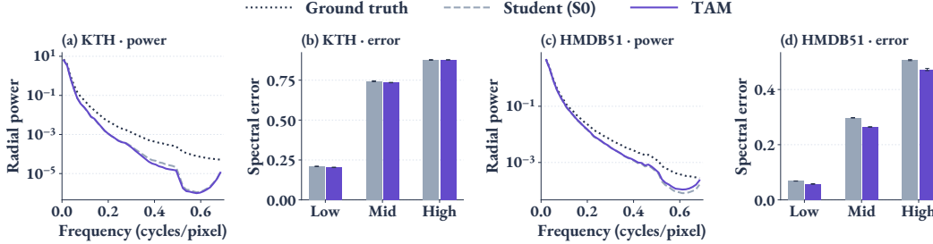
Figure 4: Spatial frequency analysis on KTH and HMDB51. Lower normalized spectral error is better; bars and error bars show means and standard deviations over four training runs.
