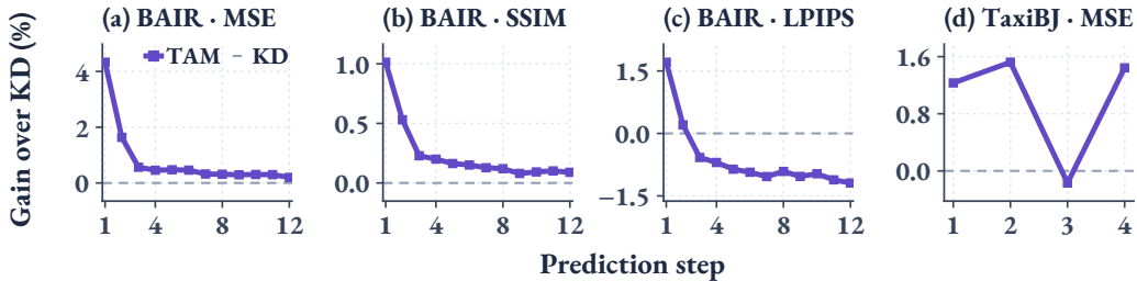
Figure 3: Prediction-horizon gains over matched KD baselines, averaged over four paired runs. Positive values indicate lower MSE/LPIPS or higher SSIM; the dashed line denotes the KD baseline.
