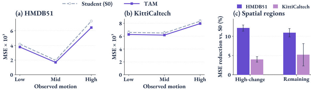
Figure 5: Prediction errors across observed-motion groups (left, middle) and relative MSE reductions in input-defined spatial regions (right). Error bars show standard deviations over four paired runs.
