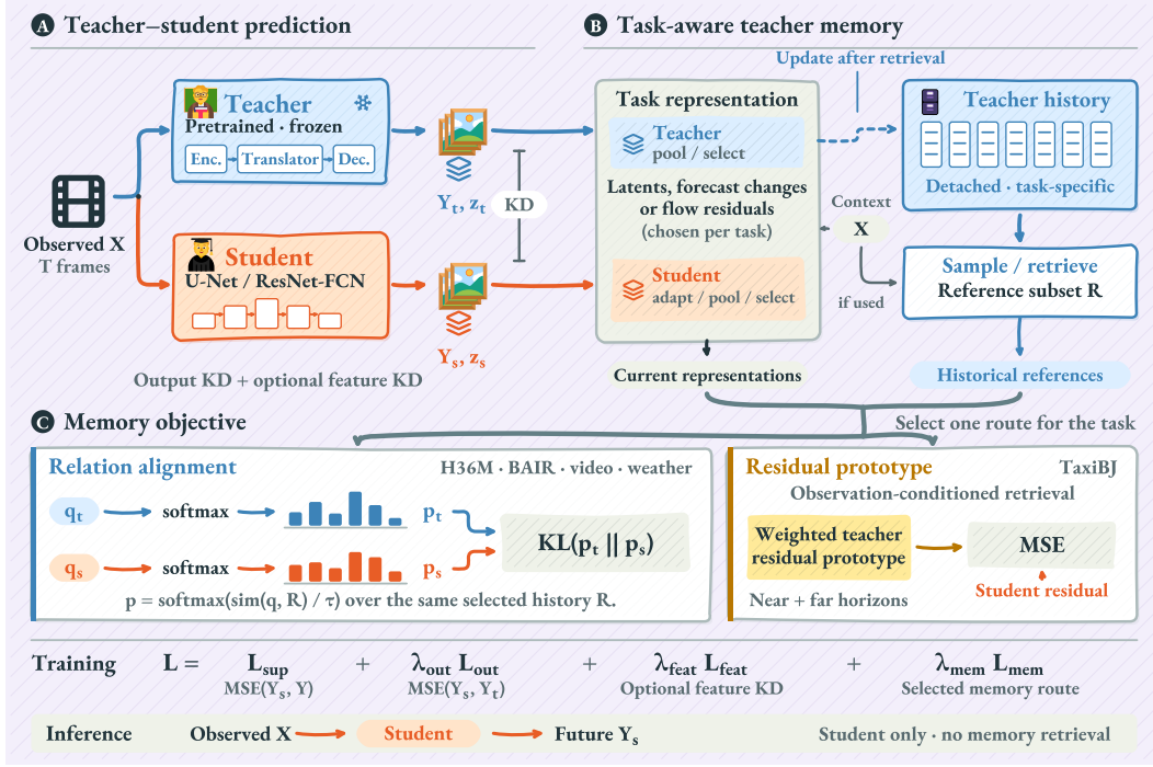
Figure 2: Overview of TAM. (A) A frozen teacher provides output and optional feature supervision. (B) Task-specific representations enter history after reference selection. (C) Memory supervision matches relations over shared references or regresses retrieved residual prototypes. Inference uses only the student. Glyphs and distribution bars are schematic.
