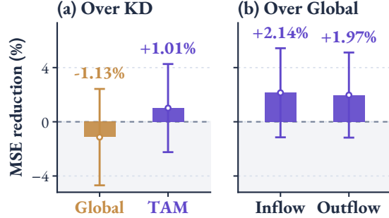
Figure 1: TaxiBJ memory comparison. (a) Overall MSE reduction over KD. (b) TAM’s inflow/outflow gains over Global Memory. Bars: four-run paired means; whiskers: population SD. Positive values indicate improvement.
