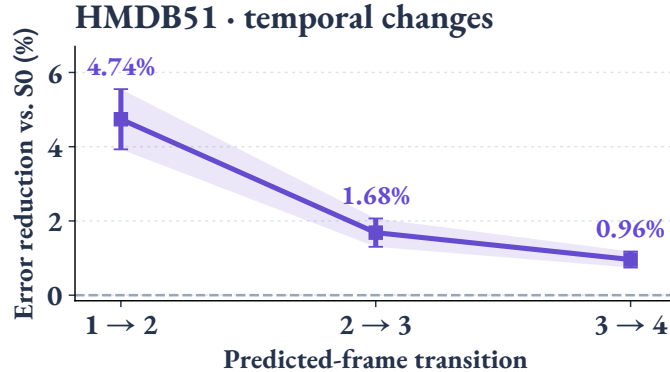
Figure 6: HMDB51 frame-difference MSE reduction relative to S0. Points and error bars show the mean and standard deviation over four paired runs.
