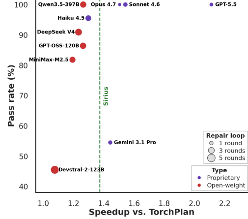
Figure 1: DataKernelBench tests LLMs on GPU kernel generation for database query optimization, where multiple models achieve 100% pass rate and substantial speedups over the TorchPlan baseline on TPC-H SF10 with NVIDIA H100. See Table 1 and Section 4.2.
