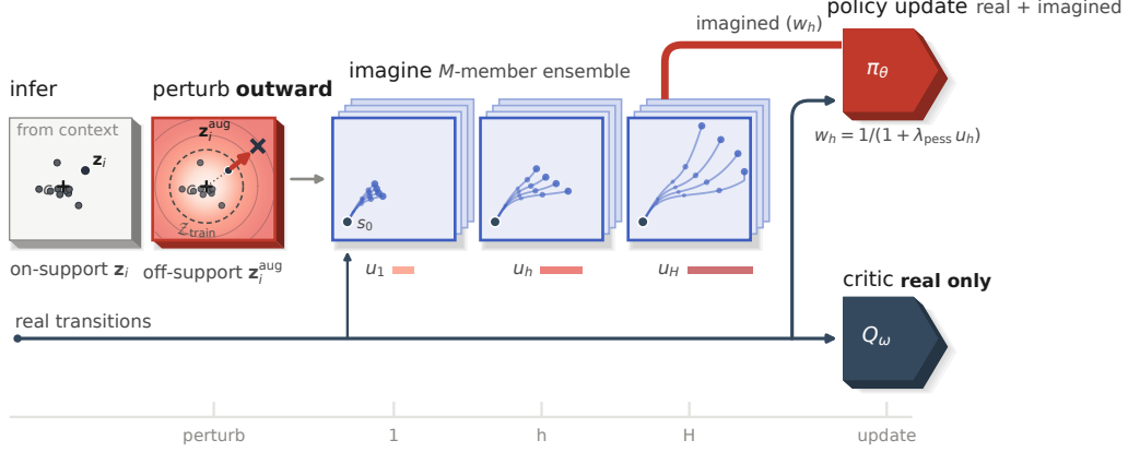
Figure 2: Conceptual overview of PLATO. From left to right: a latent \mathbf{z}_i is inferred from the context of a training task; it is pushed outward from the training centroid c to \mathbf{z}_i^{\text{aug}} , off the training support \mathcal{Z}_{\text{train}} (Assumption 1, Proposition 1); and the M -member decoder ensemble, conditioned on \mathbf{z}_i^{\text{aug}} , rolls out a short imagined trajectory from a real state s_0 , recording the per-step disagreement u_h as its members drift apart. The policy \pi_\theta is updated on real transitions and on the imagined ones, each imagined step weighted by w_h = 1/(1 + \lambda_{\text{pess}} u_h) , while the critic Q_\omega is trained on real transitions only (Theorem 2).
