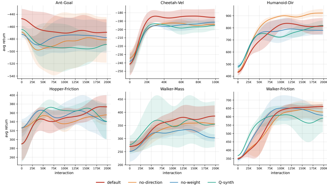
Figure 4: Component ablations of PLATO on out-of-support returns. Learning curves on six MuJoCo environments. default is the full algorithm; no-direction replaces the centroid-outward direction \hat{n}_i with a random unit vector; no-weight sets \lambda_{\text{pess}} = 0 ; Q-synth also trains the critic on imagined Bellman targets (the variant analyzed by Theorem 2). Curves show mean over 5 seeds; shaded regions indicate one standard deviation.
