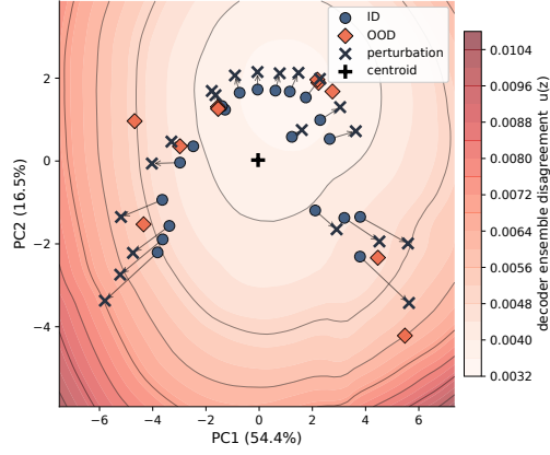
Figure 1: Latent geometry on Ant-Goal. Background: decoder-ensemble disagreement u(\mathbf{z}) over the latent space projected by principal component analysis (PCA). In-distribution (ID) tasks (blue) populate the low- u region around the centroid c (+). Out-of-support tasks (orange, labeled OOD) exhibit substantially higher disagreement on average, and our perturbations \mathbf{z} \rightarrow \mathbf{z}^{\text{aug}} (arrows, \times ) reach the same high- u outward region, consistent with Assumption 1, Proposition 1, and Theorem 1.
