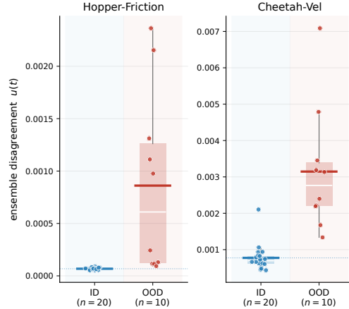
Figure 3: Off-support disagreement stays large. Per-task ensemble disagreement at the trained PLATO checkpoint. ID values (blue) are near zero, whereas out-of-support values (red, labeled OOD) are several-fold to an order of magnitude larger, consistent with Theorem 1.
