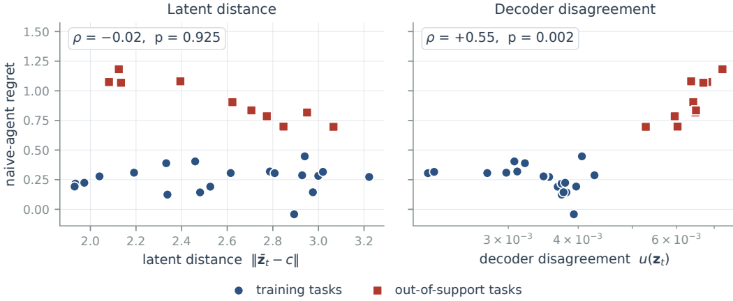
Figure 5: Ensemble disagreement tracks task difficulty; latent distance does not. Each point is one Ant-Dir task (20 training and 10 out-of-support tasks). Vertical axis: normalized regret of a naively trained agent (CSRO), (R_{\text{expert}} - R_{\text{CSRO}})/|R_{\text{expert}}| . Left: distance of the task’s mean latent from the training centroid. Right: decoder-ensemble disagreement u at the task’s latent (log scale). \rho is the Spearman rank correlation over all 30 tasks.
