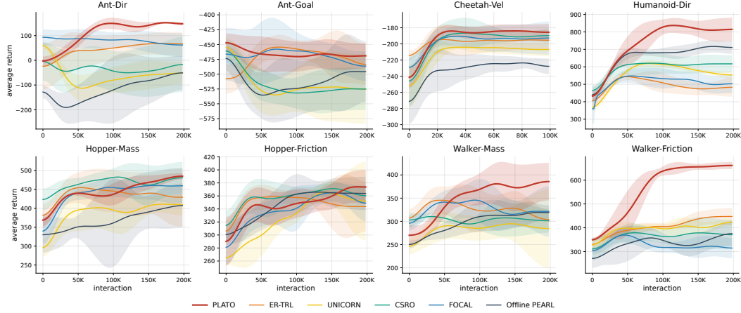
Figure 8: Learning curves on the eight MuJoCo OMRL benchmarks, out-of-support. Same format as Figure 7.
