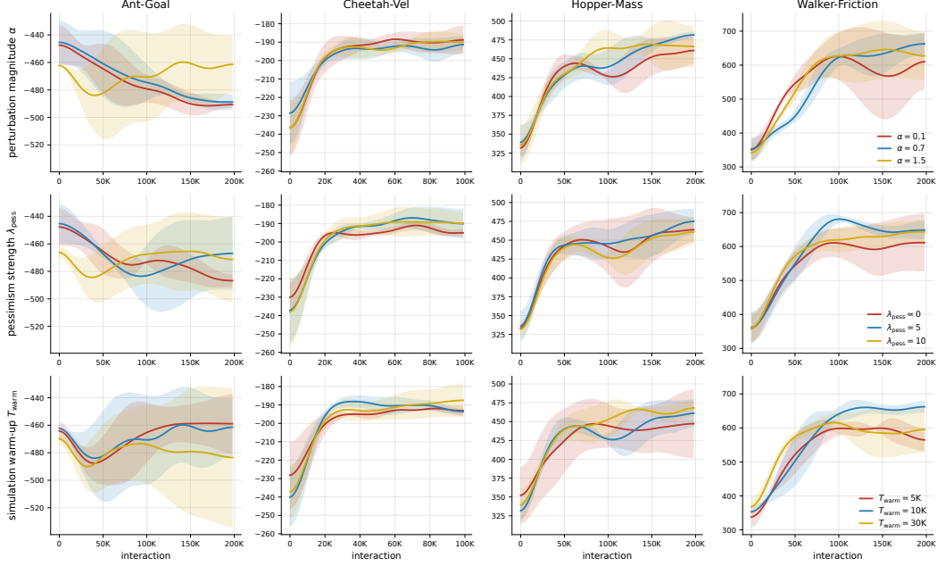
Figure 6: Out-of-support sensitivity analysis. Each row sweeps one hyperparameter, with the other two held at their middle swept value. Top: perturbation magnitude \alpha \in \{0.1, 0.7, 1.5\} . Middle: pessimism strength \lambda_{\text{pess}} \in \{0, 5, 10\} . Bottom: warm-up T_{\text{warm}} \in \{5\text{K}, 10\text{K}, 30\text{K}\} . Columns: Ant-Goal and Cheetah-Vel (reward-shift), Hopper-Mass and Walker-Friction (dynamics-shift). Curves show mean out-of-support return over 5 seeds.
