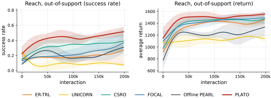
Figure 9: MetaWorld Reach, out-of-support tasks. Success rate (left) and average return (right) over training, averaged over 3 seeds; shaded regions indicate one standard deviation.
