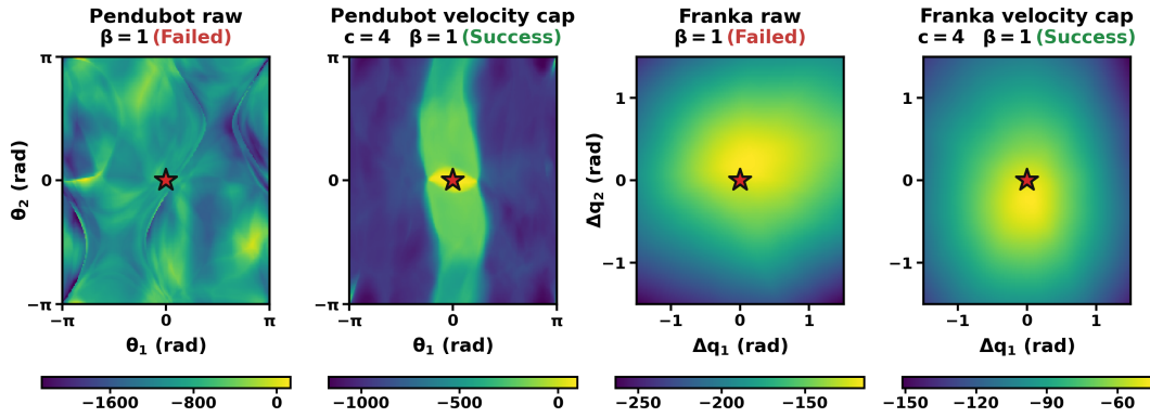
Figure 5: Velocity capping contracts critic scale and restores target-centered structure. From left to right: failed raw Pendubot, successful velocity-capped Pendubot, failed raw Franka, and successful velocity-capped Franka, all at \beta = 1 and with c = 4 in the capped conditions using seed 42. Pendubot fixes angular velocities at zero, while Franka holds all remaining joints at a common target-conditioned reference. Red stars mark the upright or zero-error target.
