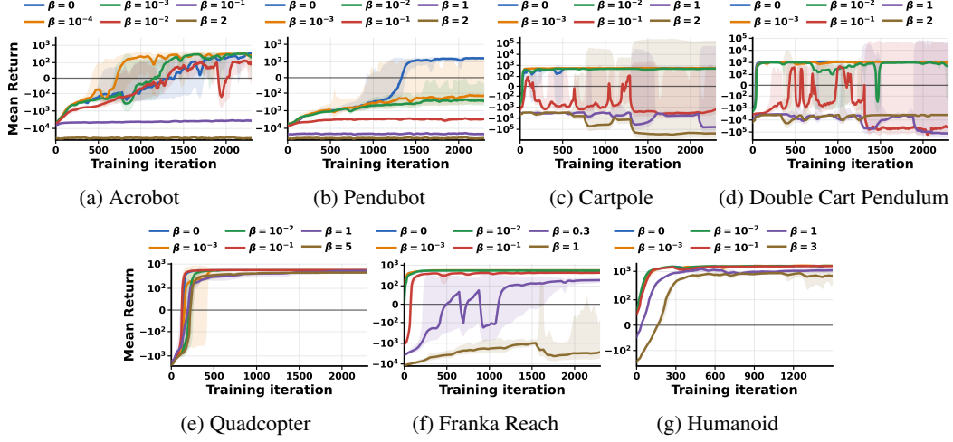
Figure 9: Training return (Equation (19)) across the seven Isaac Lab tasks. Each seed is first smoothed with a centered 51-iteration moving average; curves and shaded regions then show the across-seed mean and one standard deviation, respectively.
