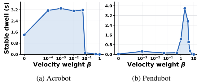
Figure 1: A velocity penalty has task-dependent effects in direct trajectory optimization , shown by the mean stable dwell for IPOPT-optimized Acrobot and Pendubot trajectories. Moderate velocity regularization helps in different ranges for the two plants, while an overly large weight suppresses successful motion in both.
