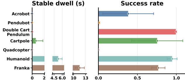
Figure 3: No-velocity-observation ablation at \beta = 0 . Each task keeps exactly the same zeroth-order reward and velocity-aware success predicate used in the full-observation experiment. Bars show the five-seed mean and population standard deviation of best dwell (left) and corresponding success rate (right).
