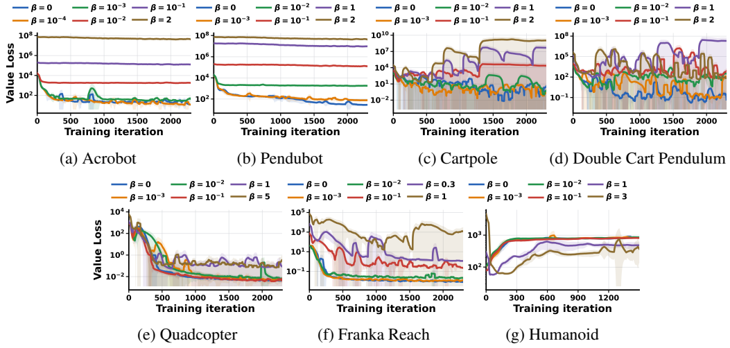
Figure 10: Training value loss (Equation (20)) across the seven Isaac Lab tasks. Each seed is first smoothed with a centered 51-iteration moving average; curves and shaded regions then show the across-seed mean and one standard deviation, respectively.
