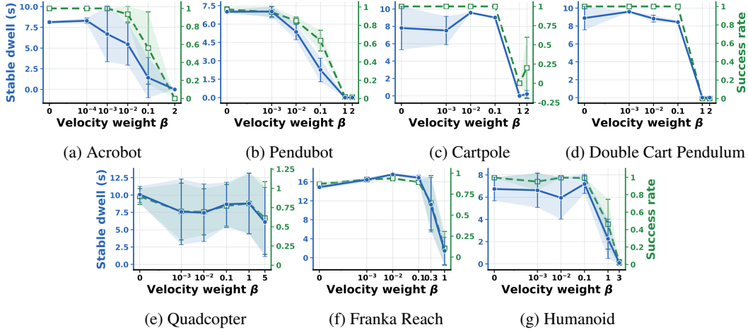
Figure 2: Velocity-reward sweeps with full configuration and velocity observations. Blue solid curves show stable dwell and green dashed curves show success rate; bands are mean \pm one population standard deviation over five seeds. Every task learns reaching, braking, and sustained stabilization at \beta = 0 , while sufficiently large velocity penalties generally reduce both metrics.
