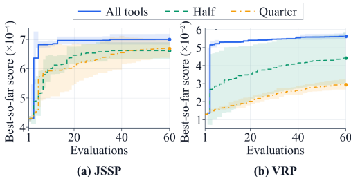
Figure 4: Effect of tool-library size on best-so-far performance over 60 evaluations for JSSP and VRP. The curves show the mean scores over seeds 1–3, and the shaded regions indicate one standard deviation around the mean. All Tools uses the full library, while Half Tools and Quarter Tools retain one-half and one-quarter of the tools, respectively.
