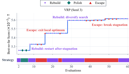
Figure 2: Traceability of TASA over 60 evaluations on a representative run of VRP (Seed 3). The curve shows the best-so-far scores, while the markers and colored timelines indicate the optimization strategies selected throughout the search.
