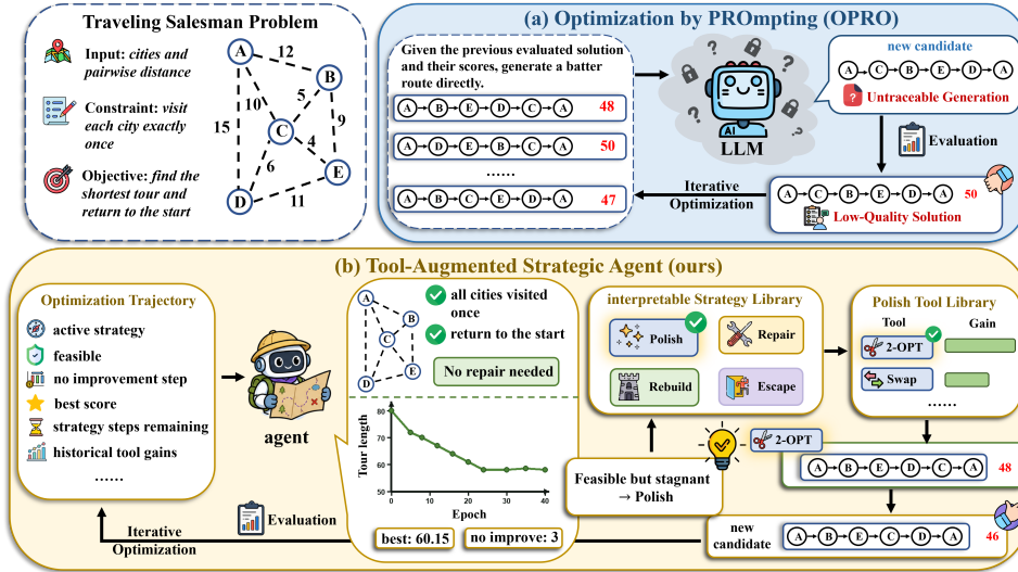
Figure 1: Motivation and overview of our Tool-Augmented Strategic Agent. TASA shifts the role of the LLM from directly generating solutions to planning optimization strategies from optimization trajectories, and executes these strategies through strategy-guided adaptive tool planner.
