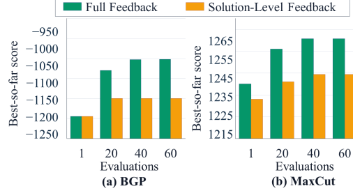
Figure 5: Effect of feedback granularity on best-so-far performance for BGP and MaxCut. The bars report the mean best-so-far scores over seeds 1–3 at evaluations 1, 20, 40, and 60. Full Feedback provides the strategy planner with the recorded optimization trajectory, whereas Solution-Level Feedback retains only solution-level information.
