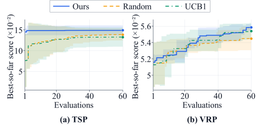
Figure 3: Effect of the tool-planning mechanism on best-so-far performance over 60 evaluations for TSP and VRP. The curves show the mean best-so-far scores over seeds 1-3, and the shaded regions indicate one standard deviation around the mean. Ours denotes the strategy-guided adaptive tool planner, while Random and UCB1 are alternative tool-planning policies.
