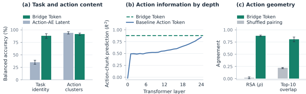
Figure 5: Bridge Tokens connect task semantics to action structure. (a) Linear-probe balanced accuracy for task identity and action clusters. (b) Action-chunk R^2 for baseline Action Tokens across layers (blue) and Bridge Tokens before the Action Expert (dashed). (c) RSA and top-10 neighbor overlap with ground-truth actions. Error bars show fold standard deviations in (a,b), and task standard deviations for Bridge Tokens or 5th–95th permutation percentiles for shuffled controls in (c).
