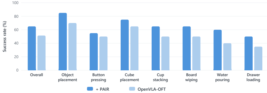
Figure 4: Real-world success rates over 20 trials per task. PAIR improves OpenVLA-OFT across all seven tasks, with an overall gain of 13.6 percentage points.
