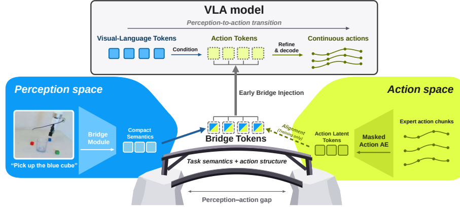
Figure 1: Conceptual view of the perception-to-action transition. Standard VLAs require Action Tokens to acquire and organize action-relevant information during decoding. PAIR instead learns perception-derived Bridge Tokens shaped by the structure of expert actions and injects them into the initial Action Tokens, so that the Action Expert begins from an action-ready intermediate state and refines it toward continuous control. The Action Autoencoder is used only during training.
