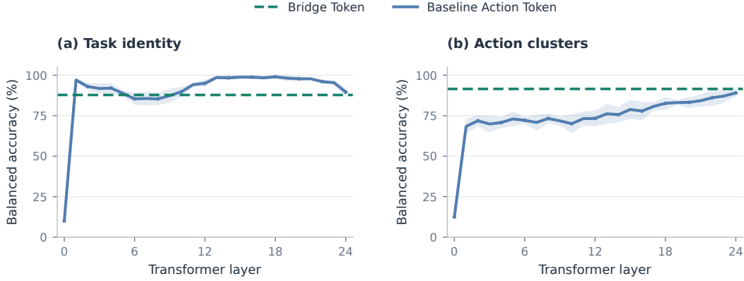
Figure 6: Task identity and action-cluster decodability across depth. Blue curves show baseline Action Tokens with fold-standard-deviation bands. Green dashed lines indicate the pre-LLM Bridge Token score. Layer 0 precedes the Transformer; layers 1–24 denote completed blocks.
