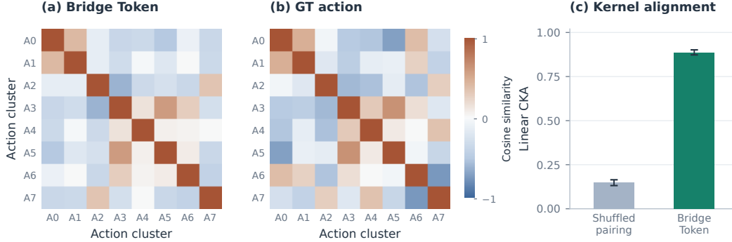
Figure 8: Action-cluster geometry and kernel alignment. (a,b) Cosine similarities between GT-derived action-cluster centroids in the two spaces, using a shared color scale. A0–A7 index unsupervised clusters rather than named behaviors. (c) Within-task linear CKA. Error bars indicate task standard deviation for Bridge Tokens and the 5th–95th percentile interval of the trajectory-permutation reference.
