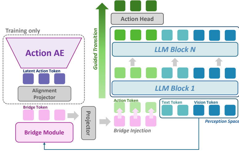
Figure 2: Overview of PAIR. The Masked Action Autoencoder encodes expert actions into Action Latent Tokens, which guide the perception-derived Bridge Tokens through representation alignment. The Bridge Tokens are projected into the Action Token space and injected at the entrance of the Action Expert.
